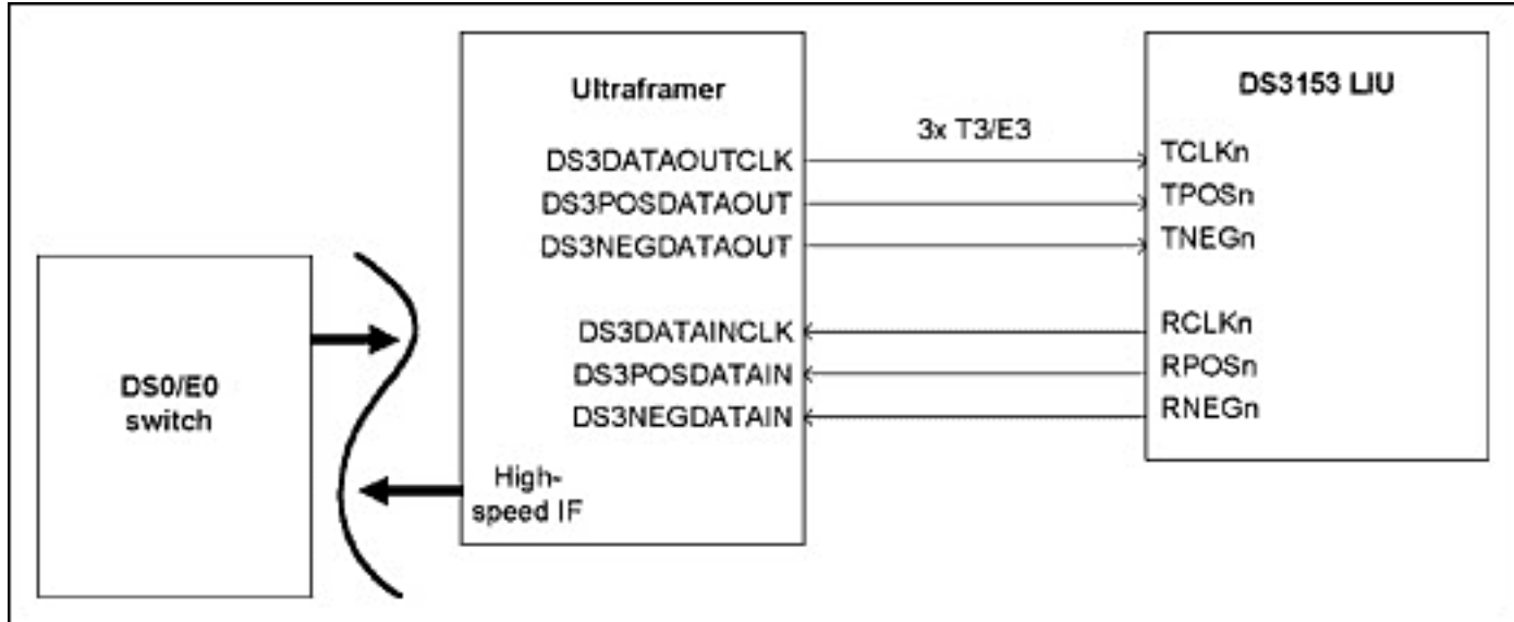
Figure 4. T3/E3 and DS0/E0 Map/Demap application.
