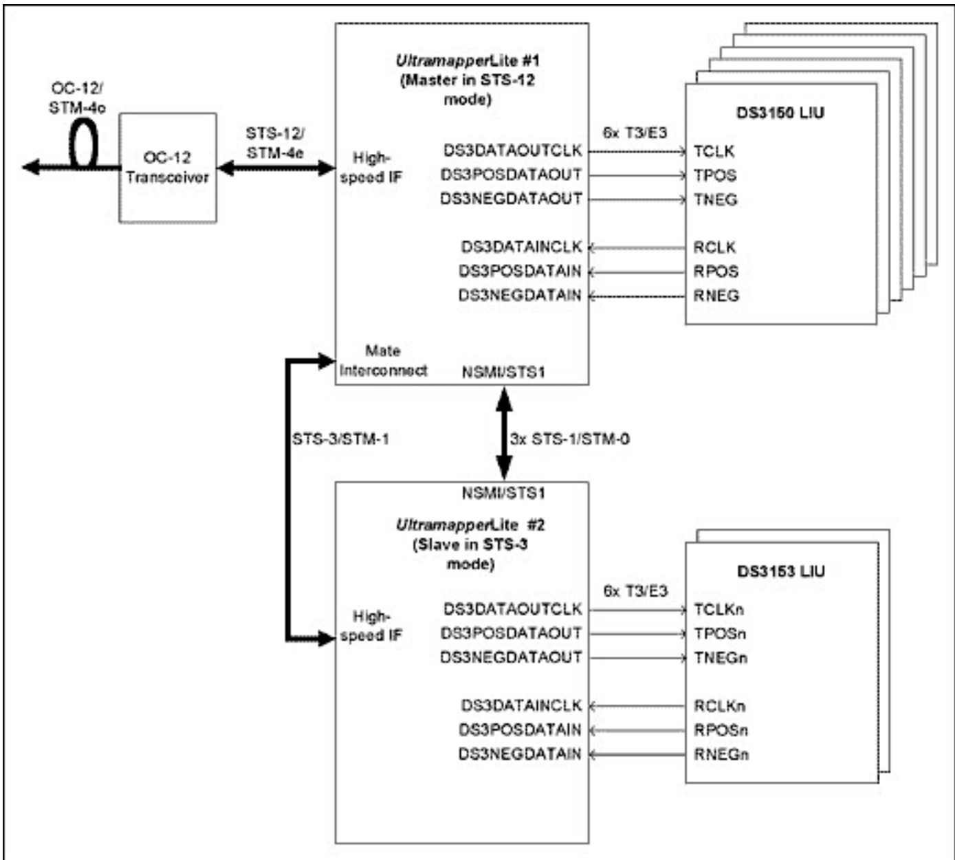
Figure 1. T3/E3 clear channel application.
