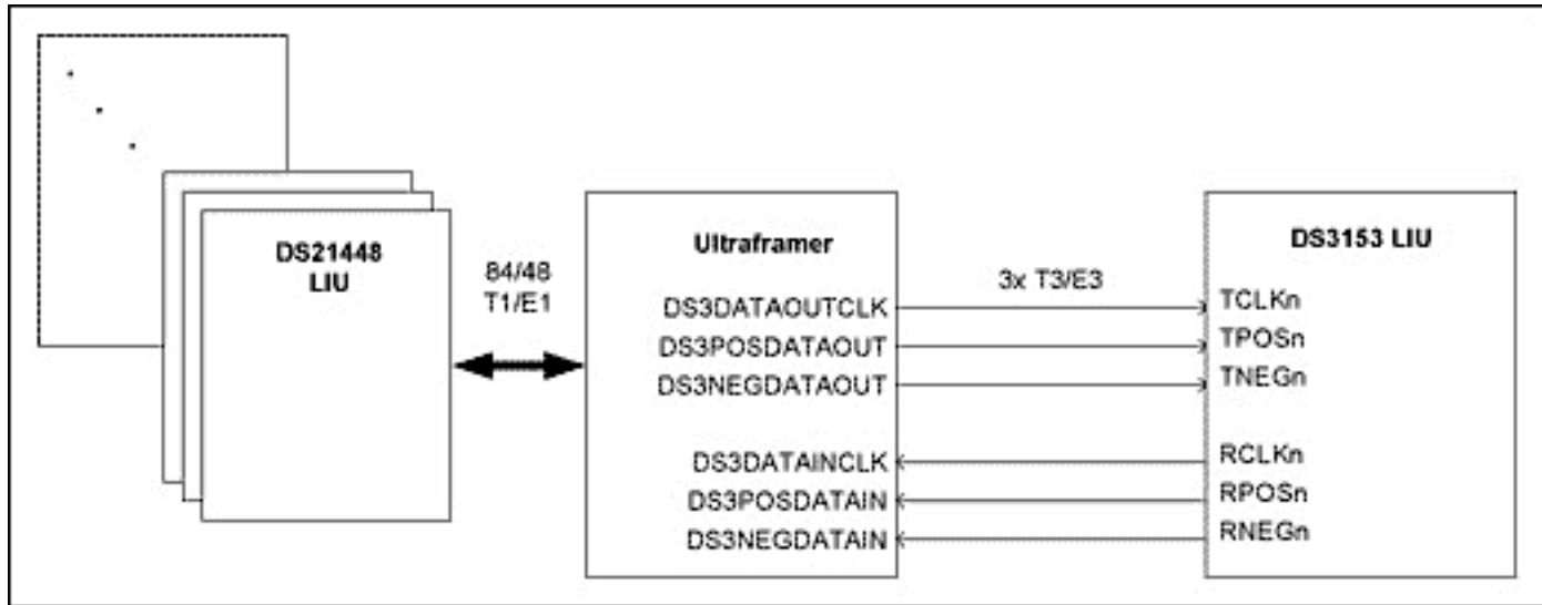
Figure 3. T3/E3 and T1/E1 Map/Demap application.
