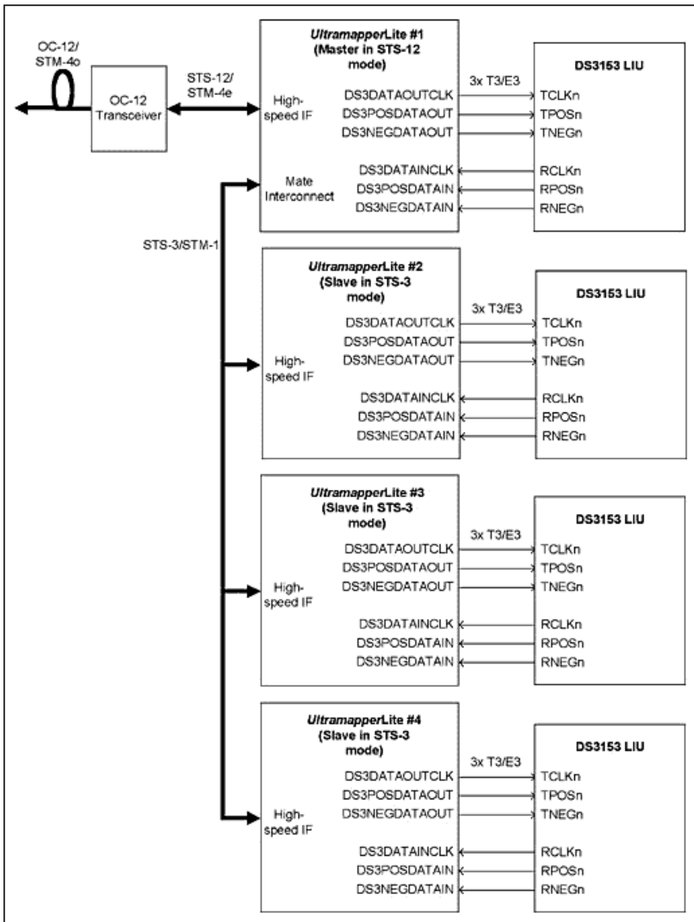
Figure 2. T3/E3 TransMUX application.
