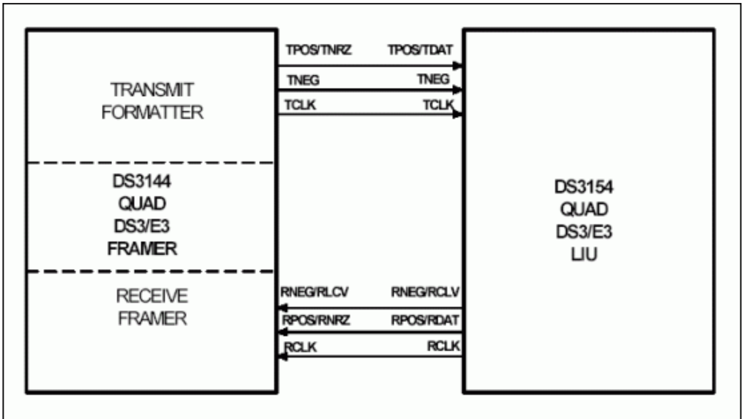
Figure 1. Functional diagram for the framer and LIU.
