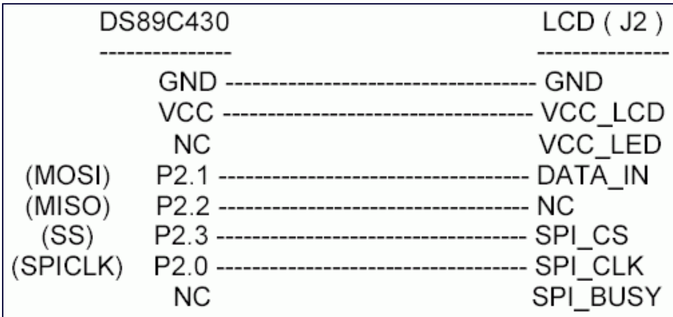
Figure 1. Connection diagram.
