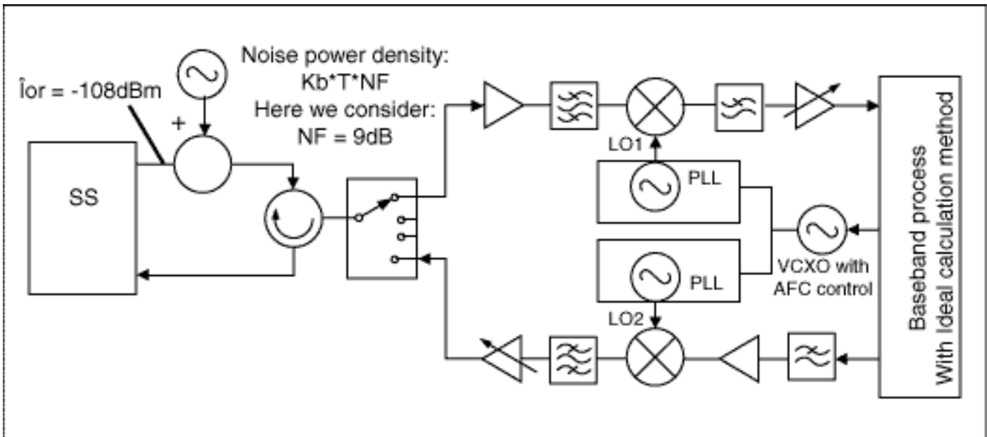
Figure 2. Analysis Model.
