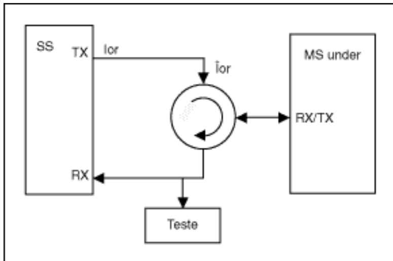
Figure 1. Test Configuration.
