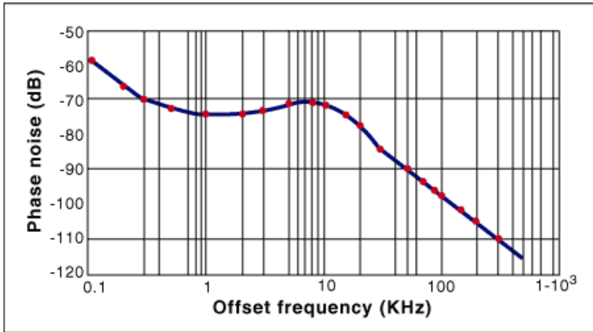
Figure 4. MAX2392 phase noise.
