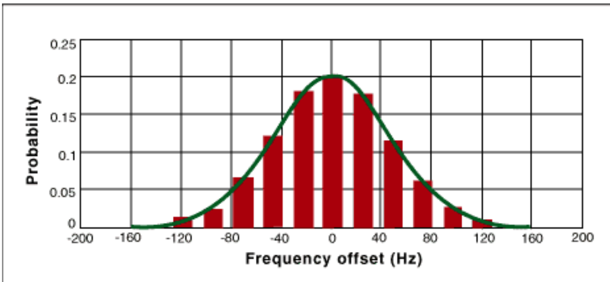
Figure 3. The probability distribution of frequency estimate error.
