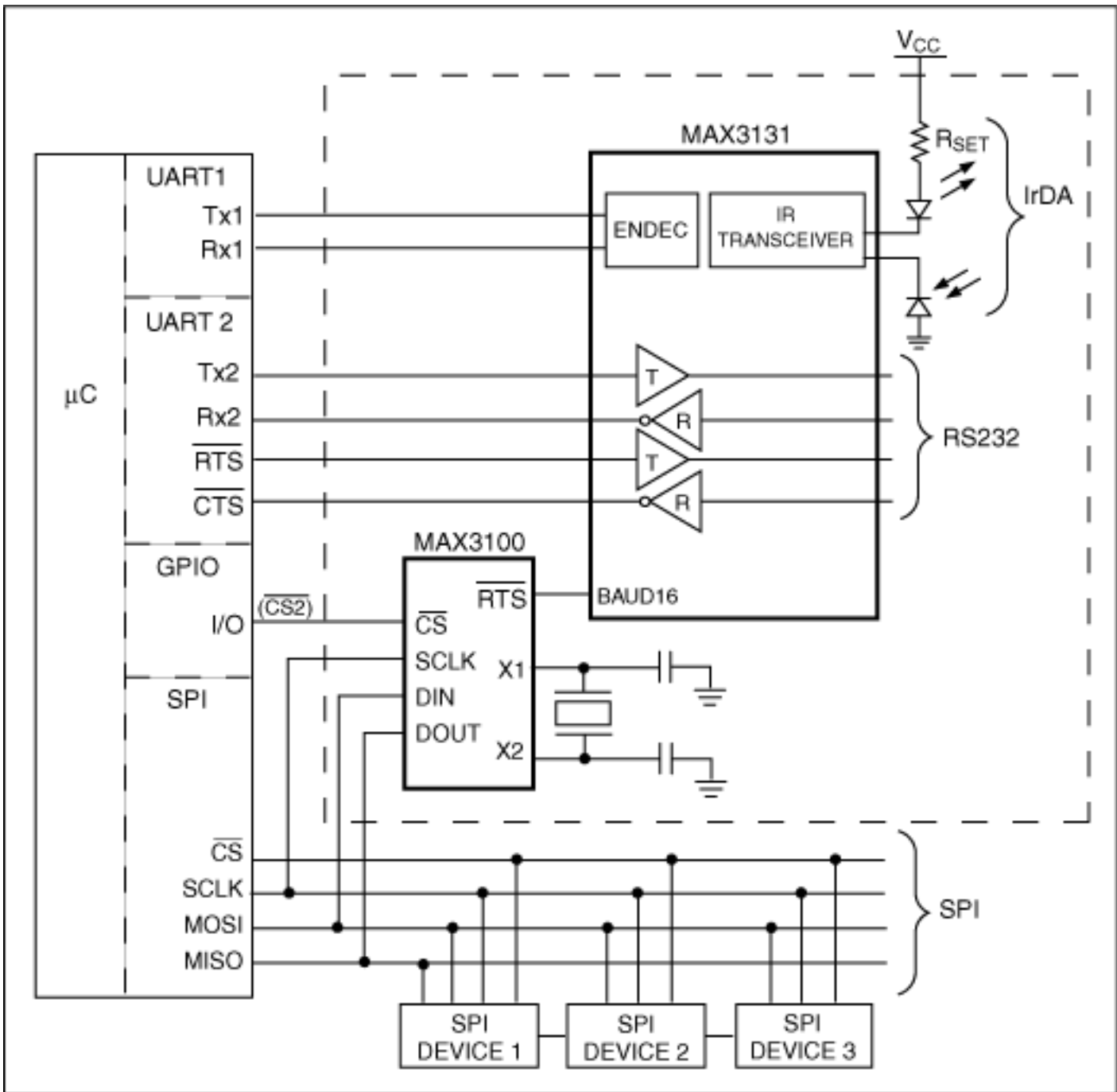
Figure 7. This MAX3100 circuit requires only one additional µC I/O to implement a software-adjustable BAUD16 clock generator.
