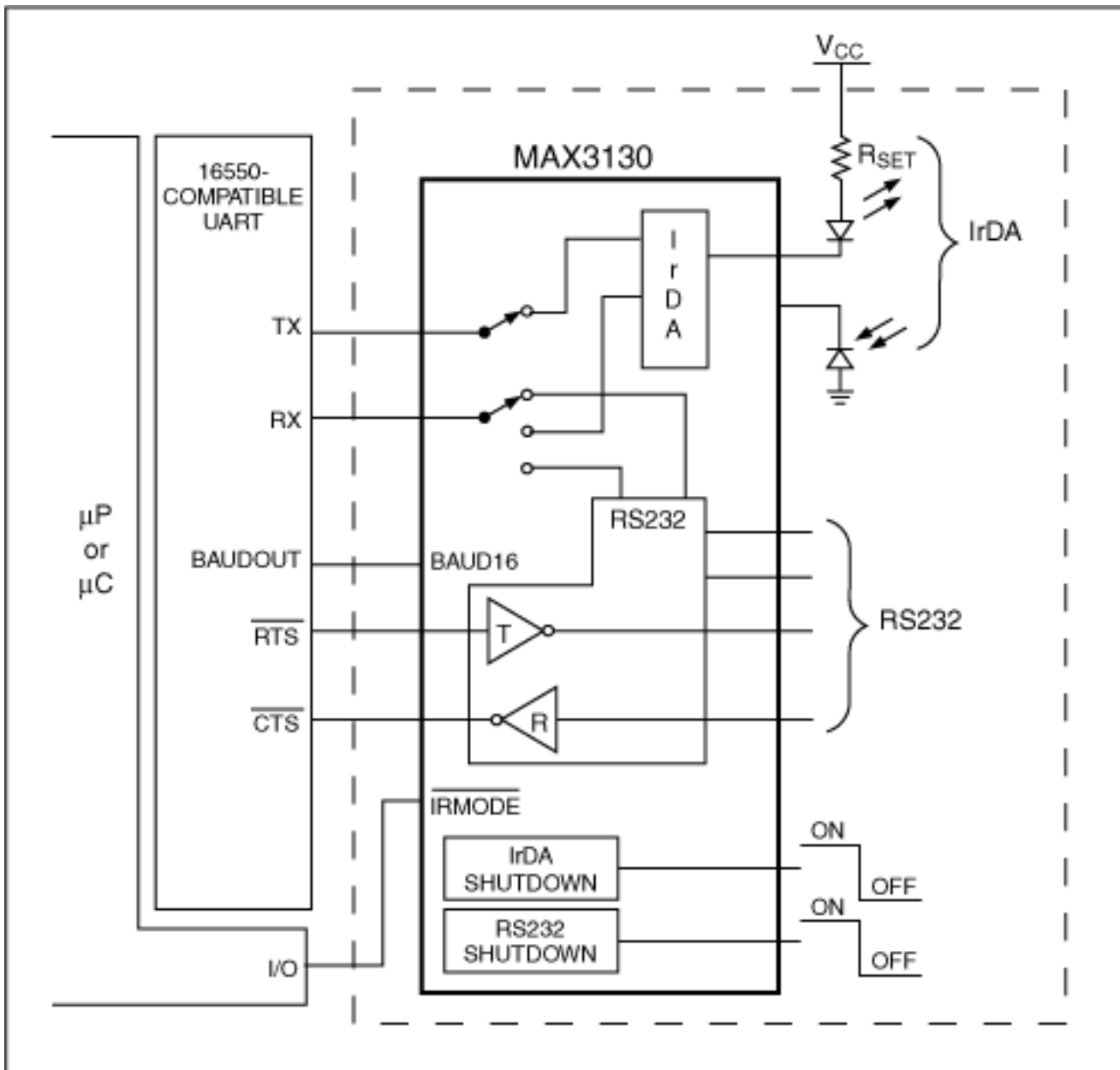
Figure 5. A better single-UART approach implements IrDA and RS-232 using only one IC.
