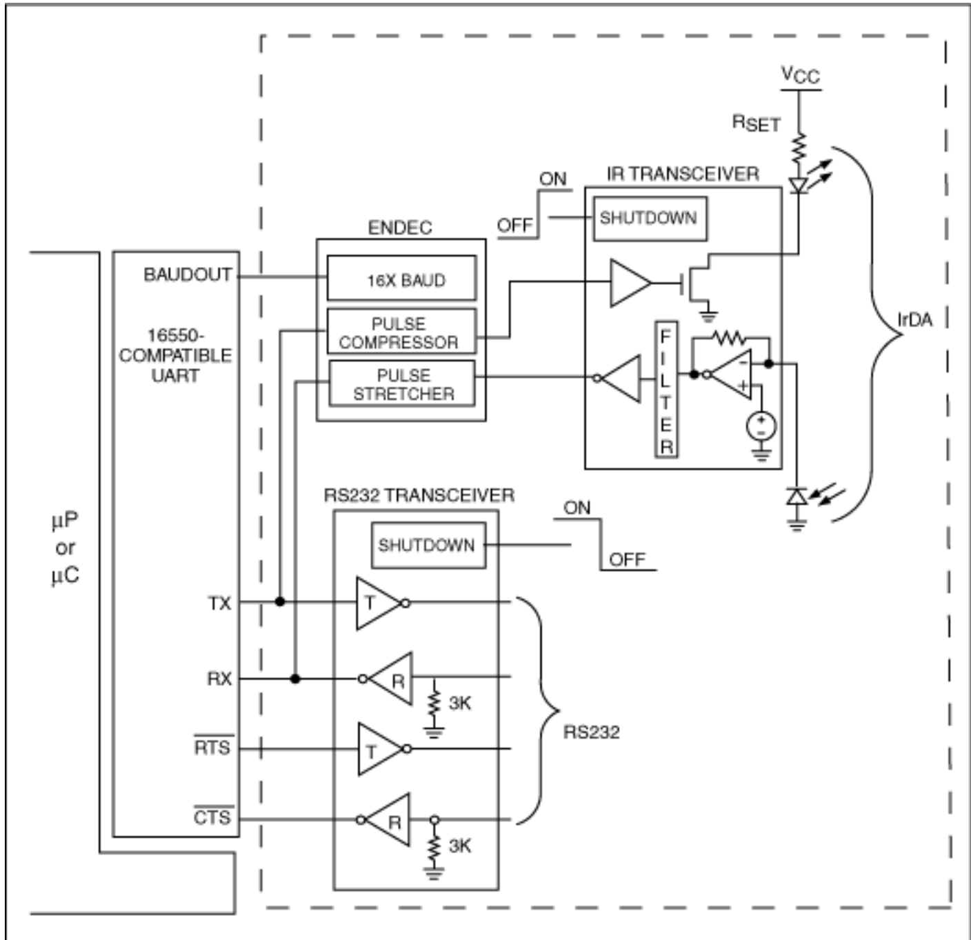
Figure 4. This alternative single-UART approach implements IrDA and RS-232 using three ICs.
