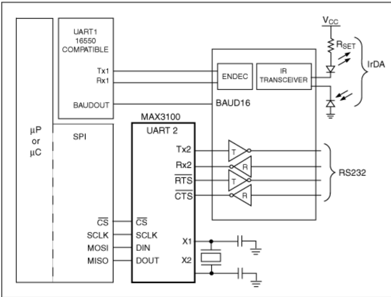
Figure 8. World's smallest hardware UART (MAX3100) interfaces to a microprocessor (or microcontroller) via a SPI port to provide a second UART.
