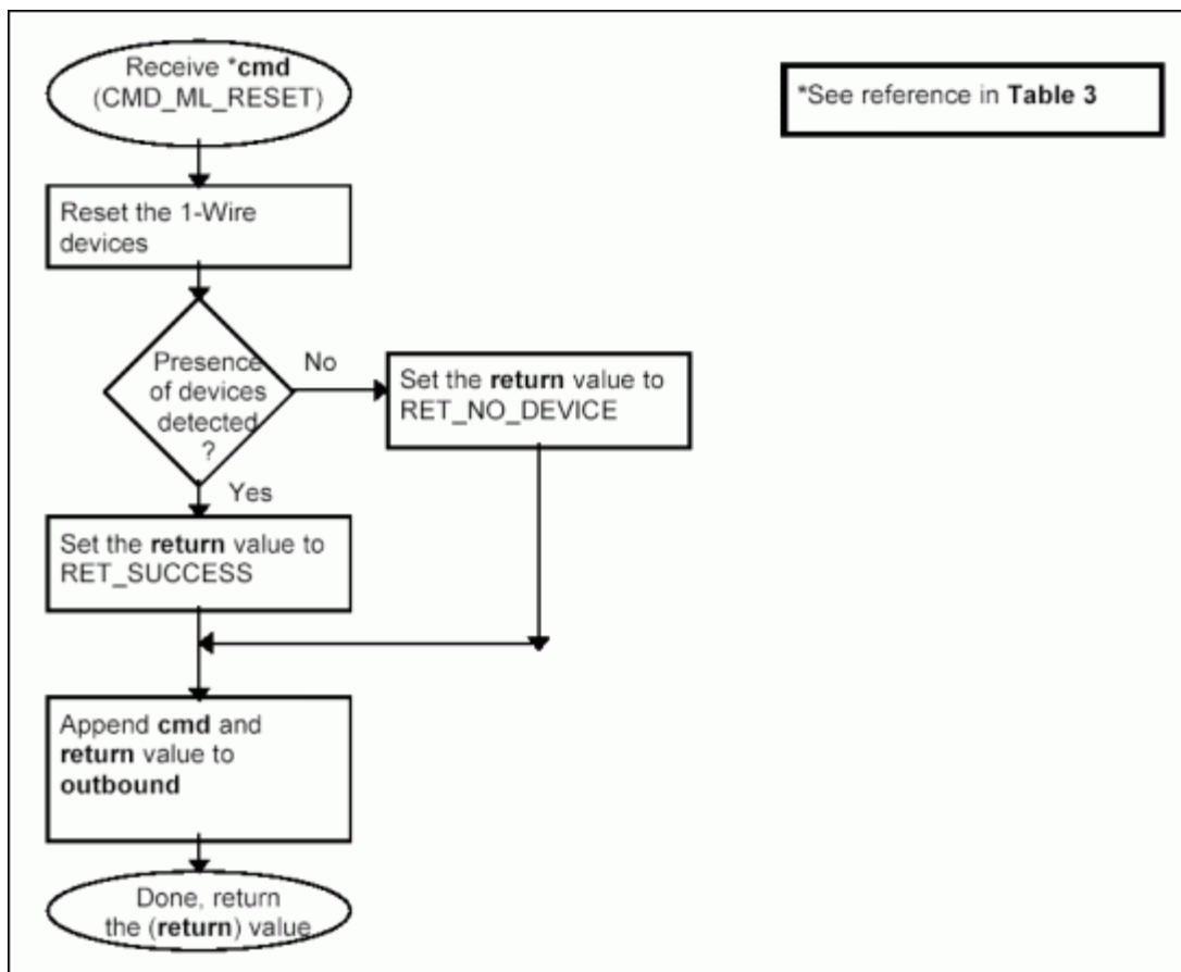
Figure 3a. Processing command CMD_ML_RESET.
