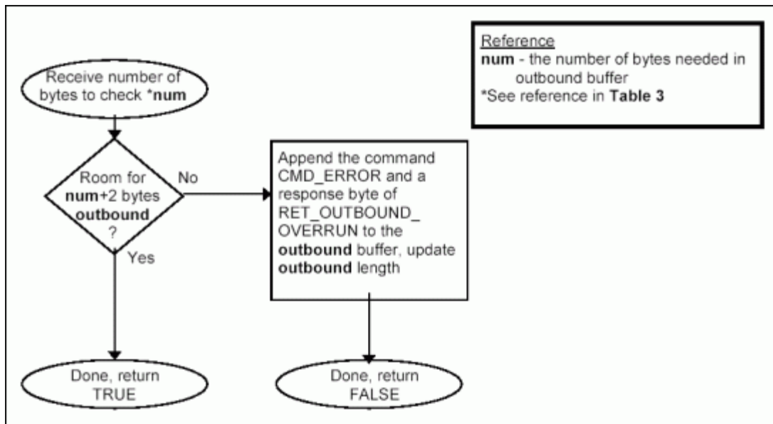
Figure 2c. Outbound space verification.
