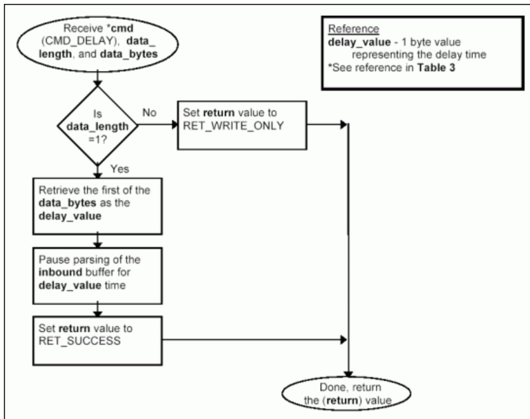
Figure 3j. Processing command CMD_DELAY.
