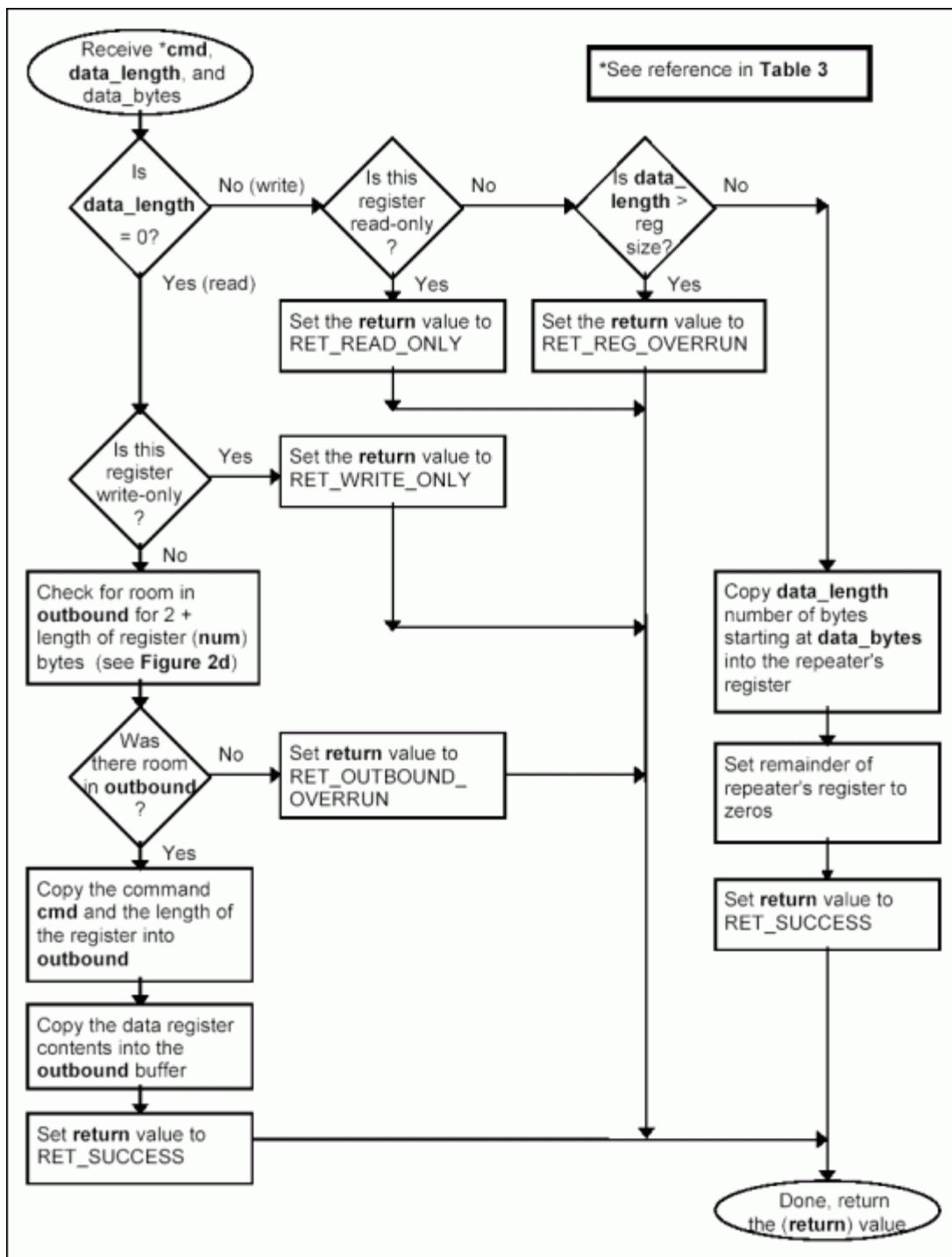
Figure 3g. Processing data register commands.
