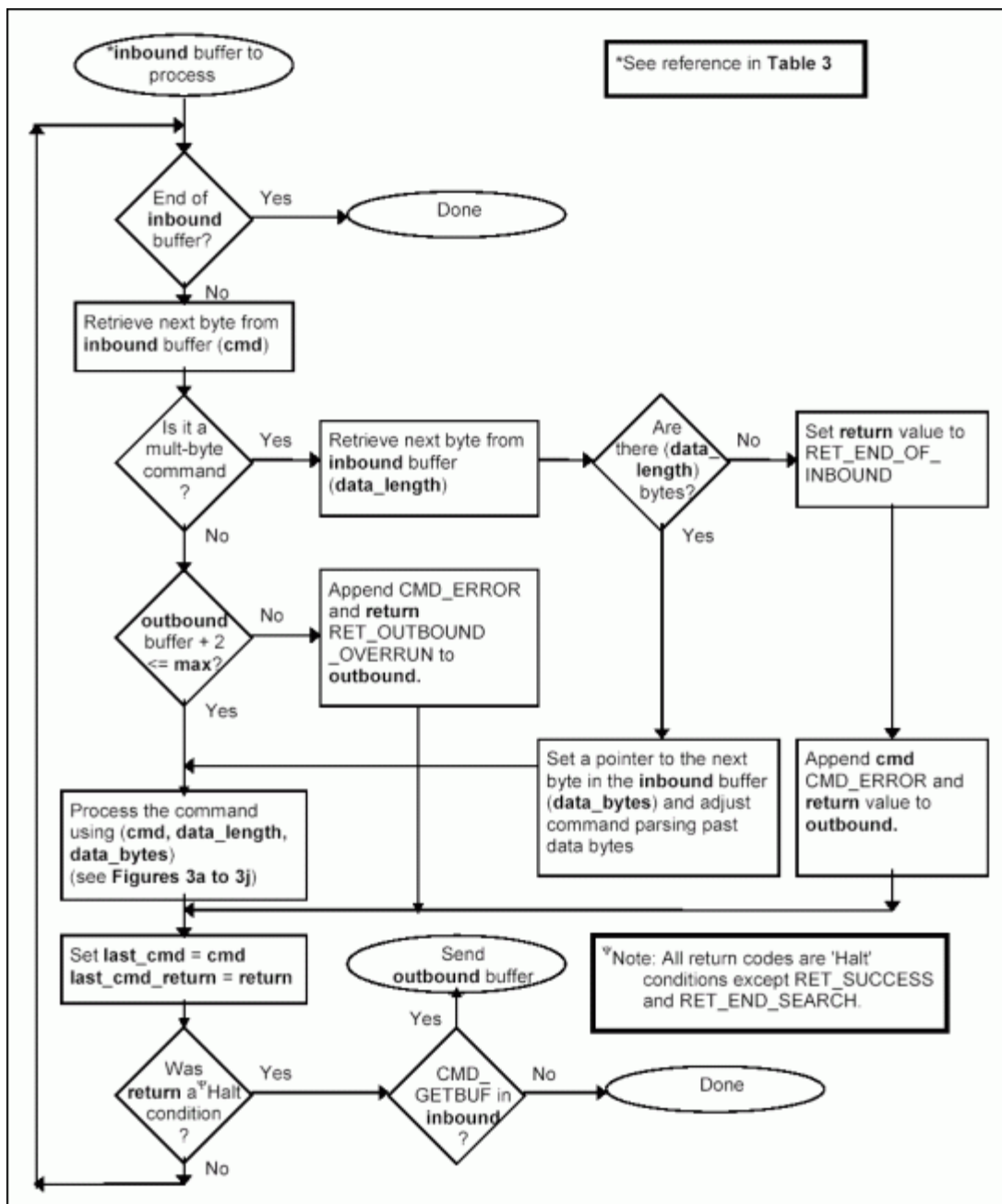
Figure 2b. Inbound command processing.
