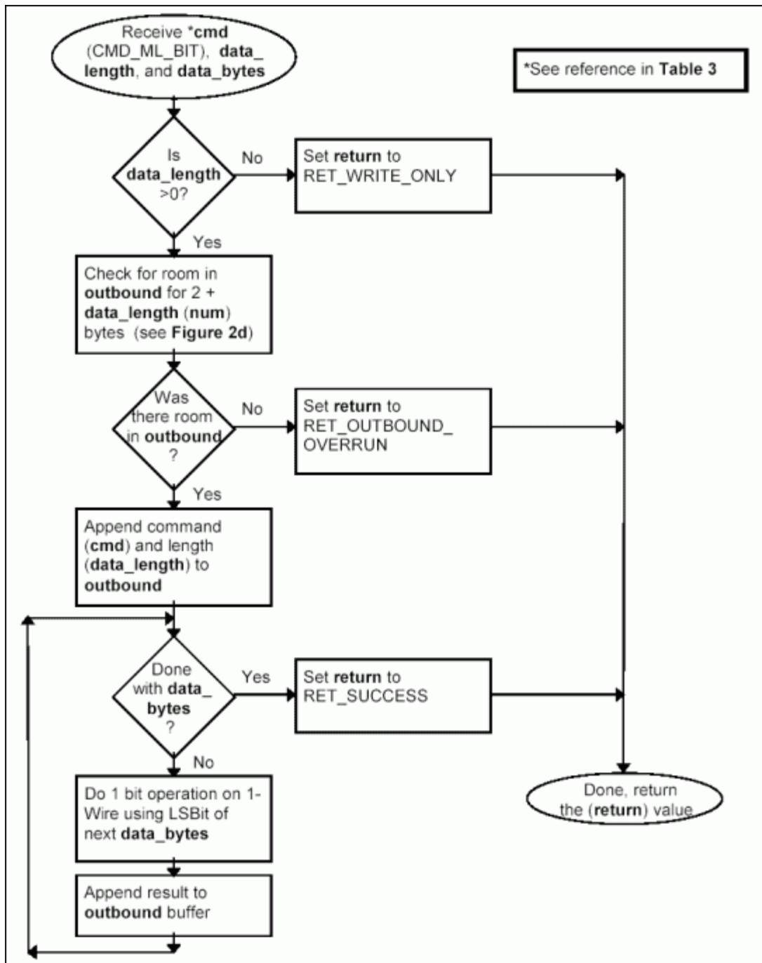
Figure 3h. Processing command CMD_ML_BIT.
