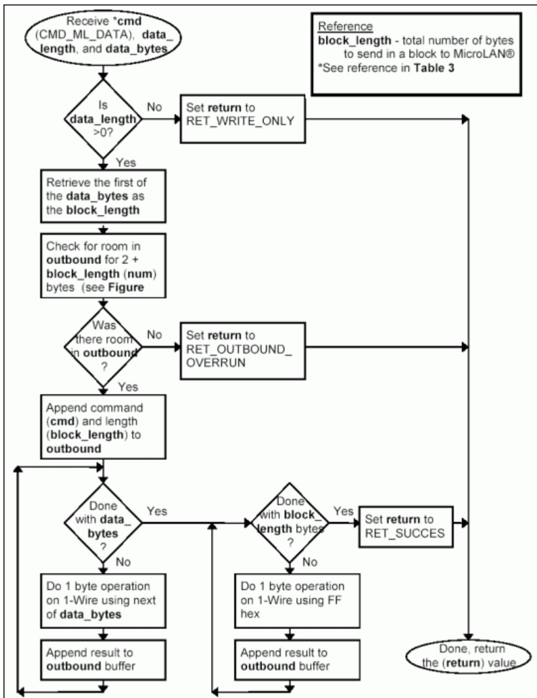
Figure 3i. Processing command CMD_ML_DATA.
