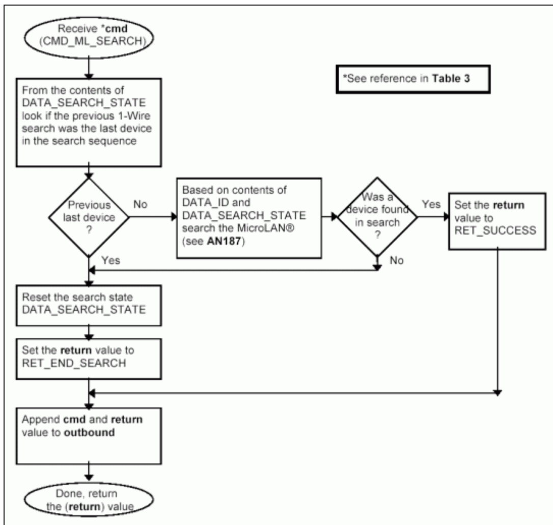
Figure 3b. Processing command CMD_ML_SEARCH.
