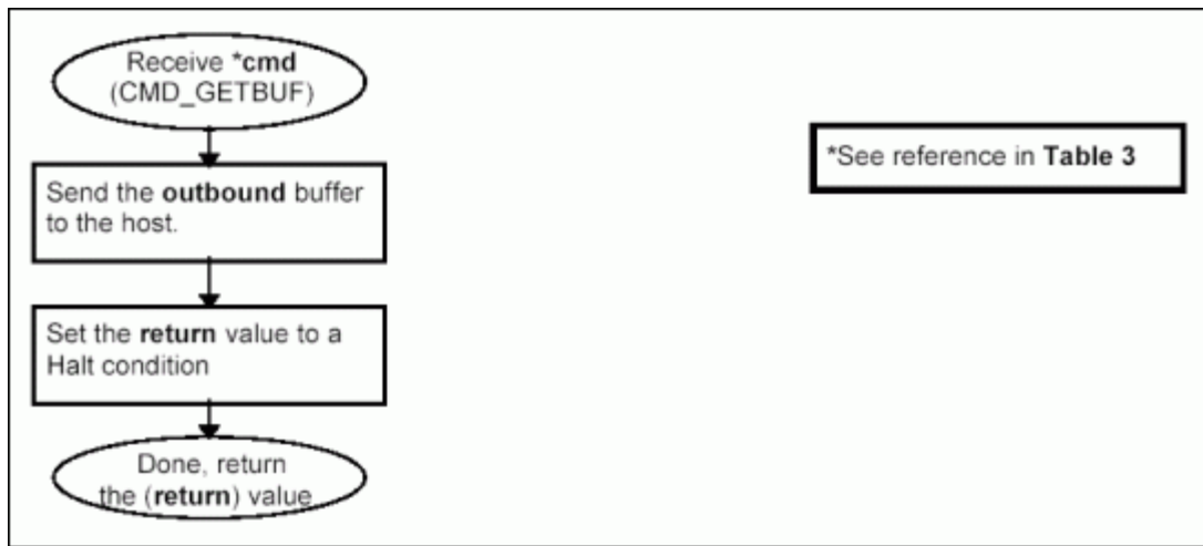
Figure 3f. Processing command CMD_GETBUF.
