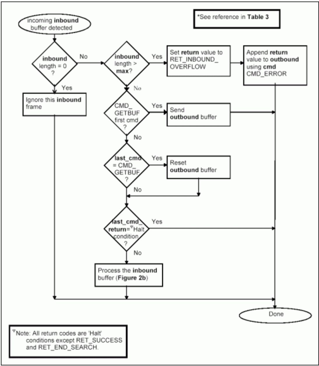
Figure 2a. Receiving inbound buffer.
