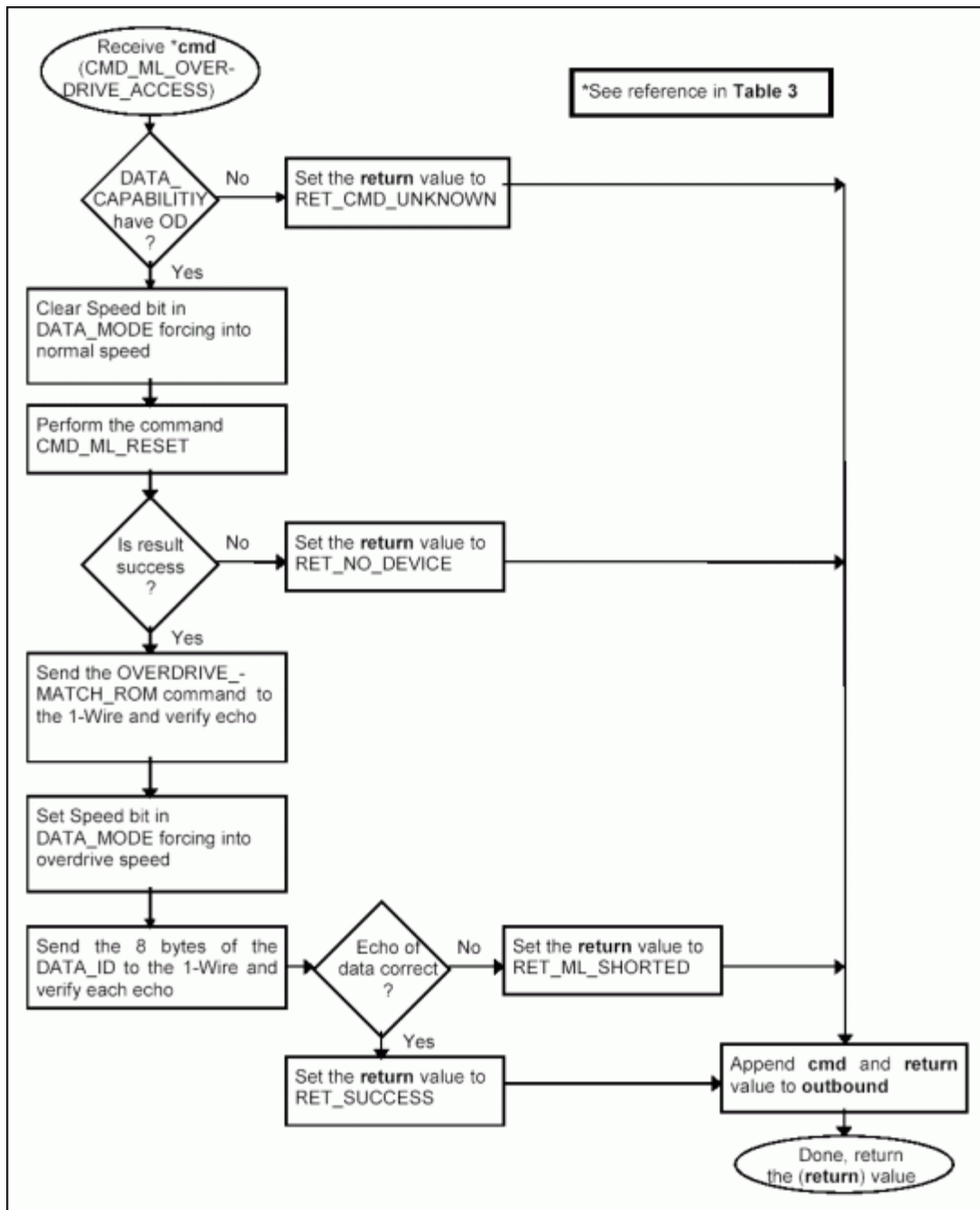
Figure 3d. Processing command CMD_ML_OVERDRIVE_ACCESS.
