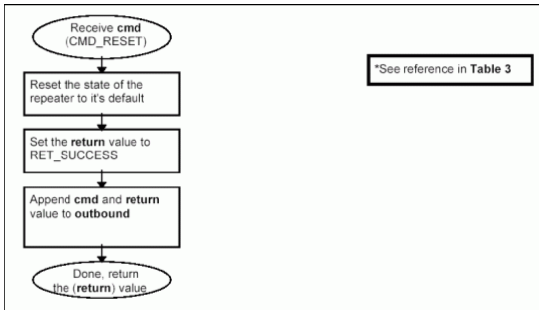
Figure 3e. Processing command CMD_RESET.
