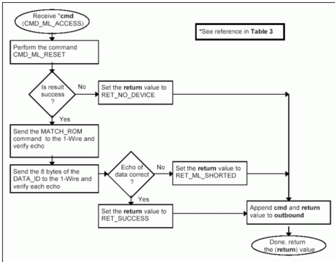
Figure 3c. Processing command CMD_ML_ACCESS.
