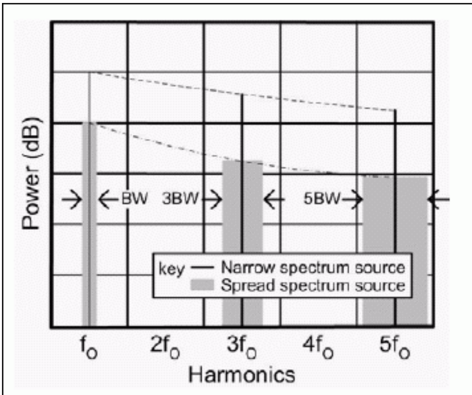
Figure 3. Spectral content for dithered oscillator harmonics.
