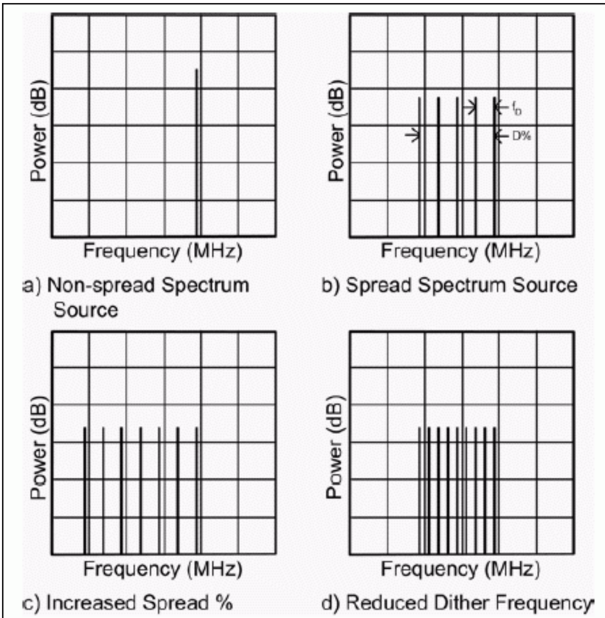
Figure 1. Spectral components of non-dithered and dithered oscillators.
