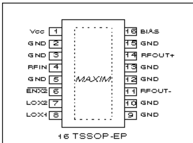
Figure 2. Pin description of the MAX2683.
