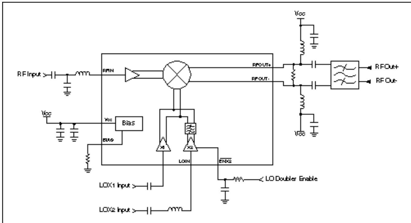
Figure 1. Simplified block diagram of a MAX2683 application.
