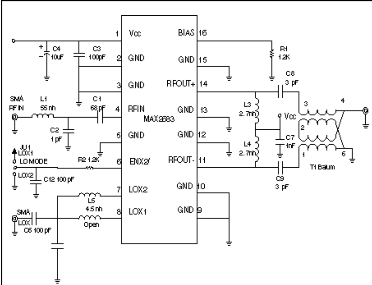
Figure 3. Application Schematic of the MAX2683.
