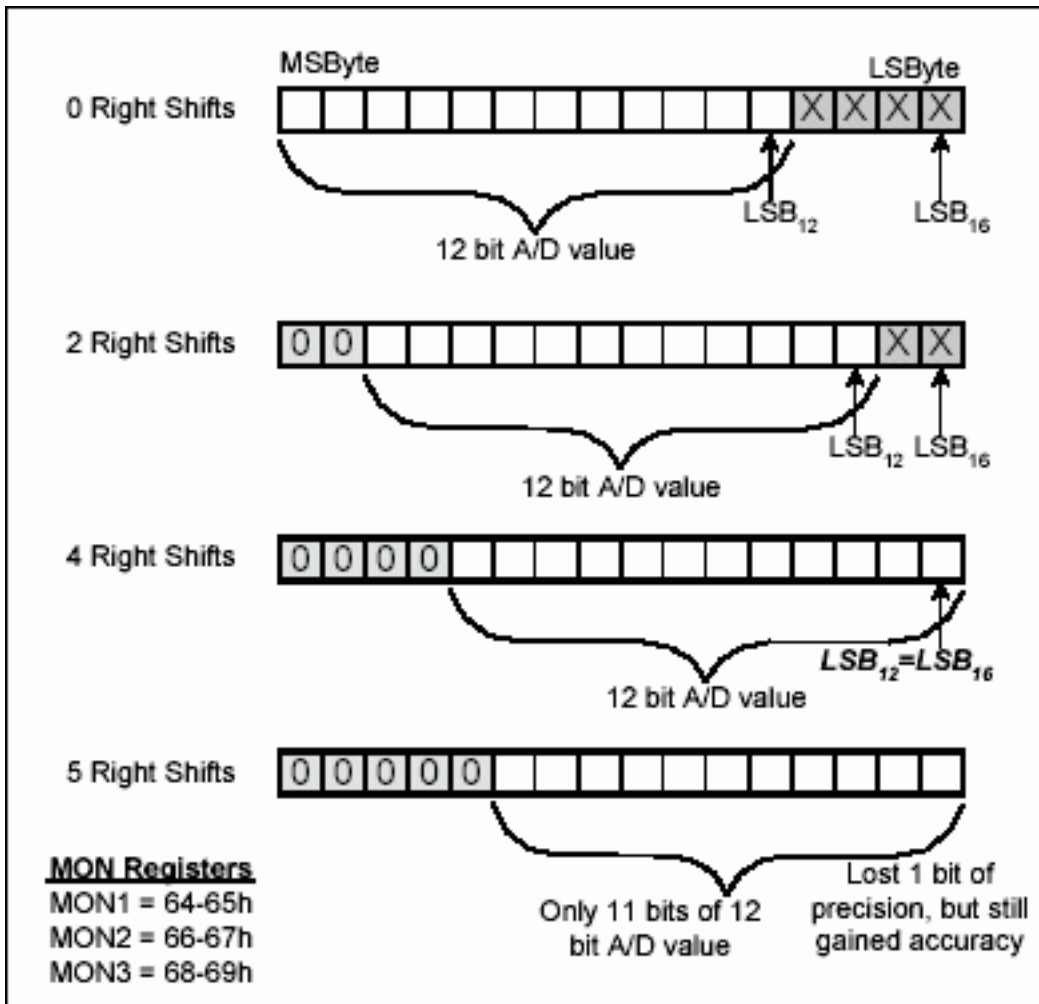
Figure 3. MON register right shifting examples.
