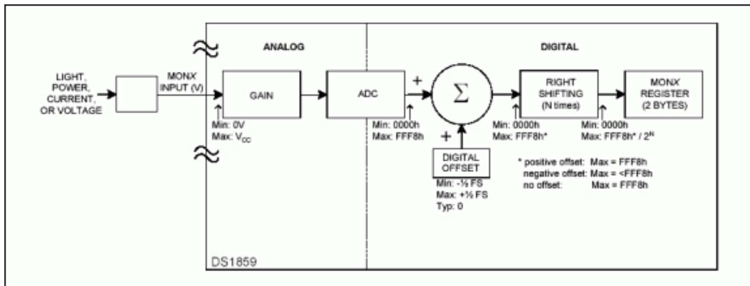
Figure 1. DS1859 MON input block diagram.
