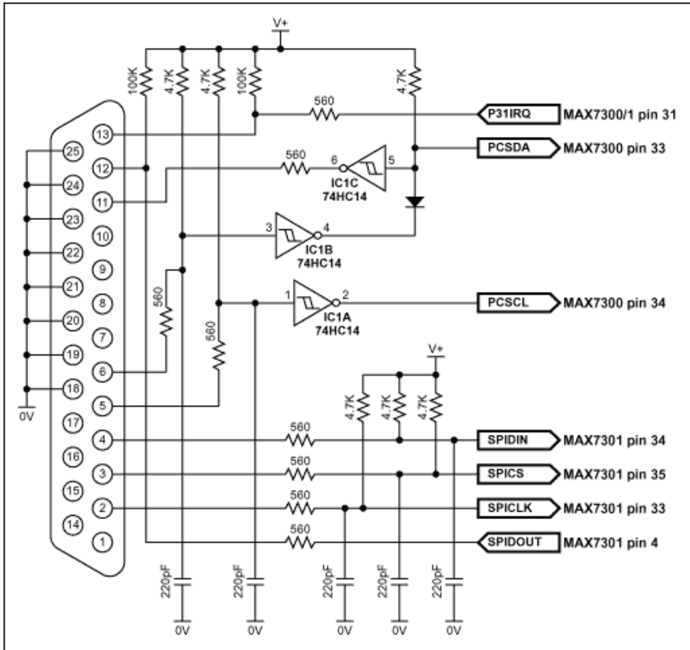
Figure 1. The MAX7300 and MAX7301 connections to the parallel port.
