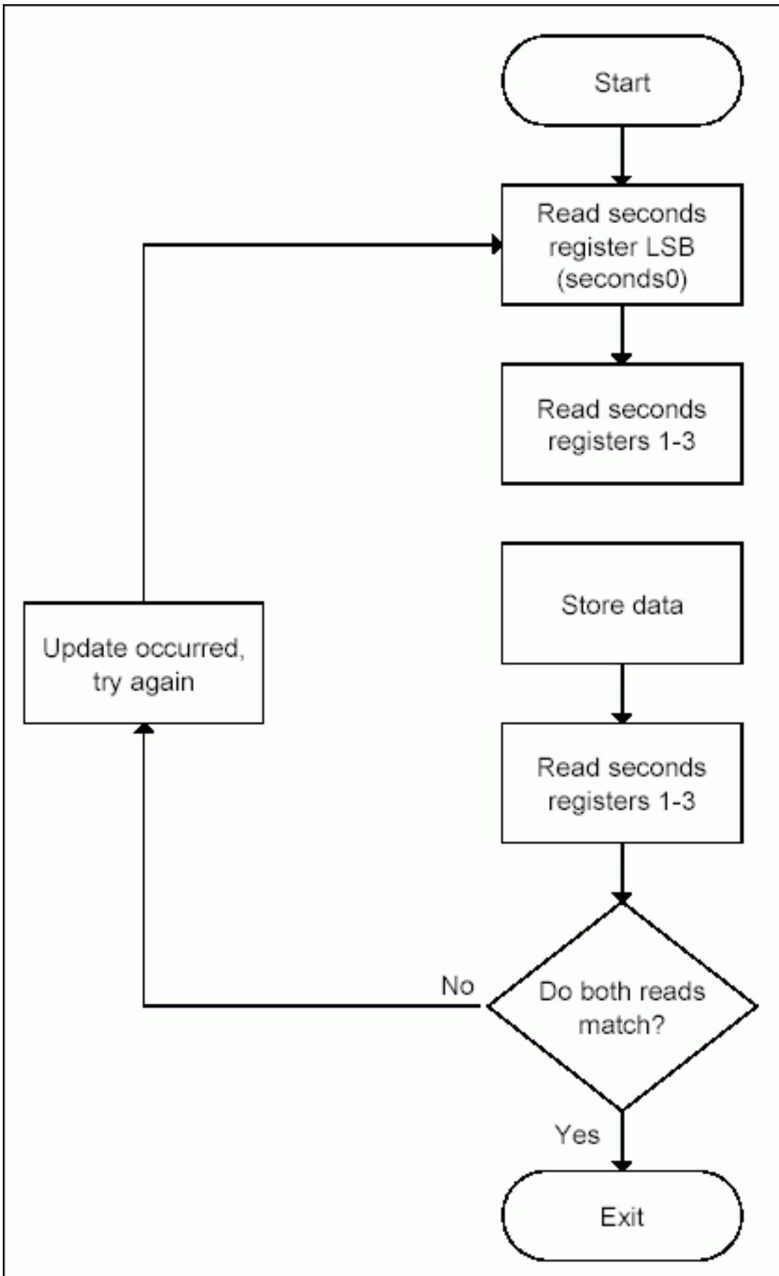
Figure 1. Reading the clock registers between updates.
