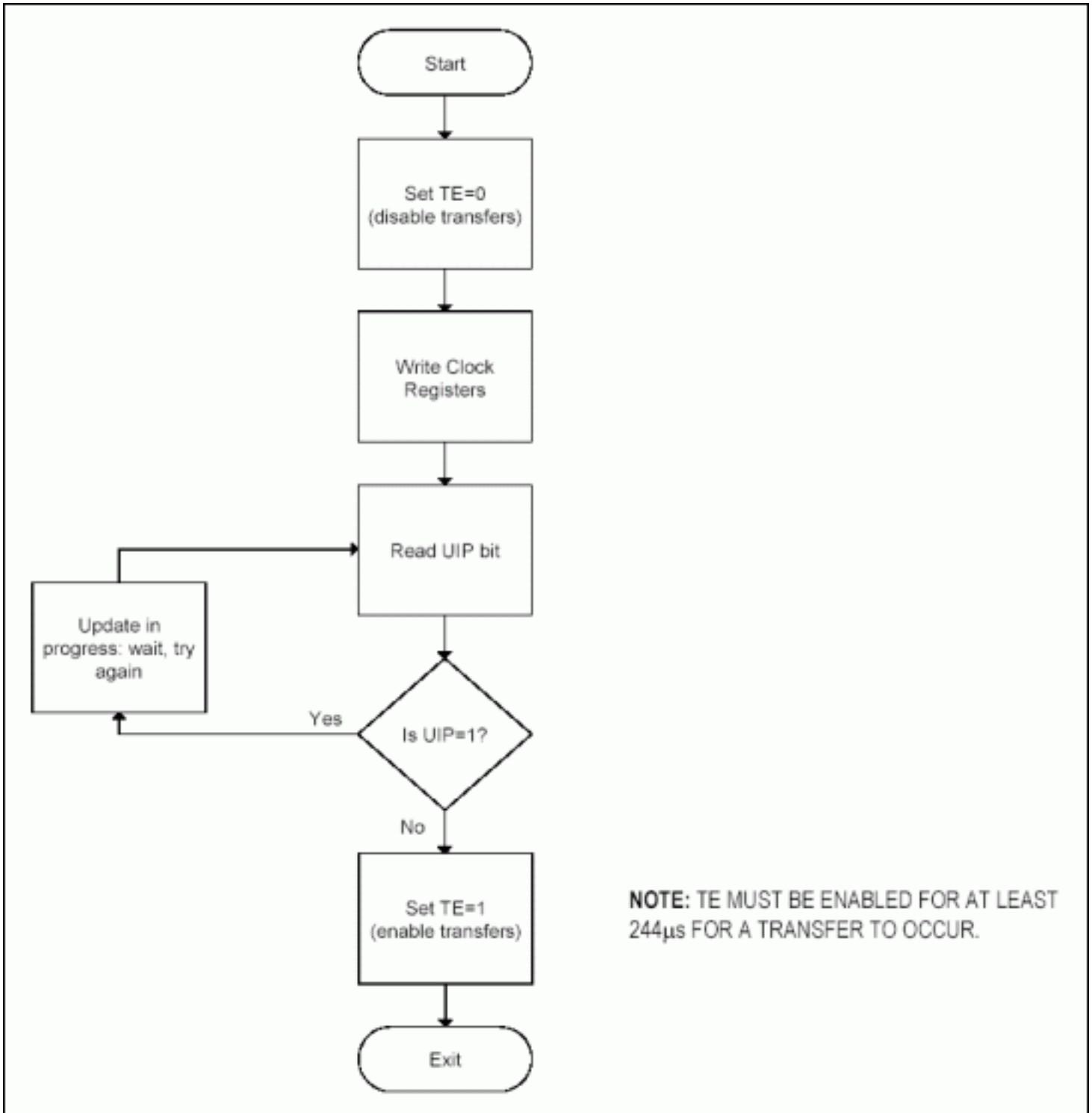
Figure 5. Writing the clock registers using the TE and UIP bits.
