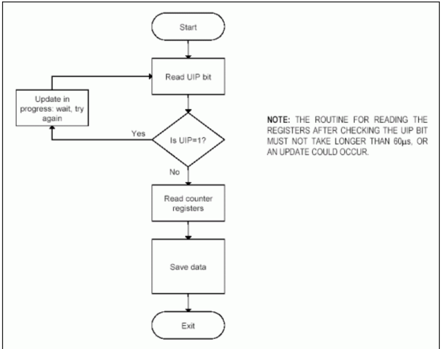
Figure 2. Reading the clock registers using the UIP bit.
