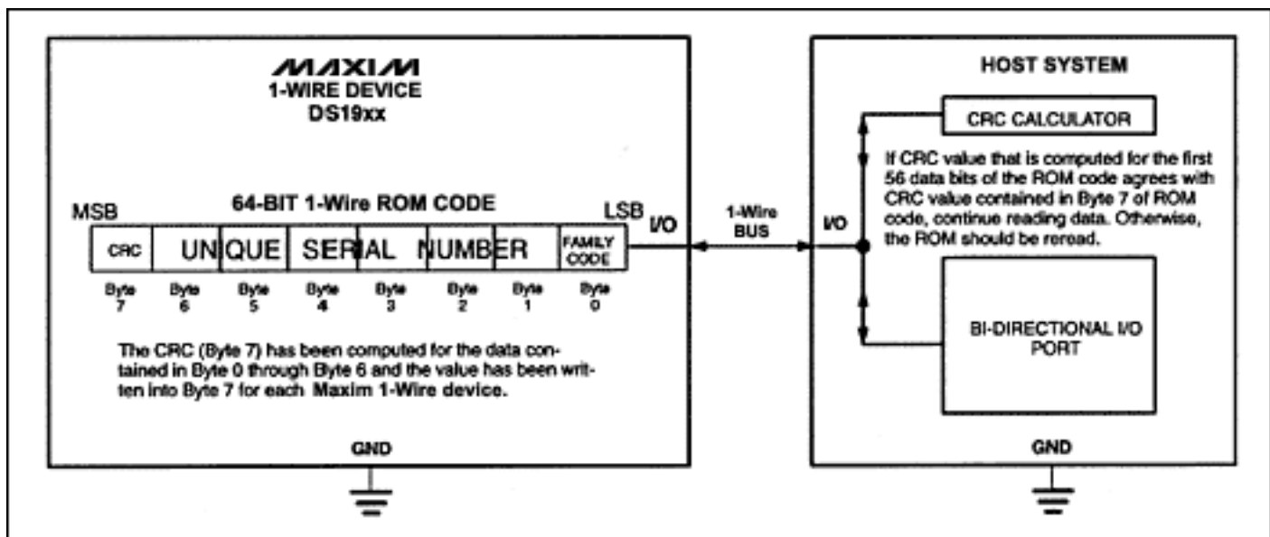
Figure 1. iButton system configuration using DOW CRC.
