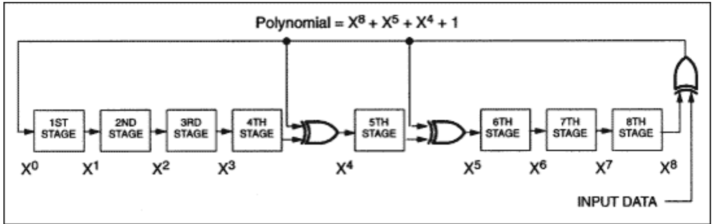
Figure 2. Maxim 1-Wire 8-bit CRC.
