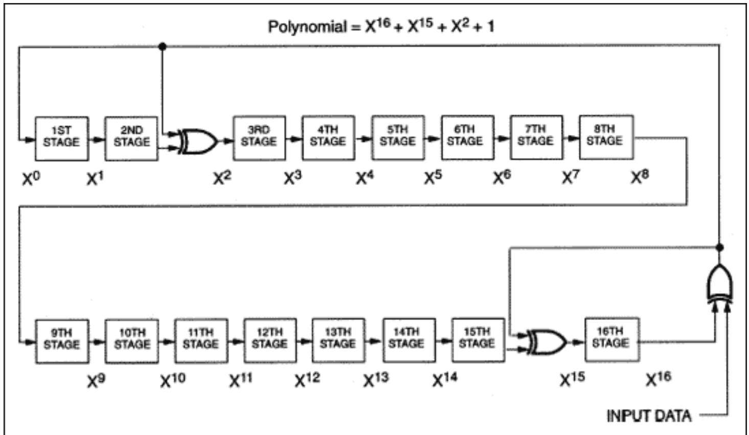
Figure 3. CRC-16 hardware description and polynomial.
