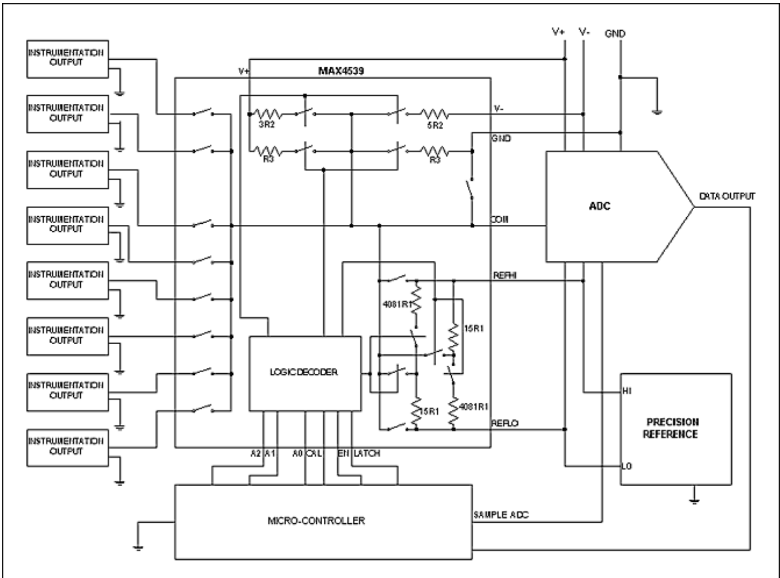
Figure 1. The MAX4539 cal-mux simplifies calibration of a multi-channel industrial control system.
