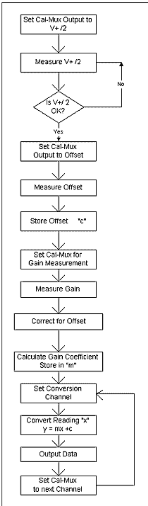
Figure 2. This flow chart details a calibration procedure implemented in the Figure 1 system.
