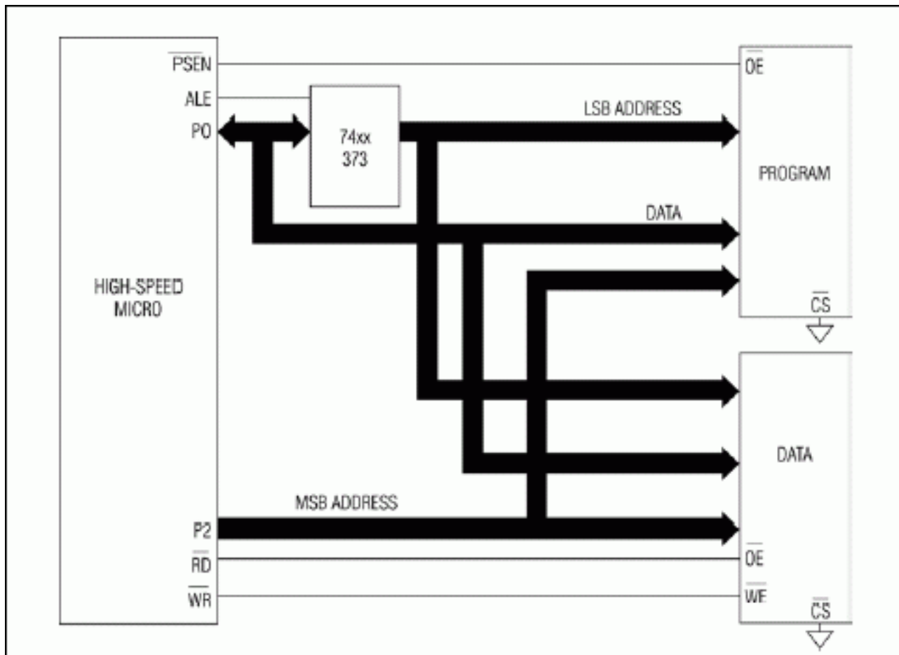
Figure 1. Non-page mode memory interface.
