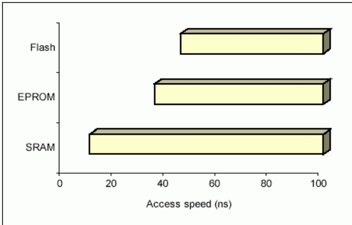
Figure 4. Representation of access times of memory types.
