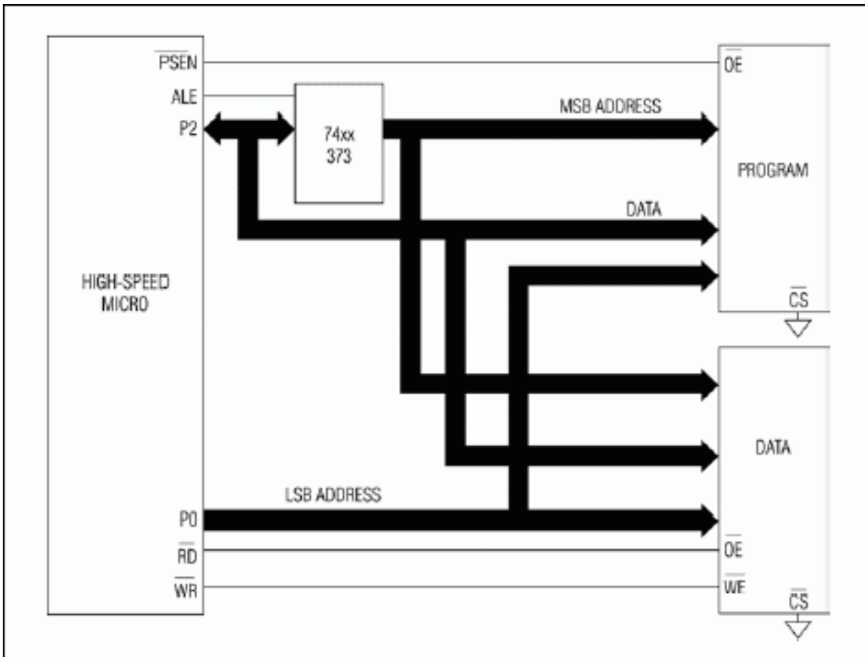
Figure 3. Page mode 2 memory interface.
