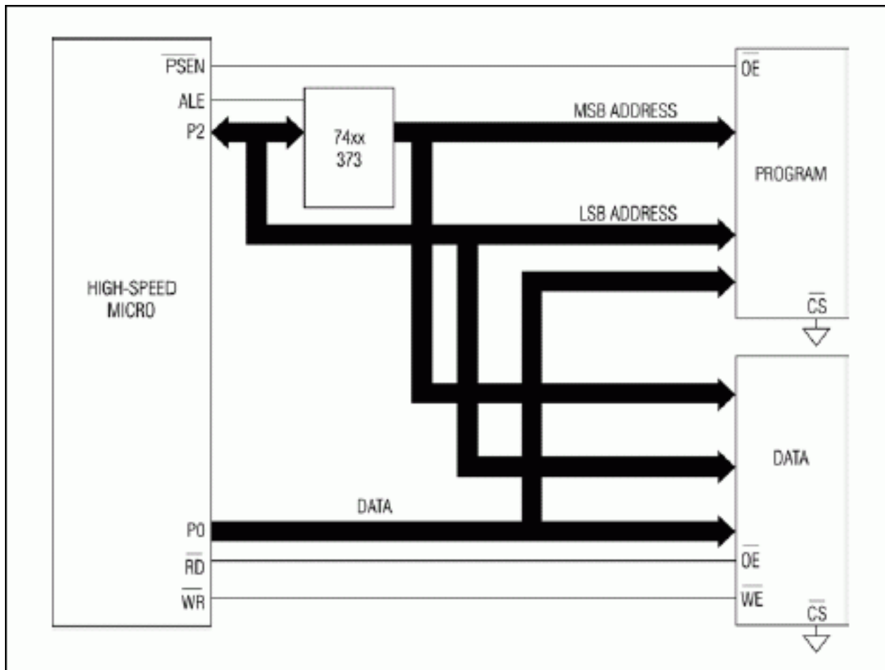
Figure 2. Page mode 1 memory interface.
