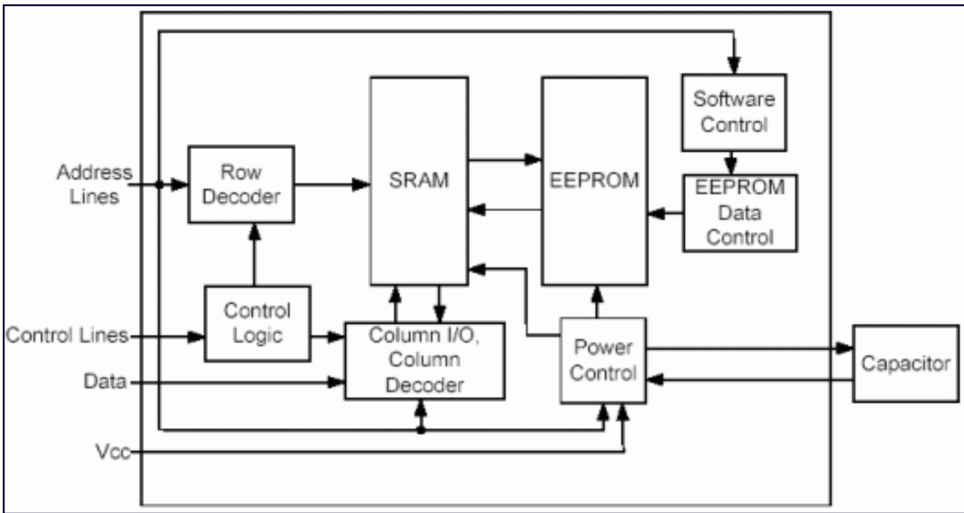
Figure 2. NOVRAMs.
