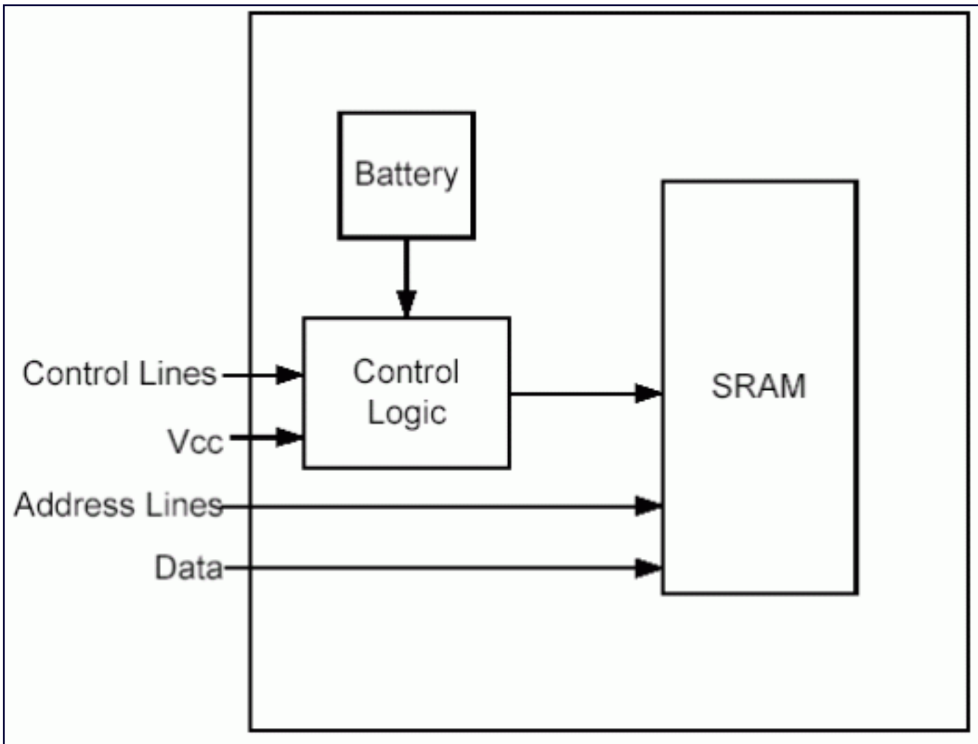
Figure 1. Battery-backed NVSRAM.
