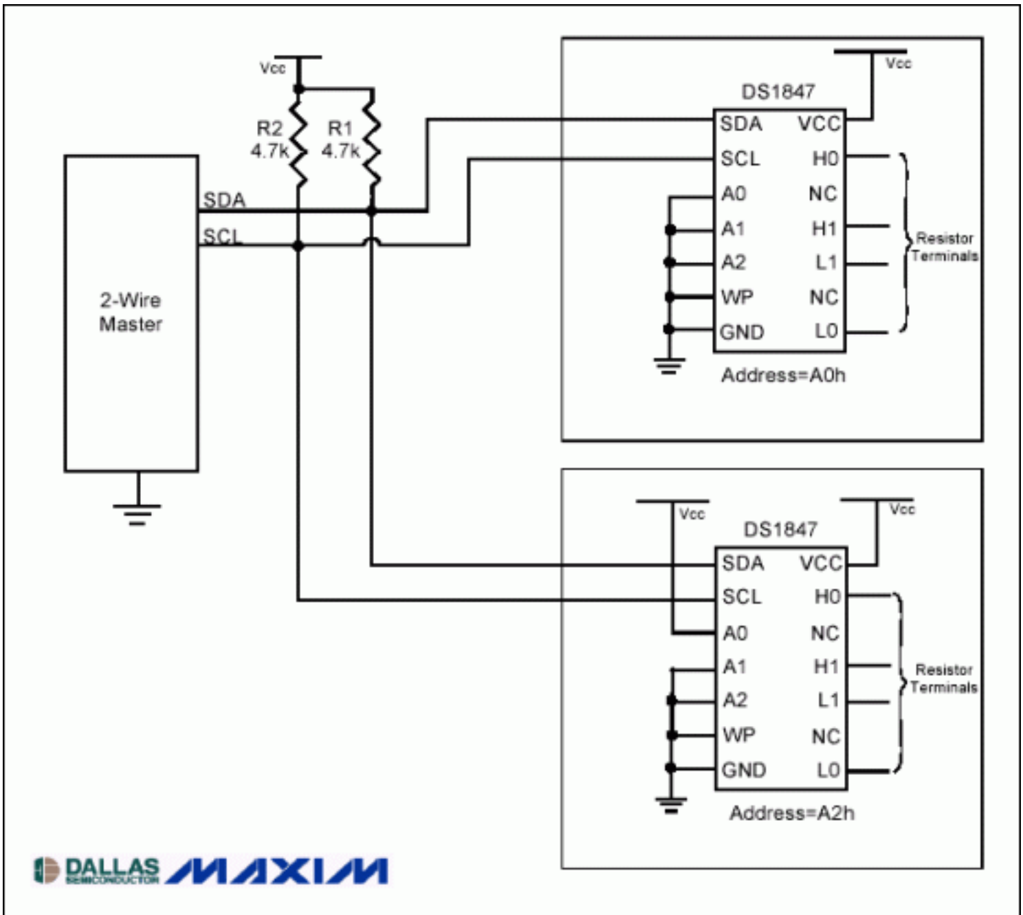
Figure 2. 2-Wire interface.
