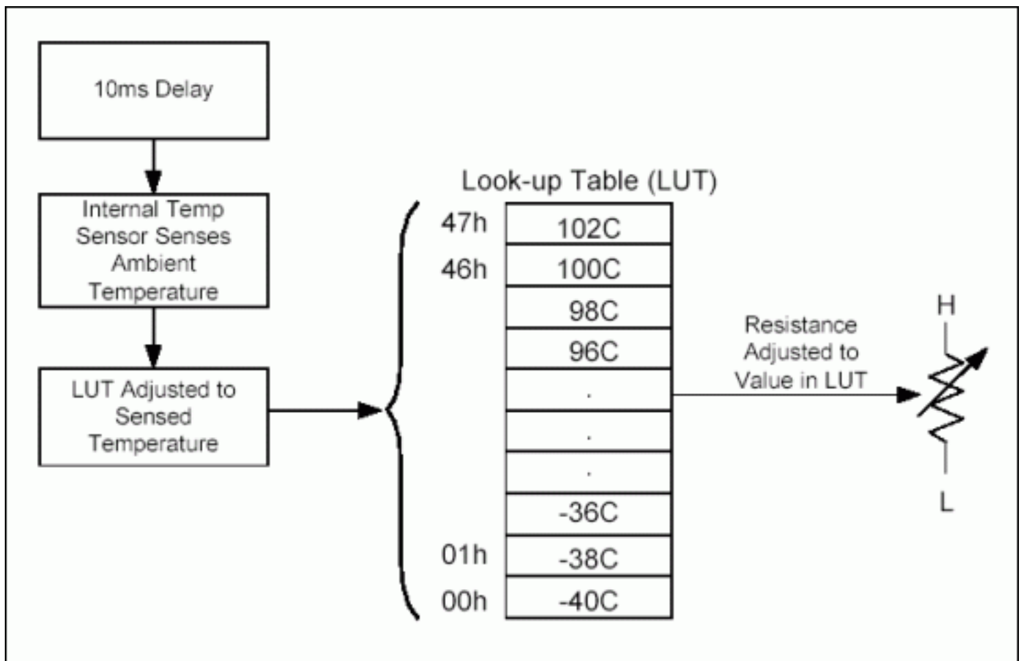
Figure 3. Lookup table.
