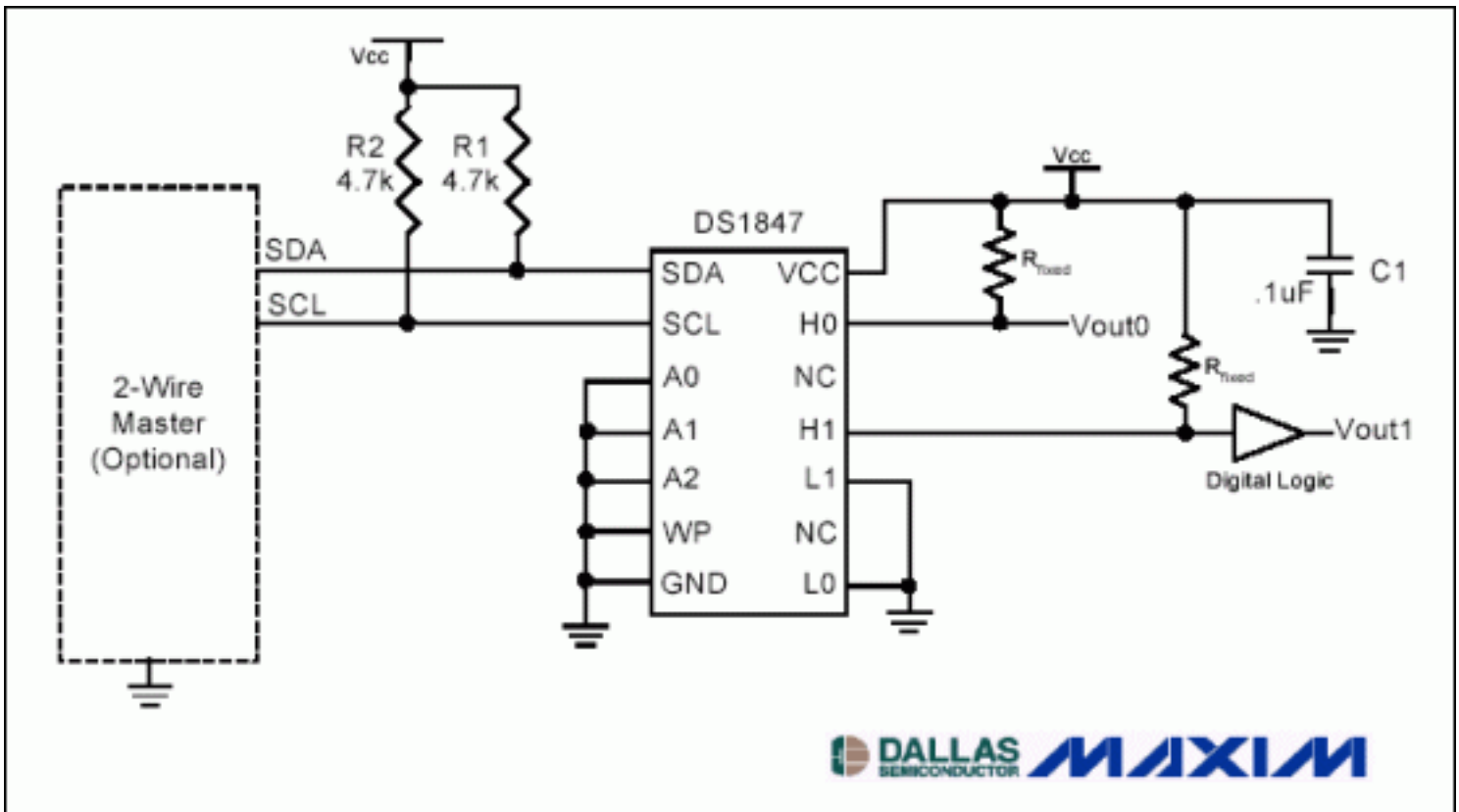
Figure 4. Voltage and digital outputs.
