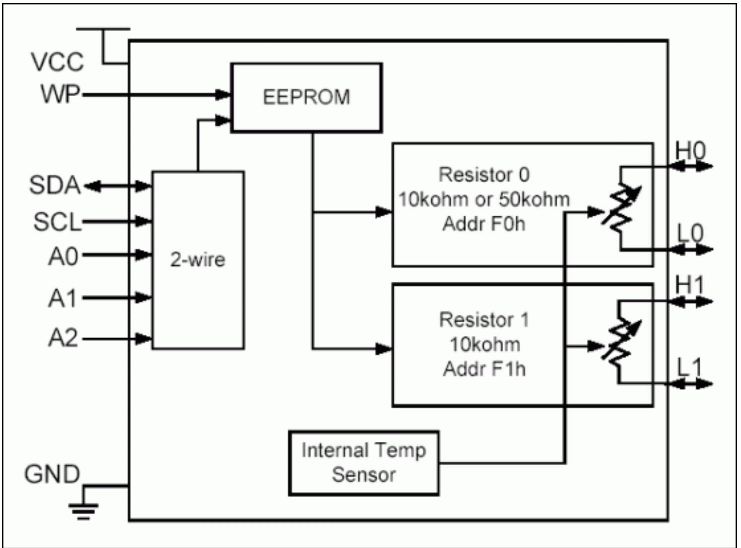
Figure 1. Block diagram.
