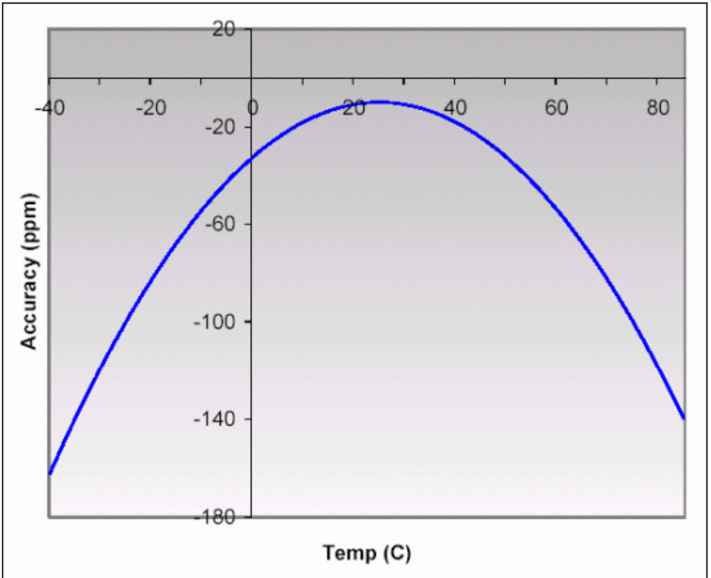
Figure 1. Typical tuning fork crystal behavior.
