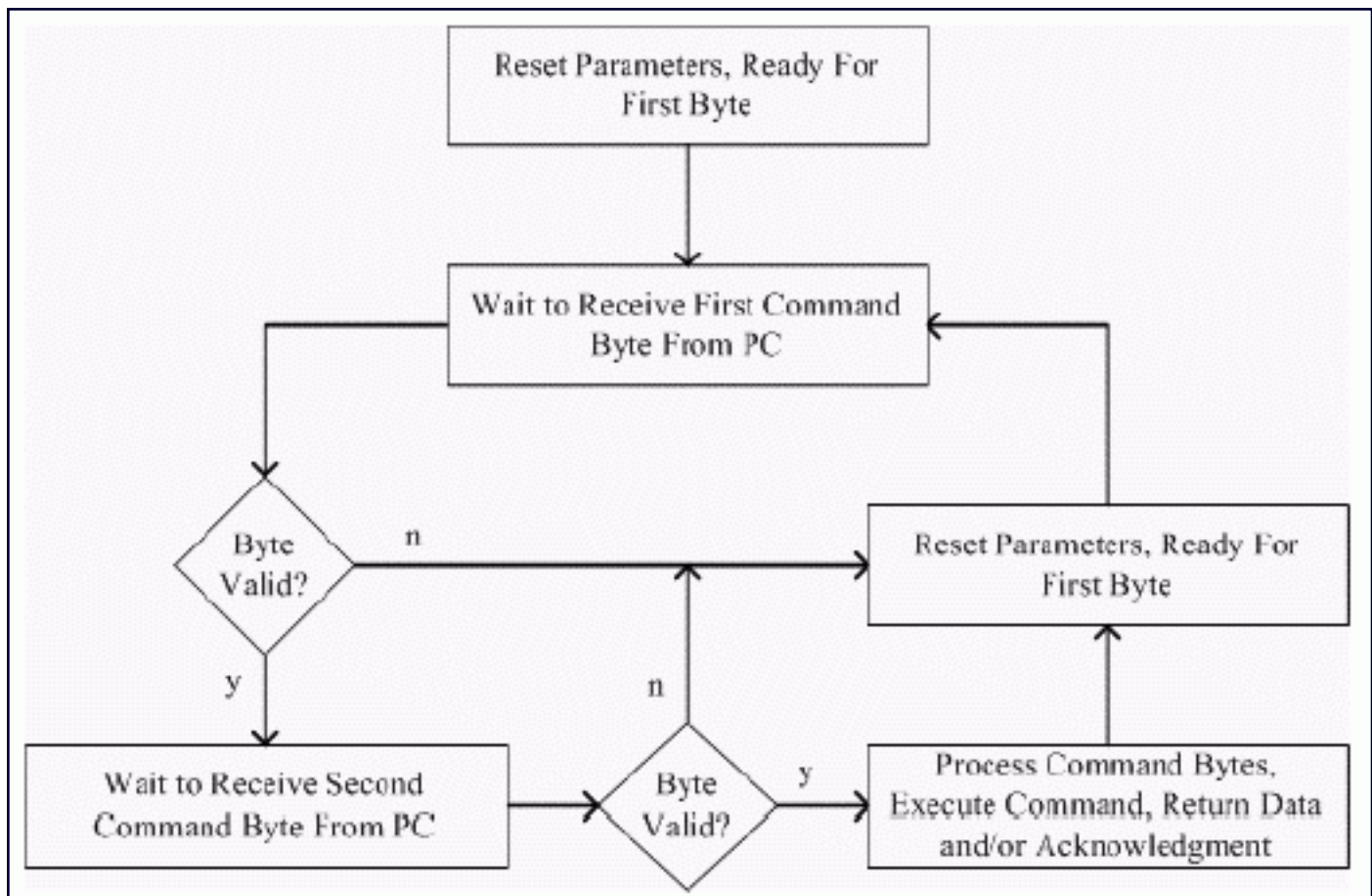
Figure 5. Firmware program flow.
