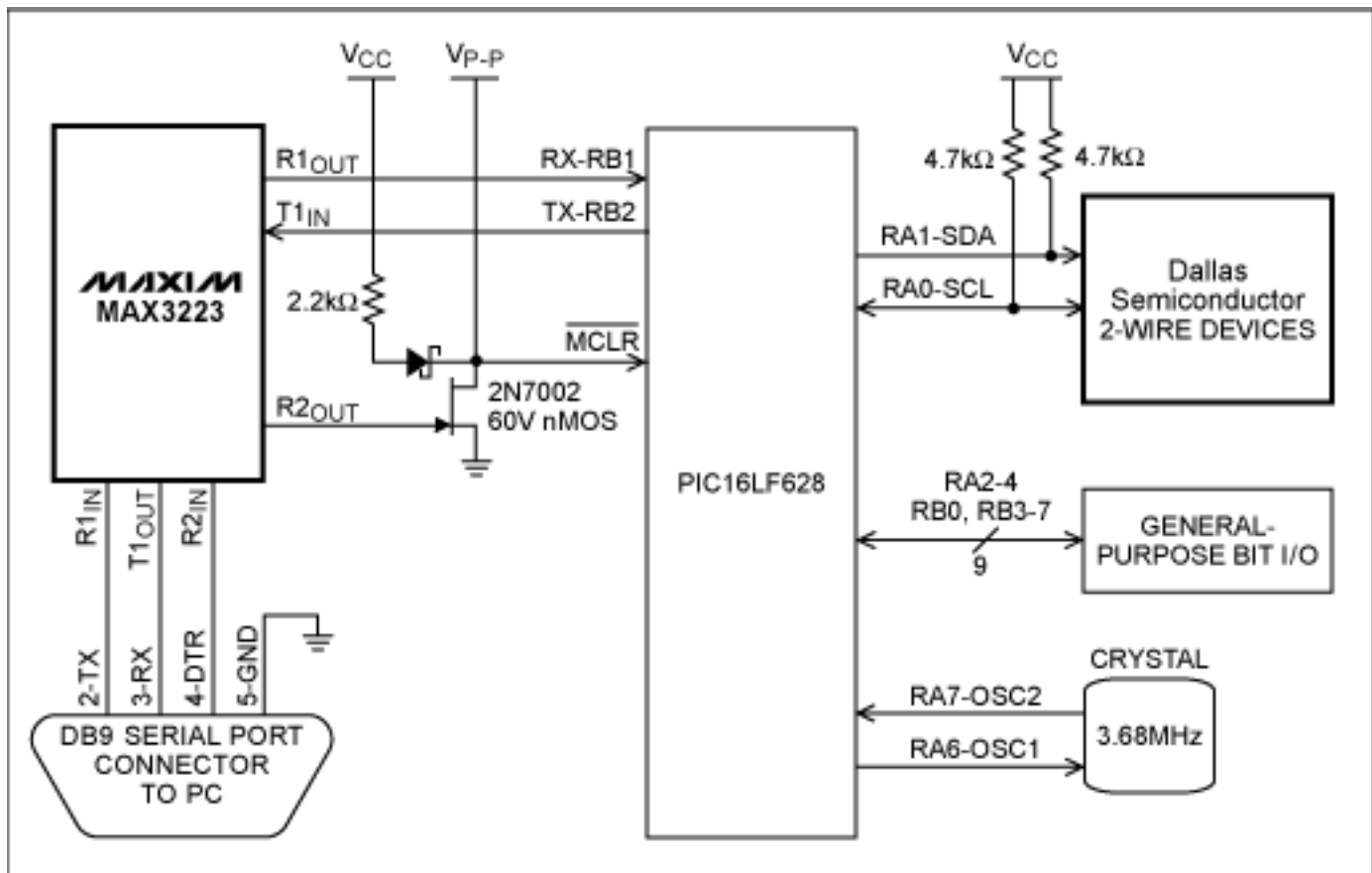
Figure 1. Reference design's hardware block diagram.
