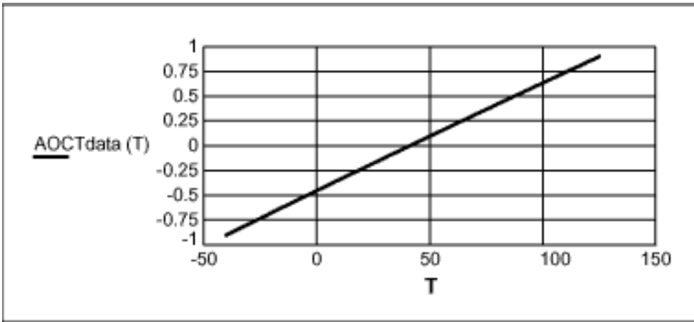
Figure 5. Amplified offset corrected temperature data \times temperature ( ^{\circ}\text{C} ). where
