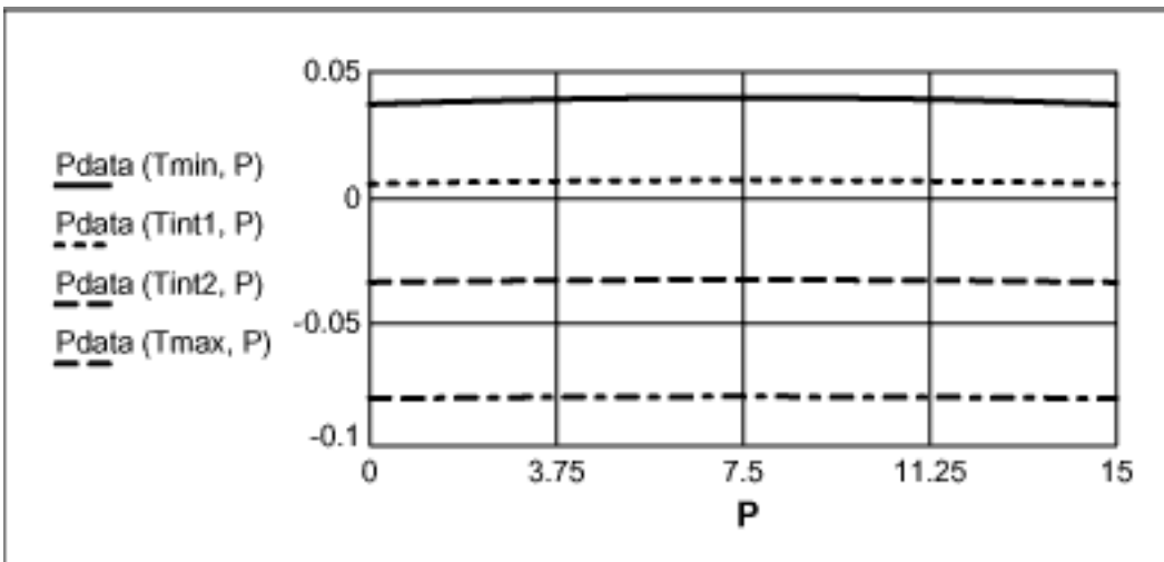
Figure 11. Sensor Offset and nonlinearity \times Pressure (psi)
