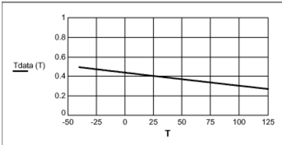
Figure 2. temperature ADC output x temperature( ^{\circ}\text{C} ).
