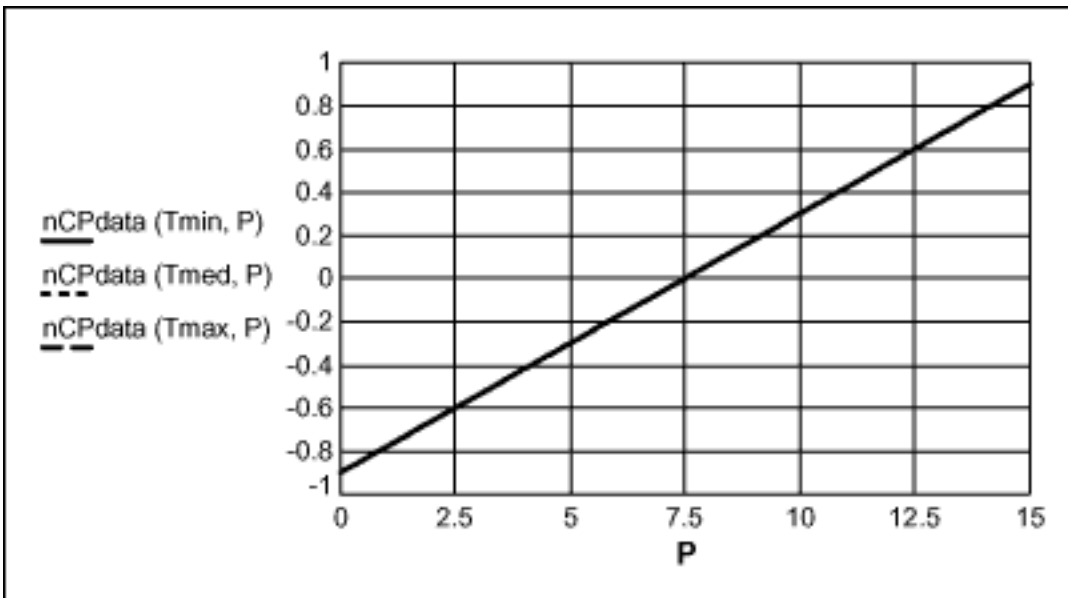
Figure 14. Normalized Corrected Sensor Data x Pressure (psi).
