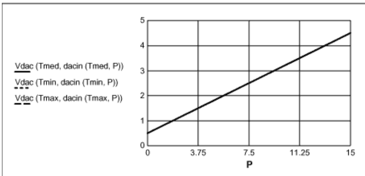
Figure 17. DAC output (V) x pressure (psi).
