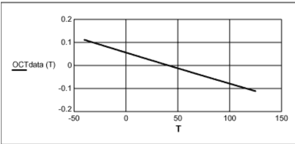
Figure 4. Offset corrected temperature data \times temperature ( ^{\circ}\text{C} ).
