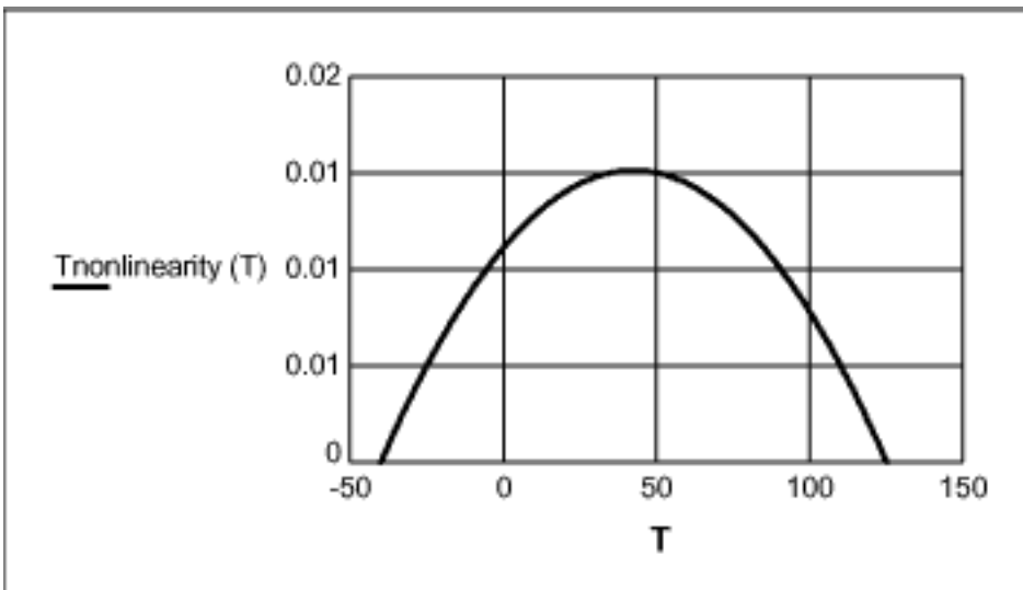
Figure 6. Nonlinearity of Temperature data \times Temperature ( ^{\circ}\text{C} ).
