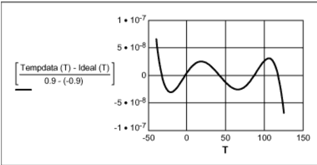
Figure 8. Linearity error of tempdata(T) x temperature (°C).
