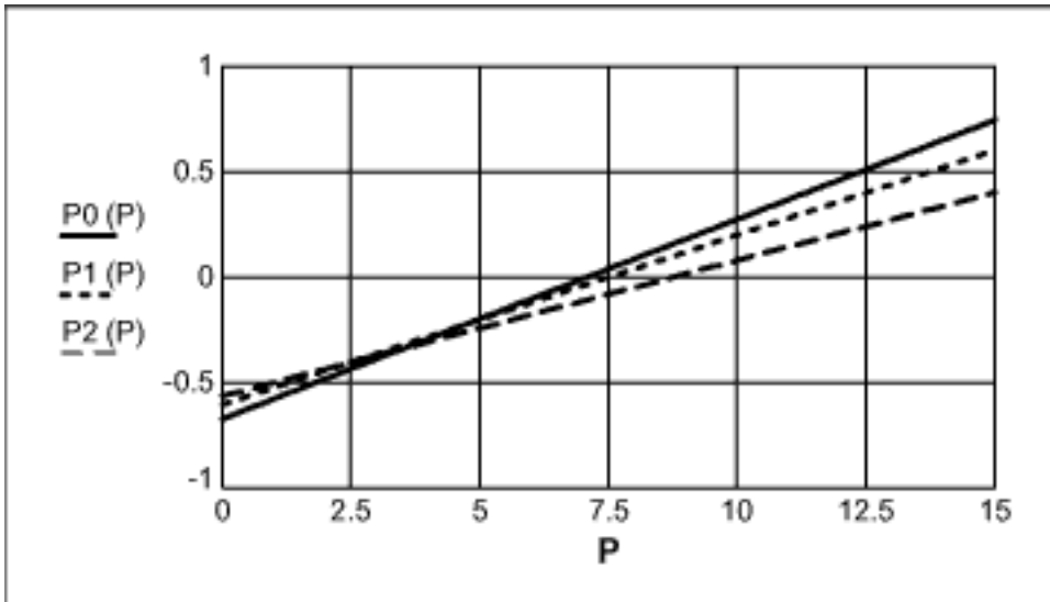
Figure 1. ADC output \times sensor excitation (psi).
