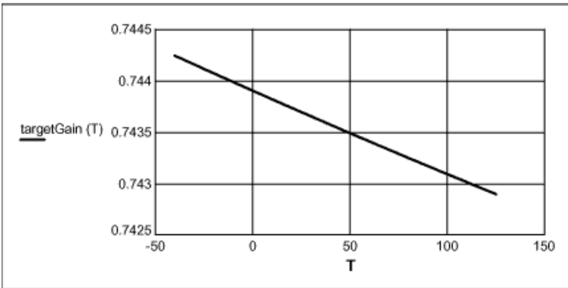
Figure 16. DAC gain correction \times temperature ( ^{\circ}\text{C} ).
