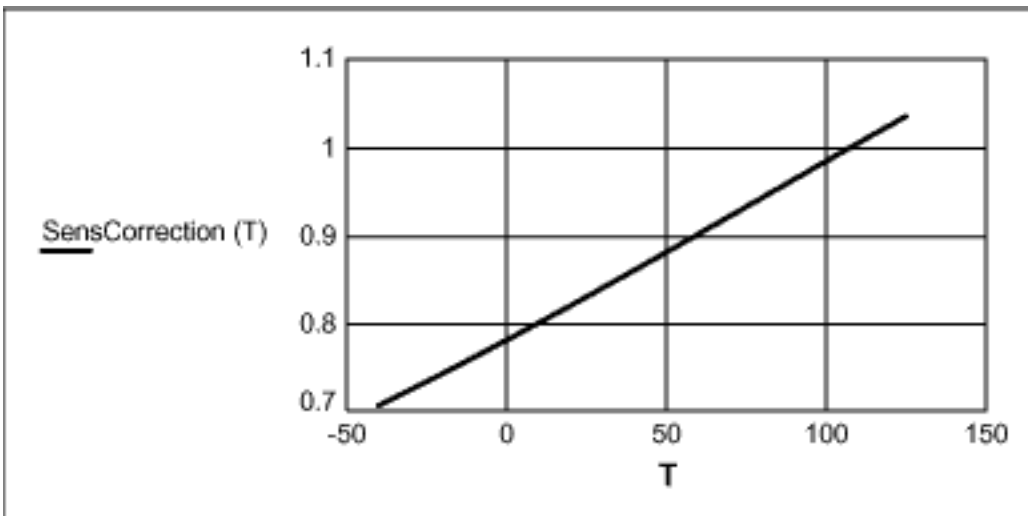
Figure 13. Sensitivity correction function \times temperature ( ^{\circ}\text{C} ).
