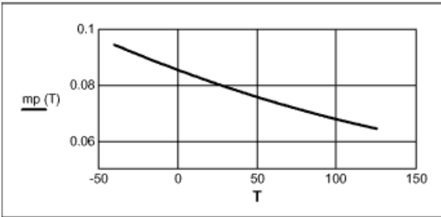
Figure 10. Sensor sensitivity \times Temperature ( ^{\circ}\text{C} ). The pressure nonlinearity and offset correction function can be expressed by:
