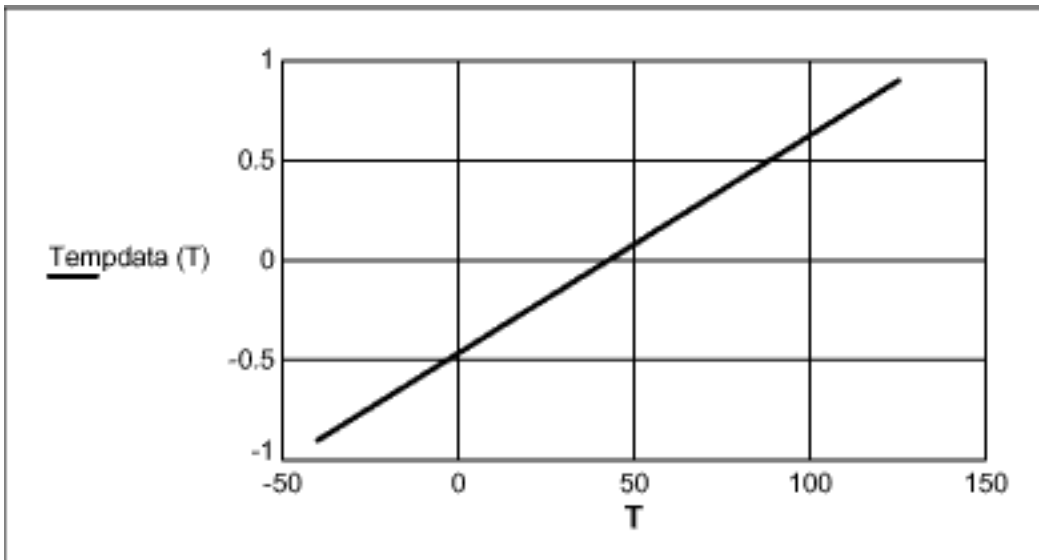
Figure 7. Linear temperature data x temperature.
