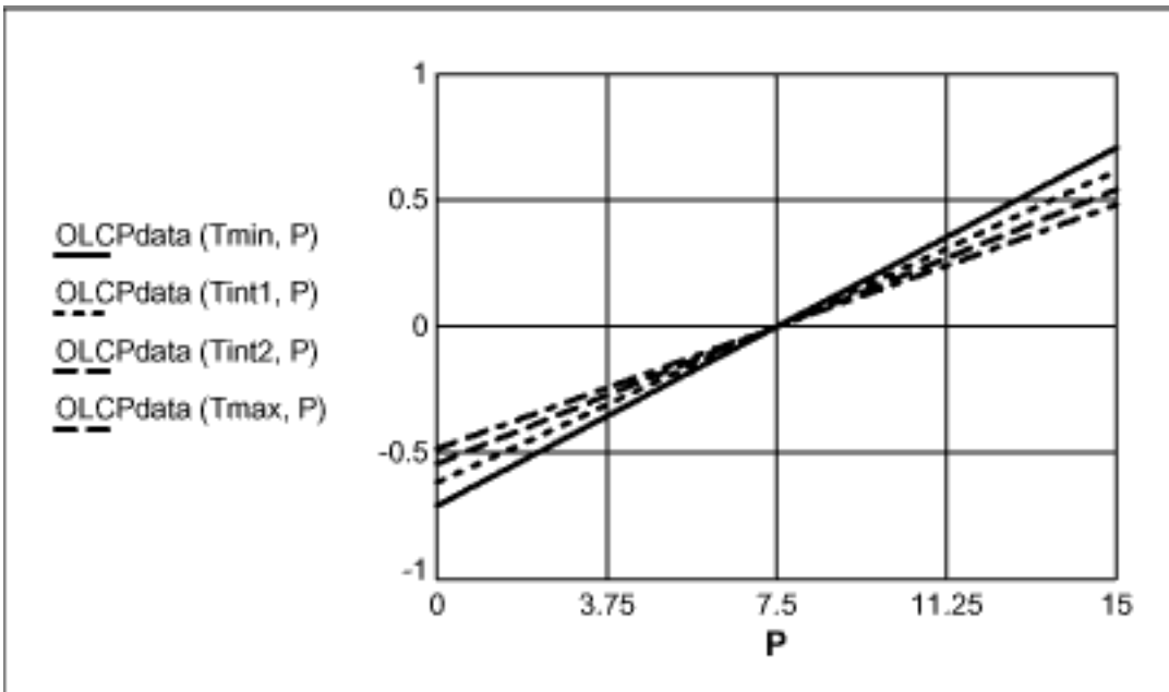
Figure 12. Offset and nonlinearity corrected sensor data x pressure (psi).
