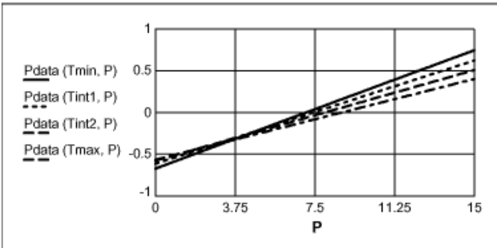
Figure 9. Raw sensor data x pressure (psi).
