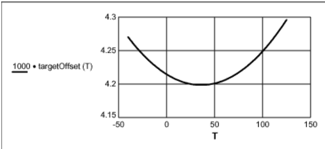
Figure 15. Target DAC input value x Temperature ( ^{\circ}\text{C} ).
