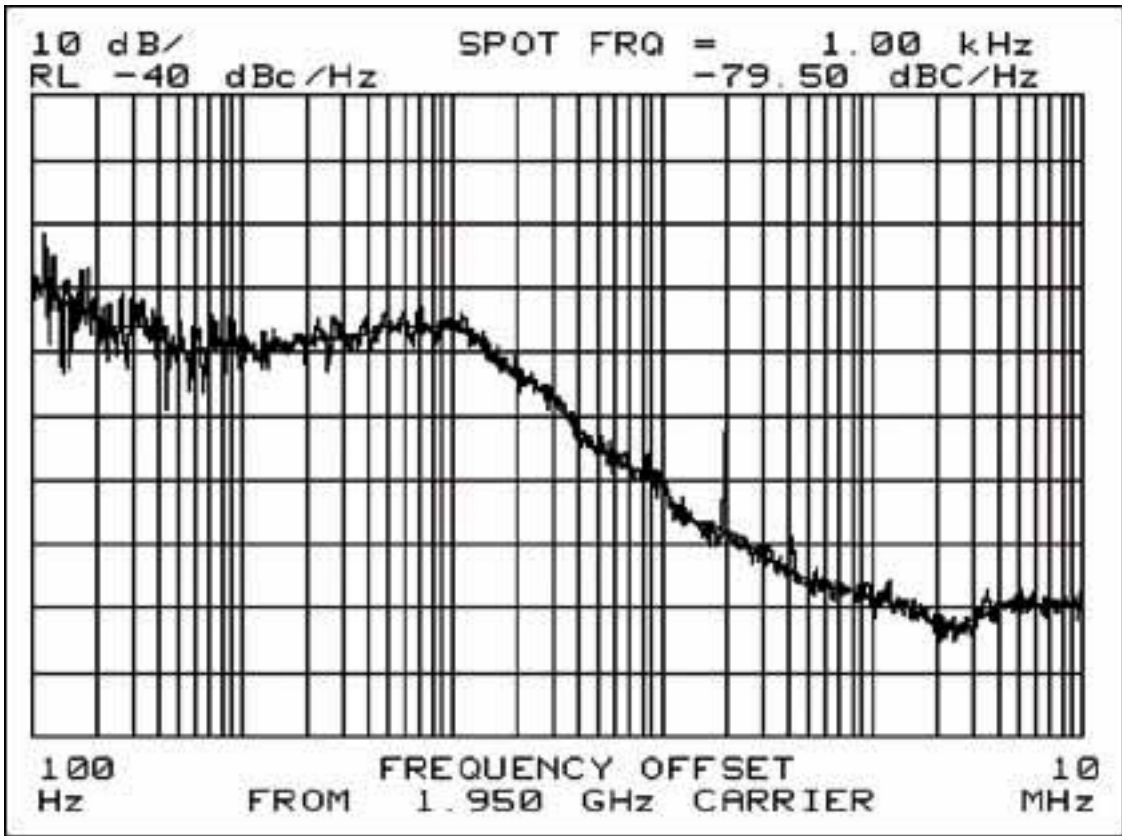
Figure 2. Phase noise plot at 19.2MHz reference crystal.
