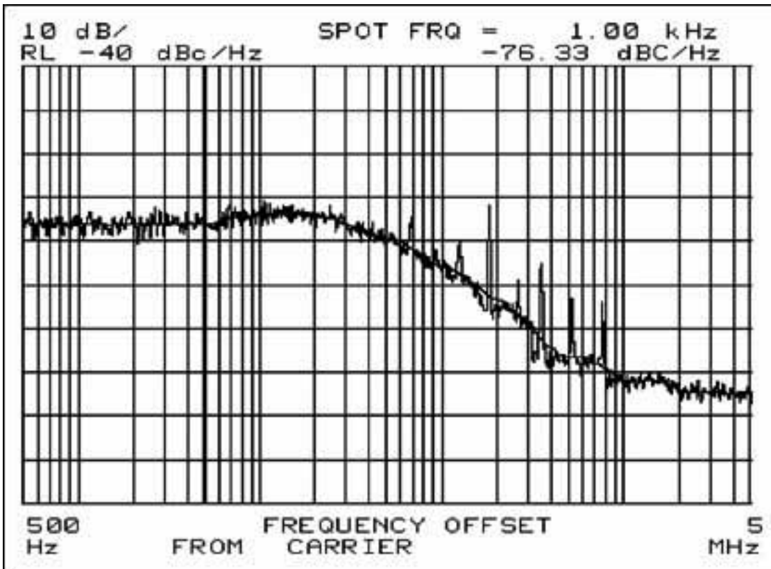
Figure 3. Phase noise plot at 26MHz reference crystal.
