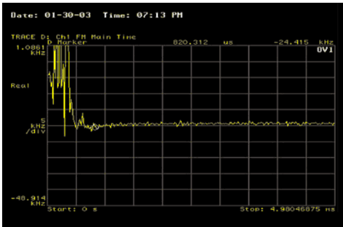
Figure 7. PLL settling time over 60MHz jump at 26MHz crystal.
