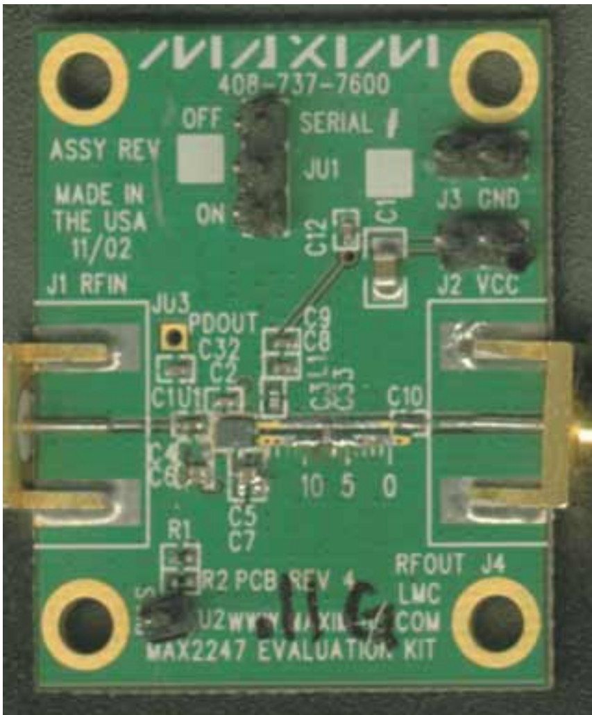
Figure 3. close-up photograph of the component locations.
