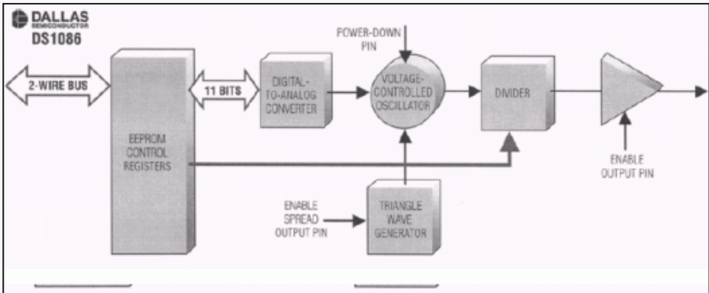
Figure 4. The DS1086 Spread Spectrum EconOscillator.
