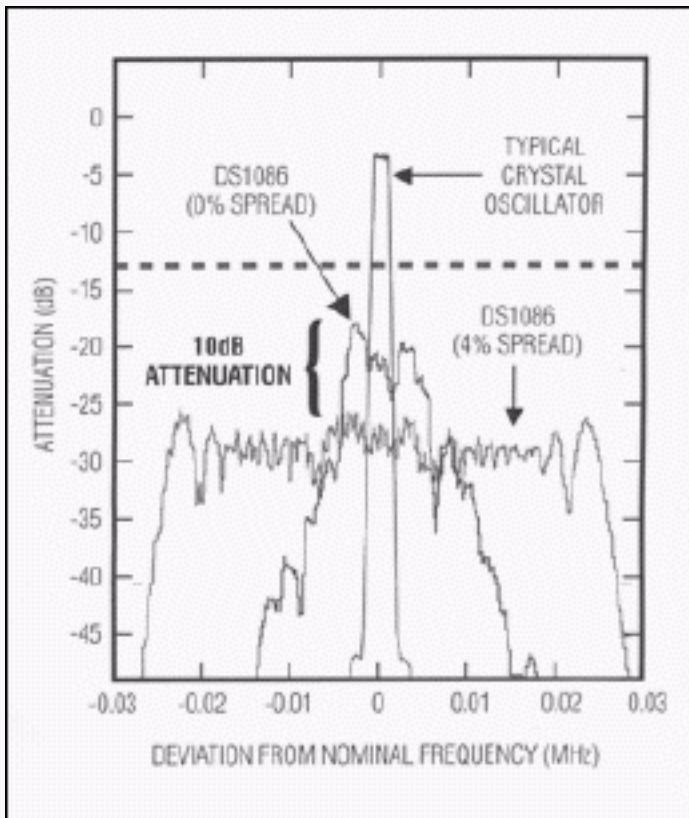
Figure 3. Clock spectrum dither comparison.
