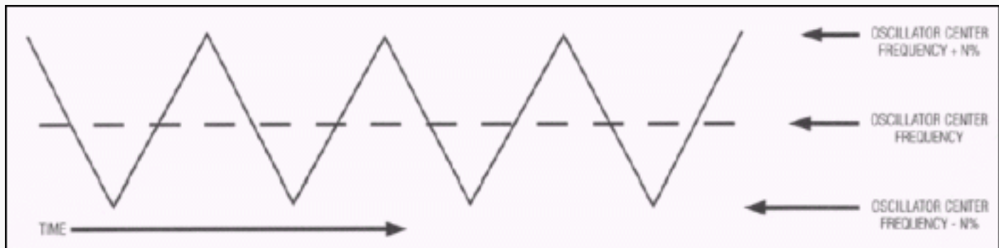
Figure 2. Oscillator dither.
