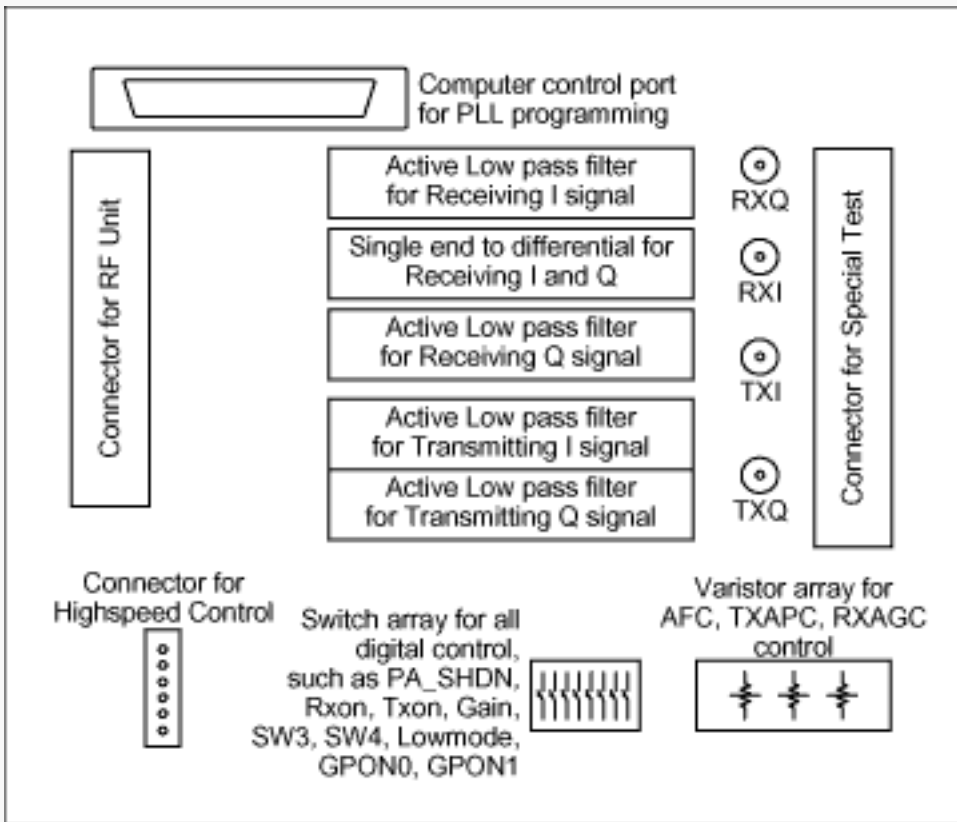
Figure 2. Interface board block diagram.
