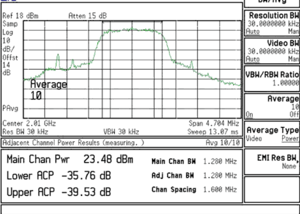
Figure 37. Transmitter intermodulation test 5.
