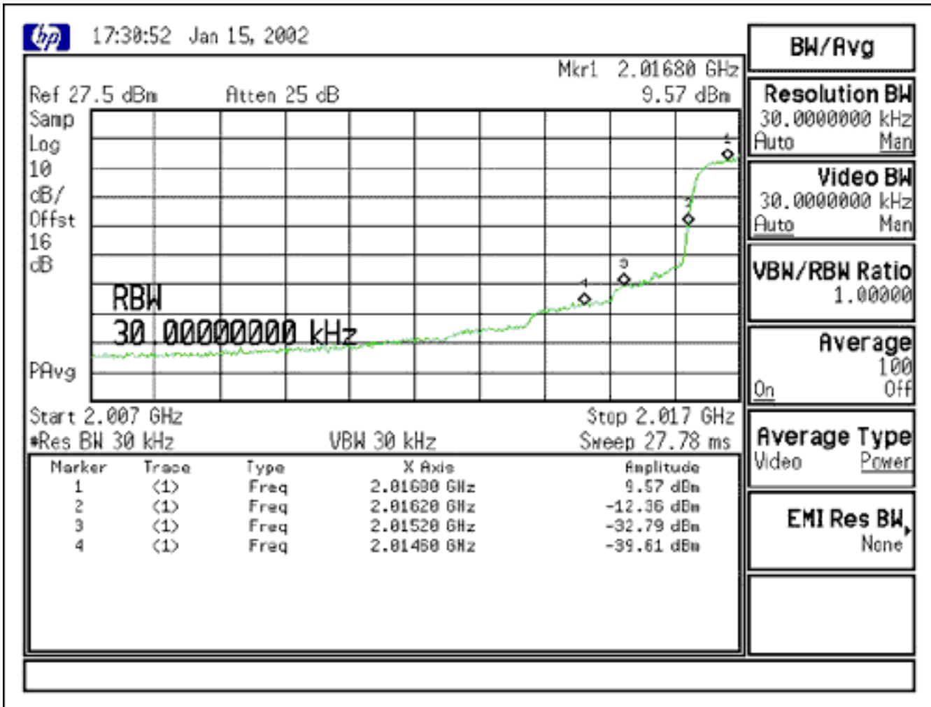
Figure 28. Spectrum emission mask test.
