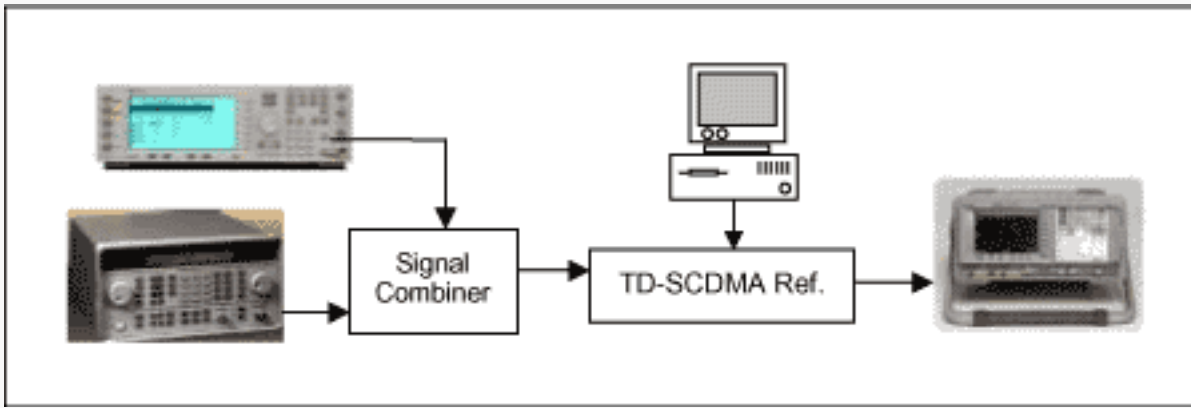
Figure 7. IIP3 test set up.
