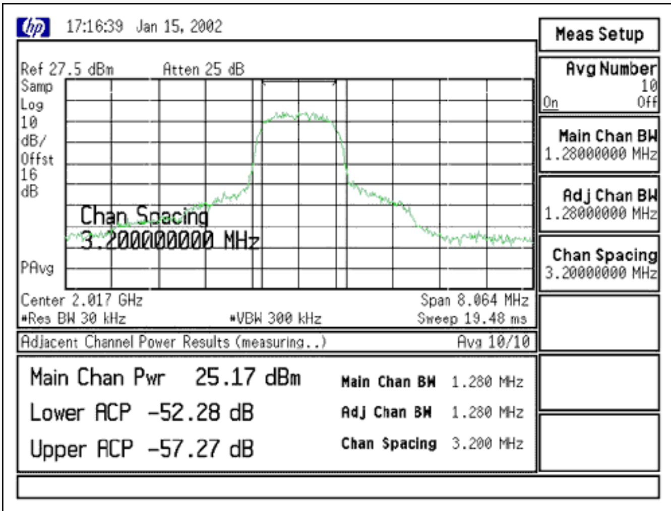
Figure 31. ALT channel ACLR test.
