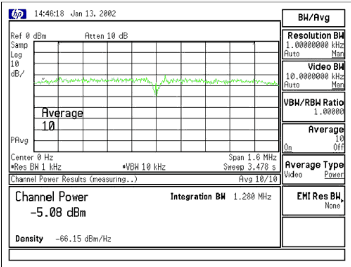
Figure 18. Low-side intermodulation test.
