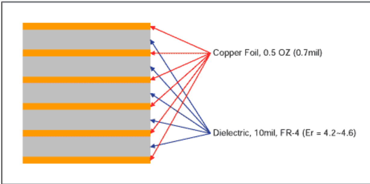
Figure 39. PCB layer stackup uses FR-4 dielectric.
