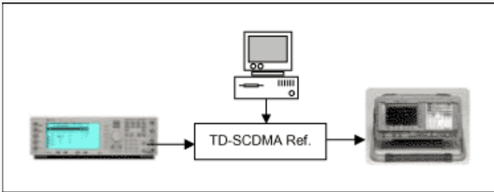
Figure 8. IIP2 test.
