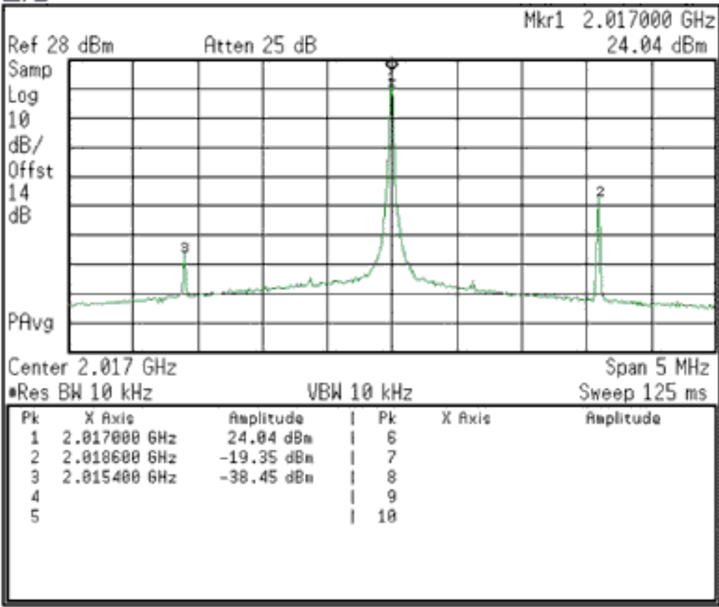
Figure 33. Transmitter intermodulation test 1.
