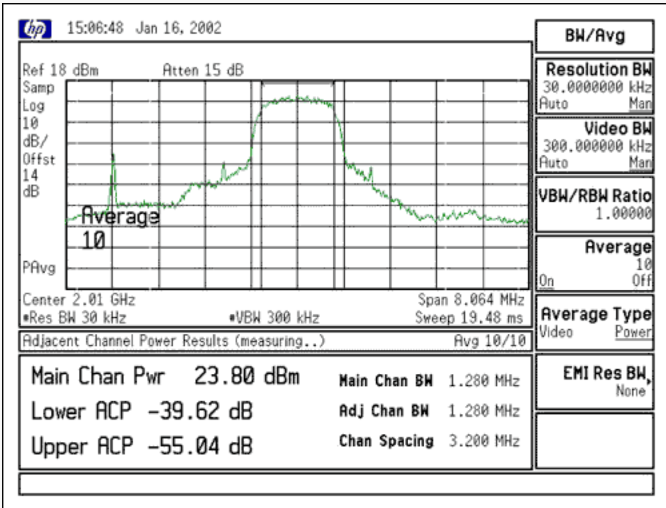
Figure 38. Transmitter intermodulation test 6.
