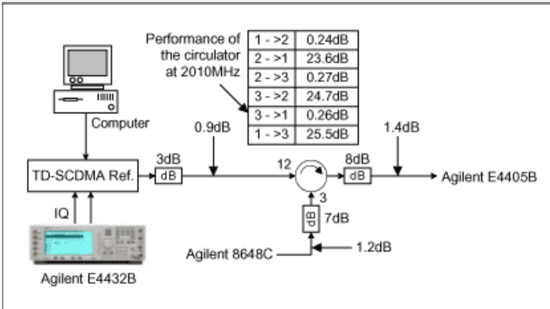
Figure 32. Transmitter intermodulation test.
