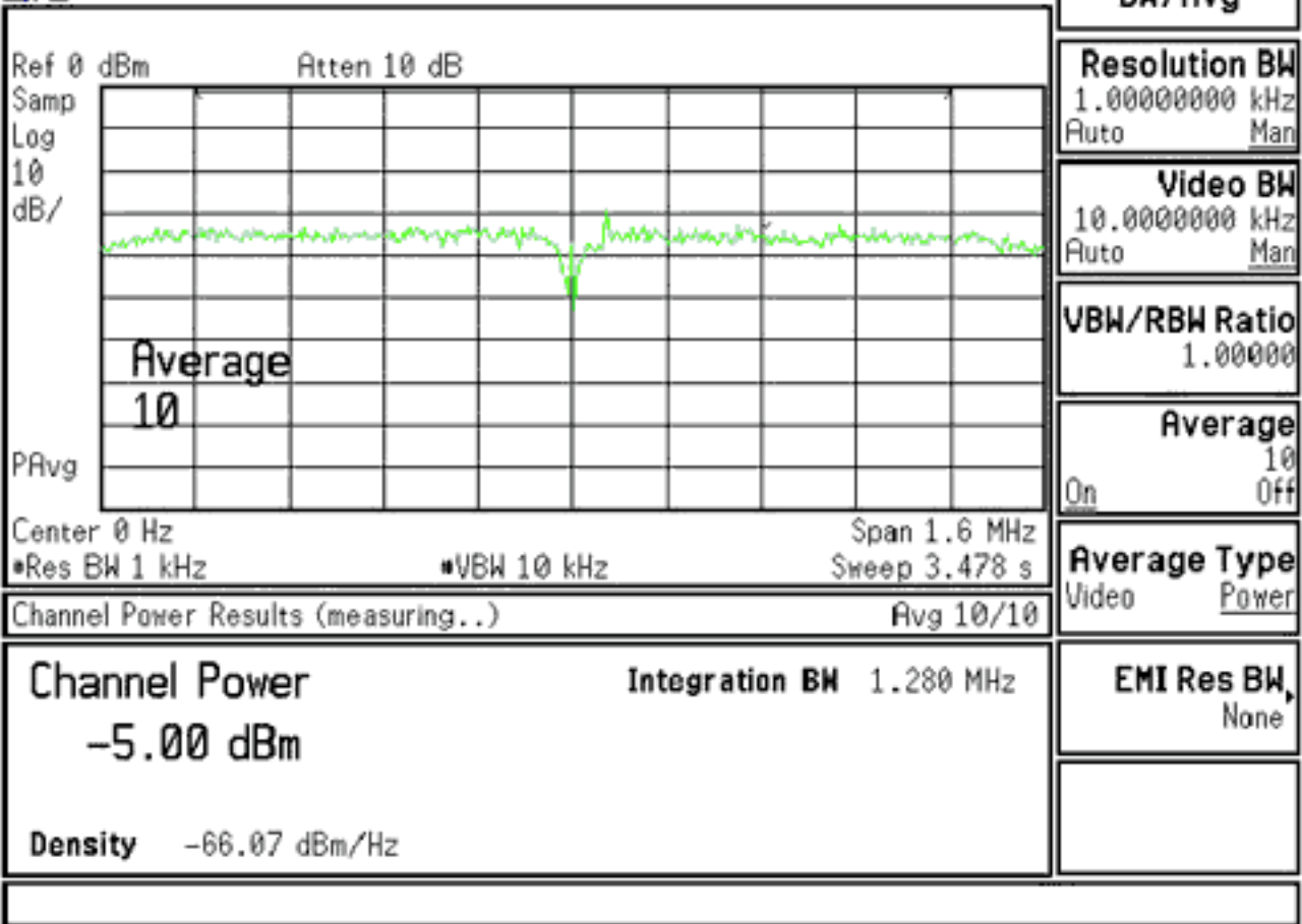
Figure 17. High-side intermodulation test.
