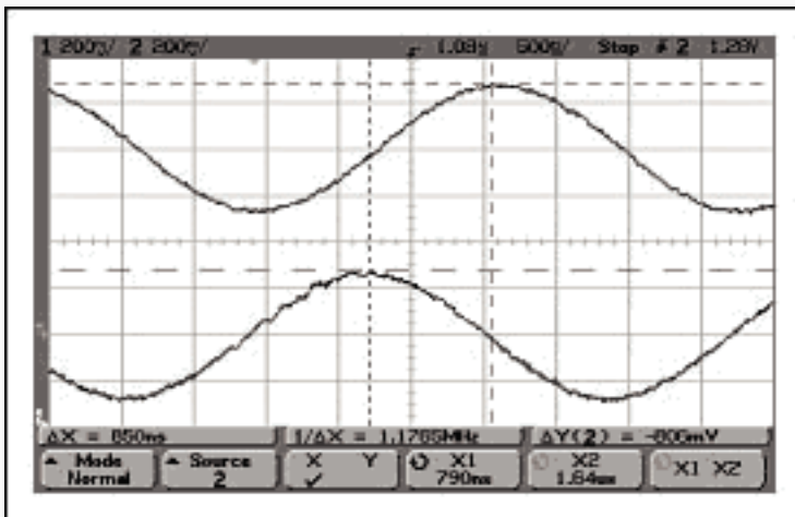
Figure 22. Before LPF phase imbalance test @300kHz.
