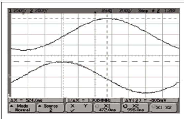
Figure 23. Before LPF phase imbalance test @500kHz.
