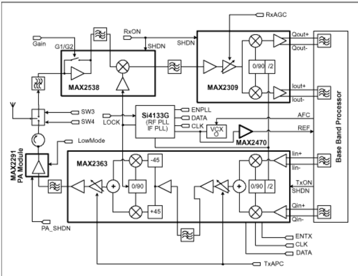
Figure 1. TD-SCDMA RF transceiver block diagram.
