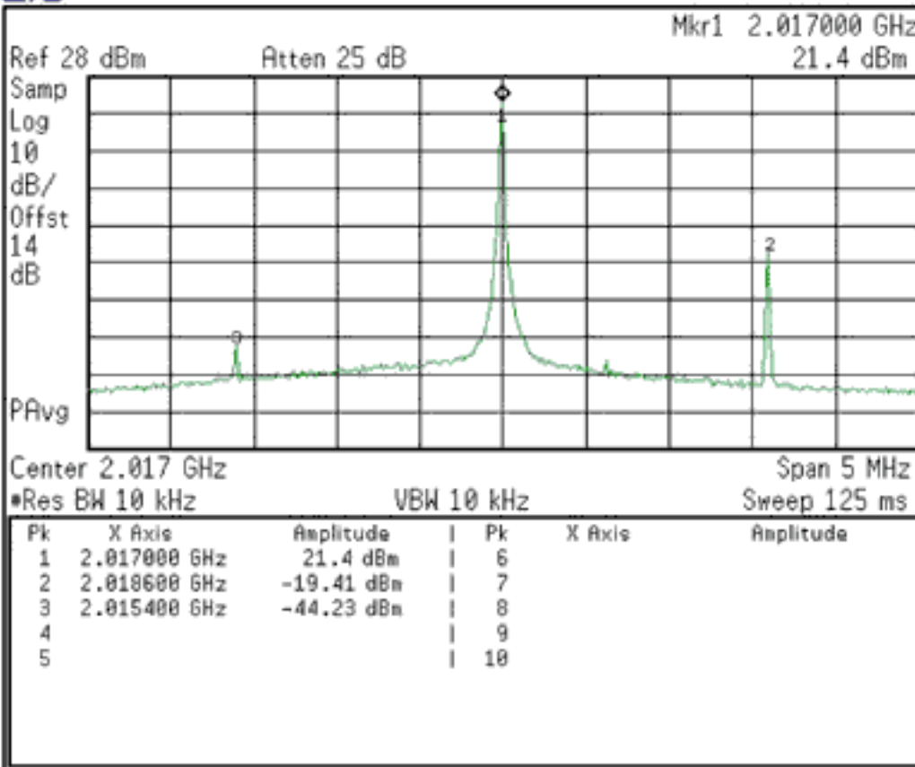
Figure 34. Transmitter intermodulation test 3.
