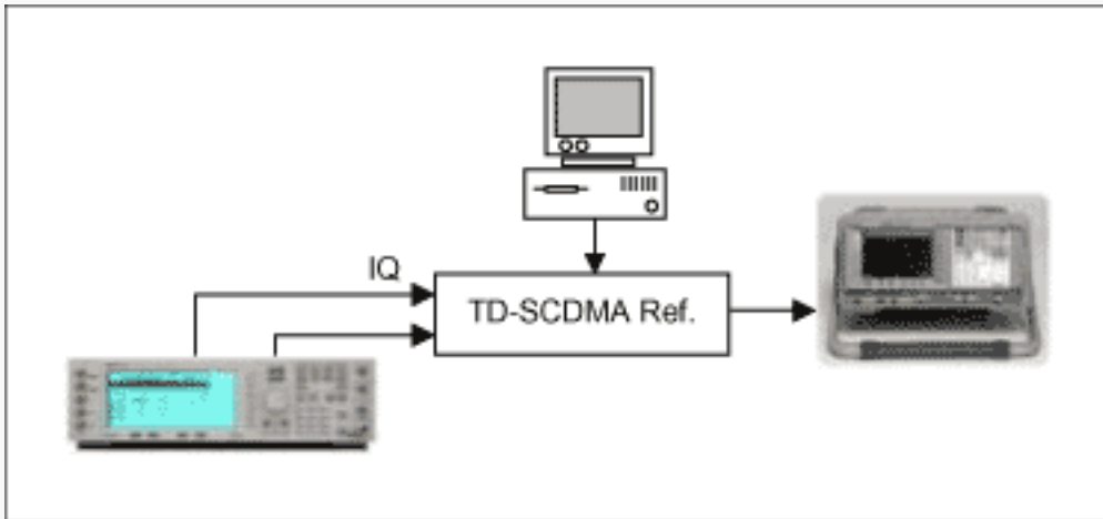
Figure 24. Output power test setup.
