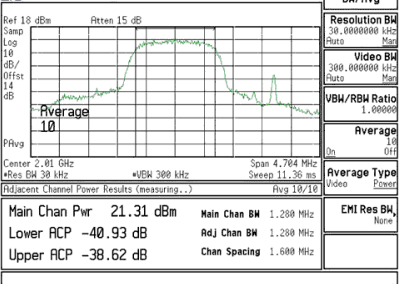
Figure 36. Transmitter intermodulation test 2.
