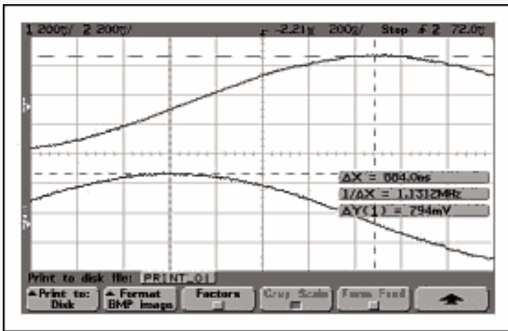
Figure 21. After LPF phase imbalance test @300kHz.
