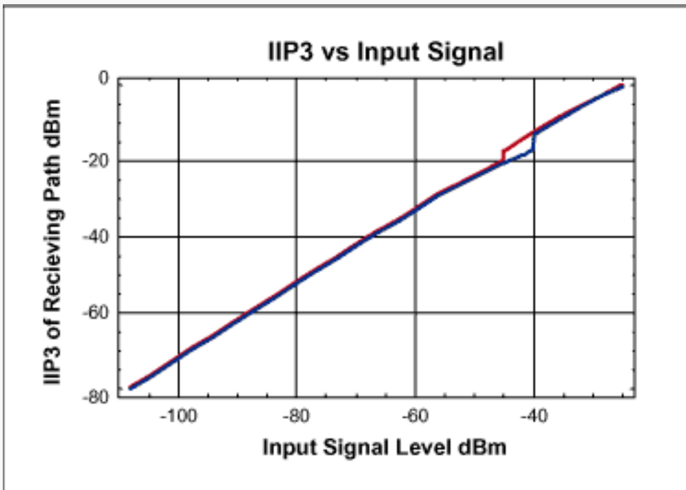
Figure 14. Cascade IIP3 vs. input signal strength.
