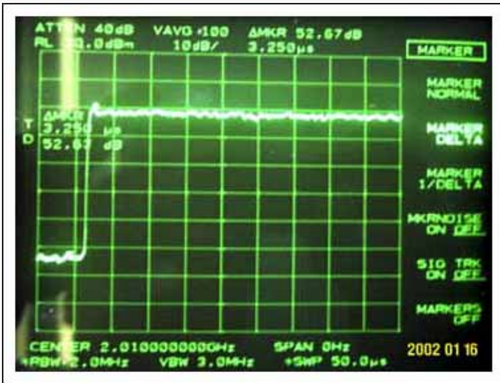
Figure 26. Transmitter on time test screen.
