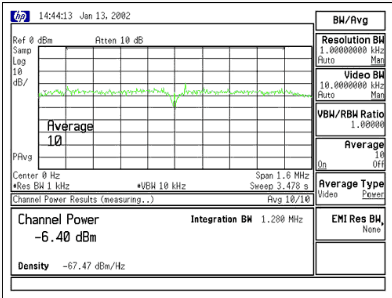
Figure 16. Baseband noise floor with No RF input.
