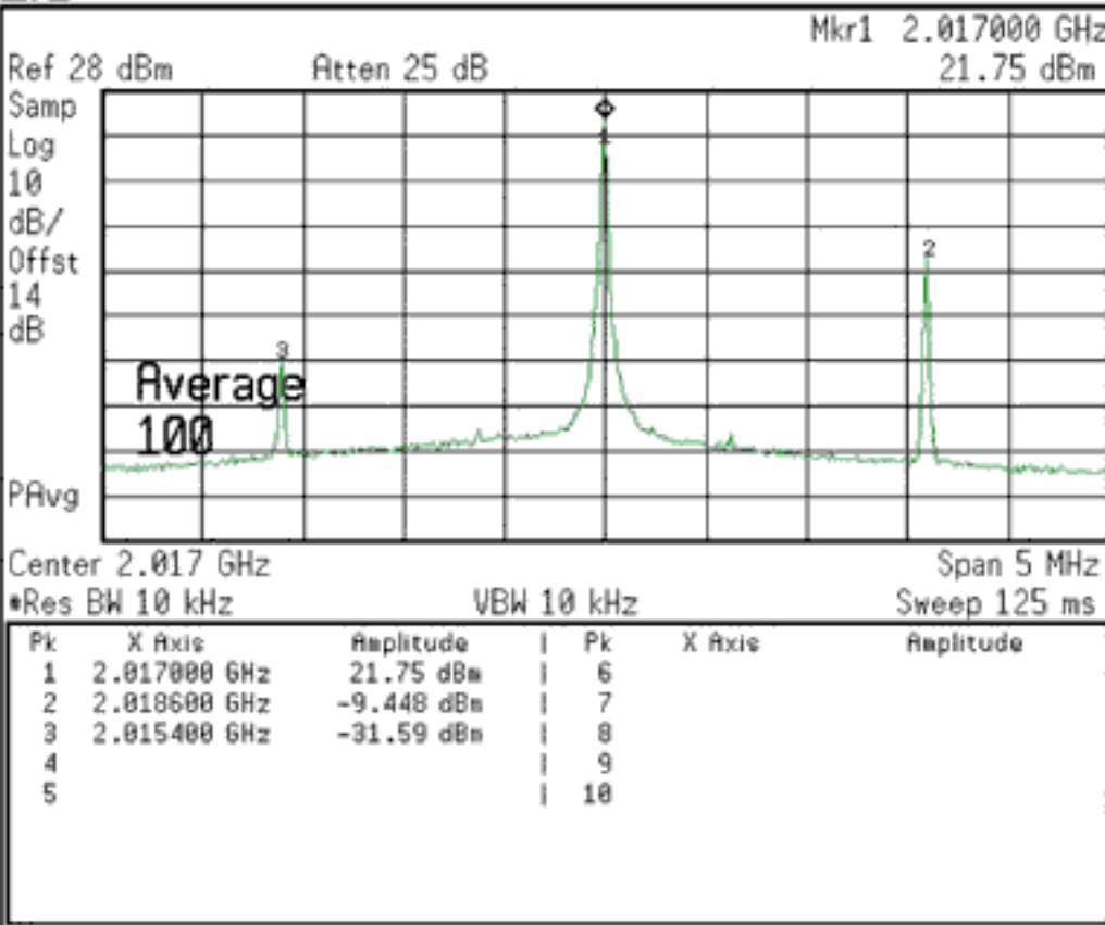
Figure 35. Transmitter intermodulation test 4.
