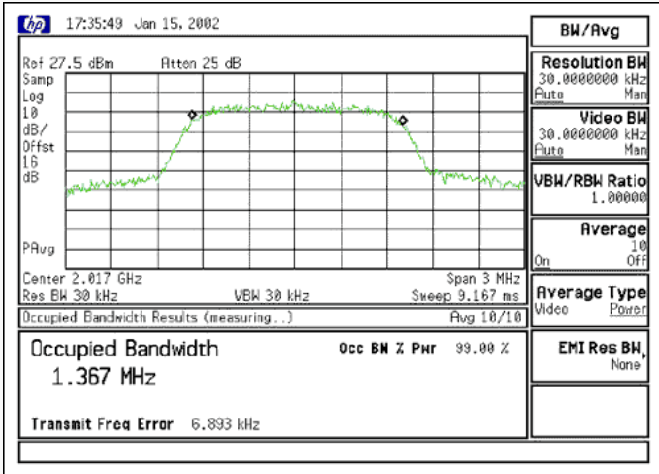
Figure 27. Occupied bandwidth test.
