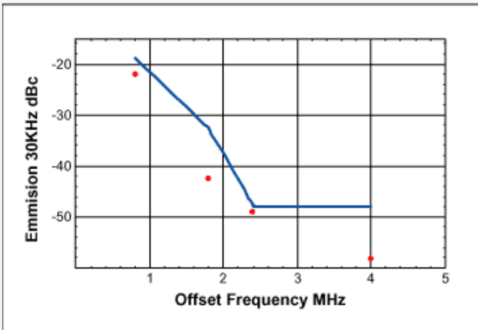
Figure 29. Spectrum emission mask test result.
