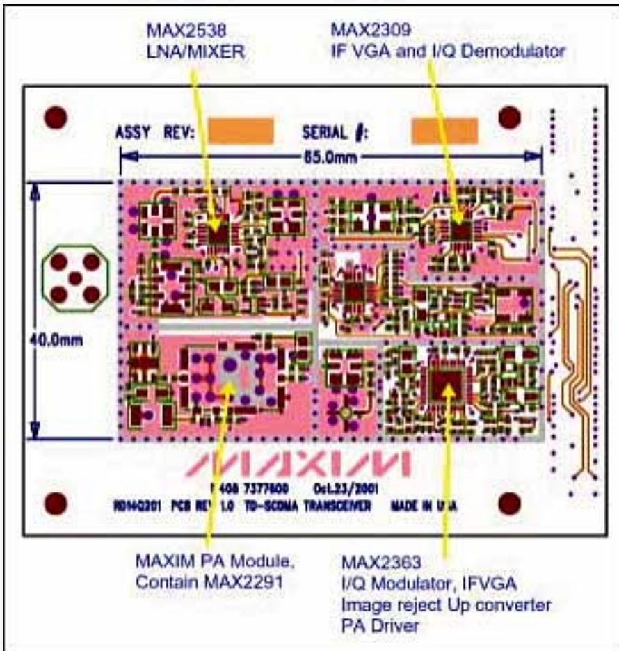
Figure 4. TD-SCDMA transceiver dimensions.
