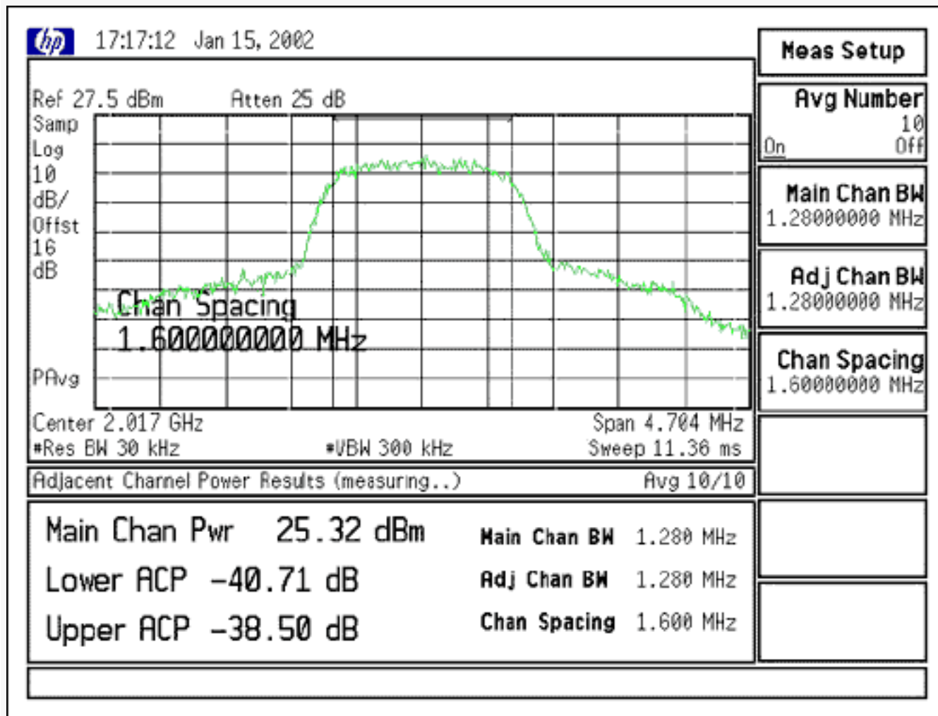
Figure 30. Adjacent channel ACLR test.
