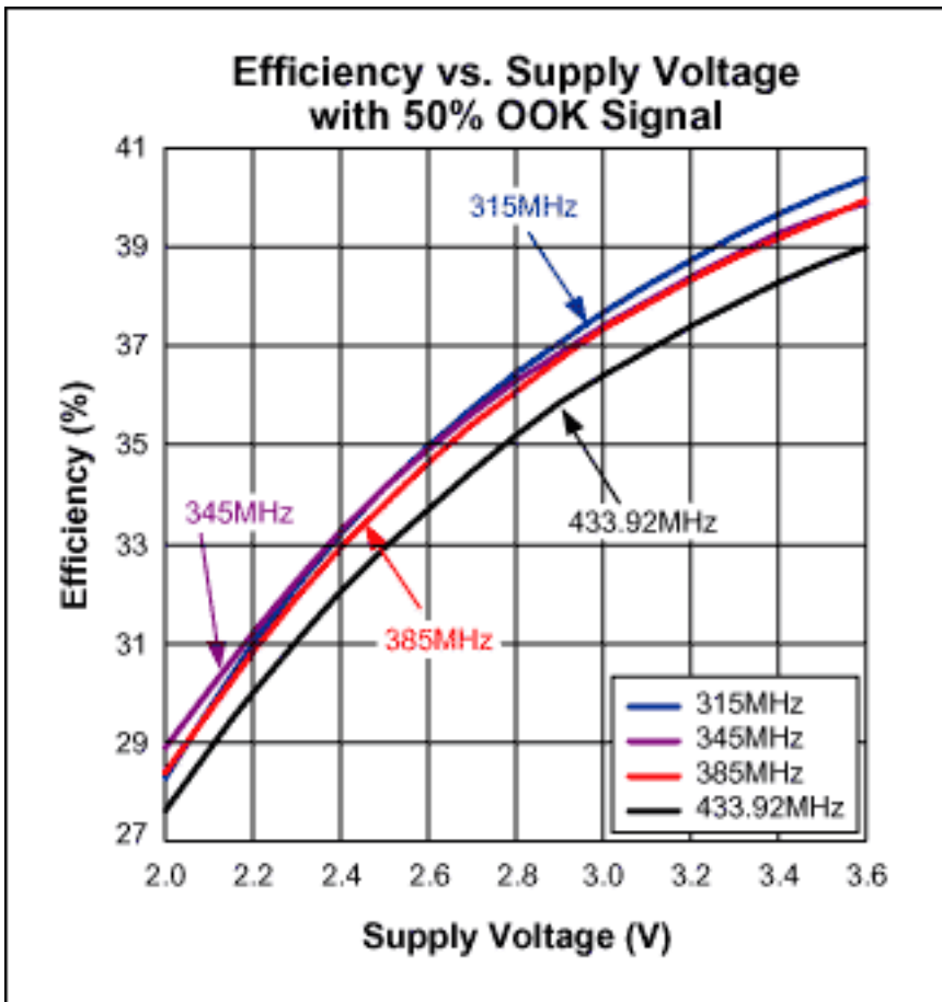
Figure 3. Efficiency vs. supply voltage with 50% OOK signal.
