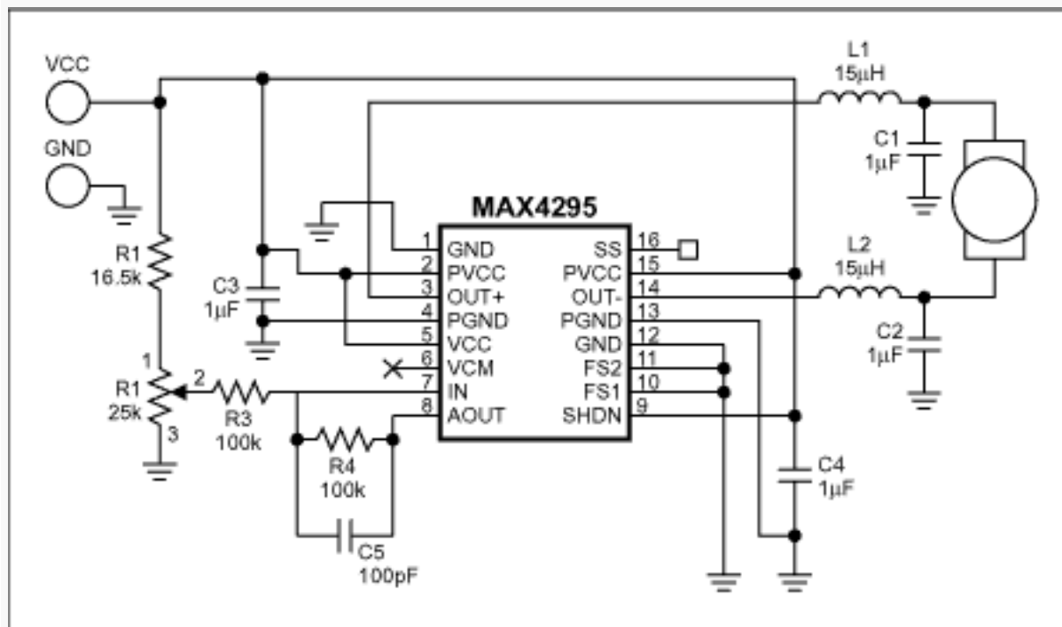
Figure 1. A class D audio amplifier (U1) helps implement this simple motor-speed controller.
