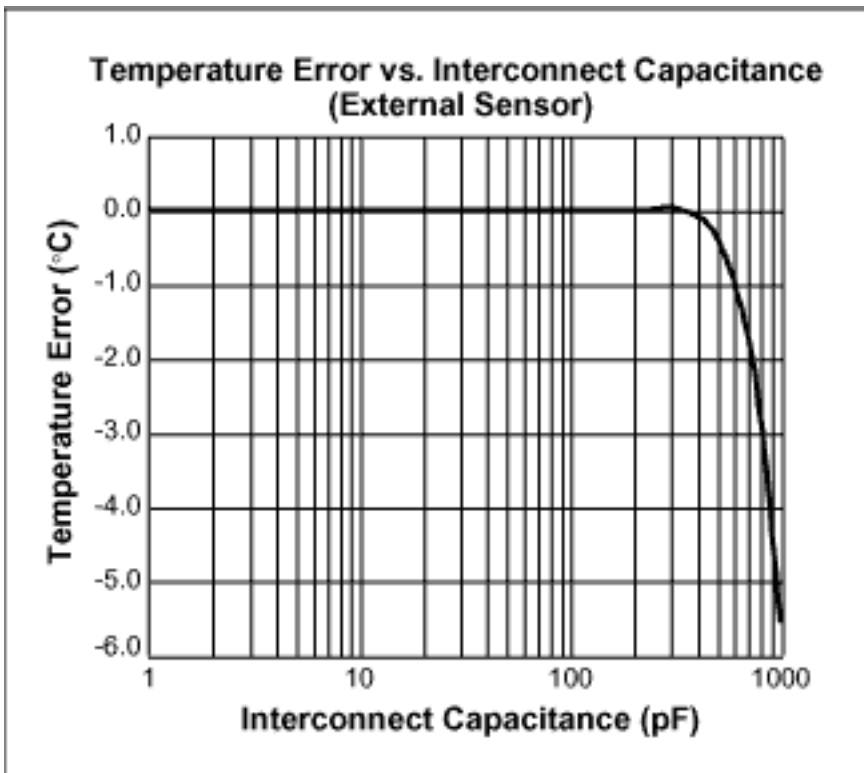
Figure 4. Effect of external sensor capacitance.
