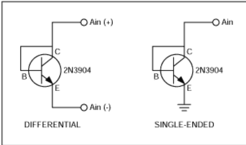
Figure 1. Connecting differential and single-ended temperature sensors.
