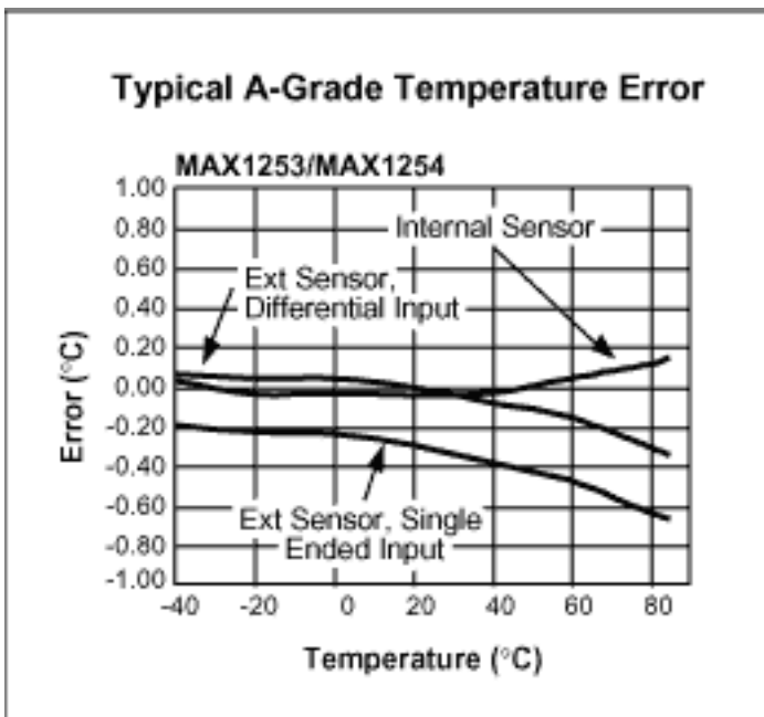
Figure 2. Typical A-grade temperature error.
