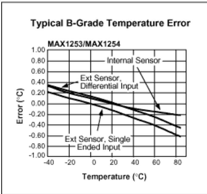
Figure 3. Typical B-grade temperature error.
