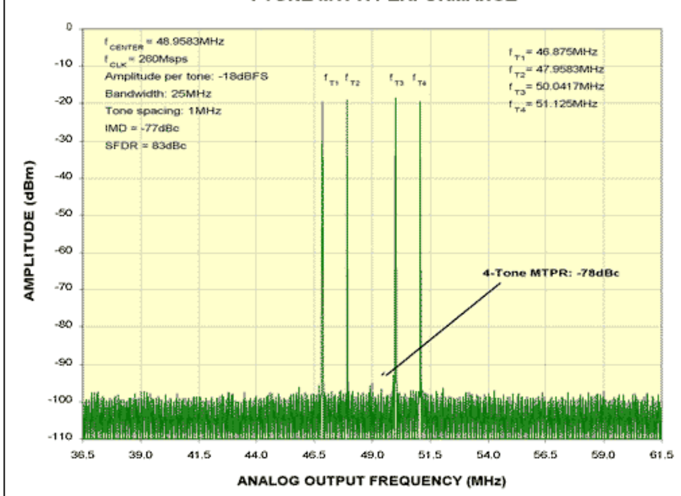
Figure 2. This spectrum plot depicts the four-tone MTPR performance at f_{\text{CENTER}} = 48.9583\text{MHz} and f_{\text{CLK}} = 260\text{MHz} of the MAX5195, which meets the most critical GSM/EDGE specifications.
