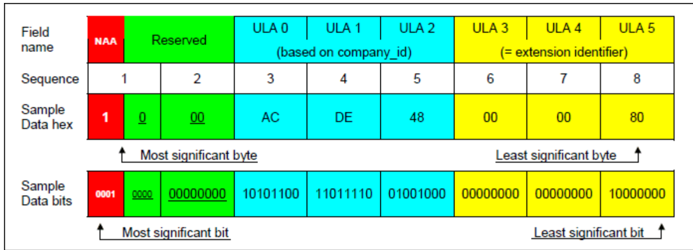
Figure 3. FC-PH IEEE 48-bit identifier format.
