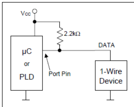
Figure 10. Minimal 1-Wire interface.
