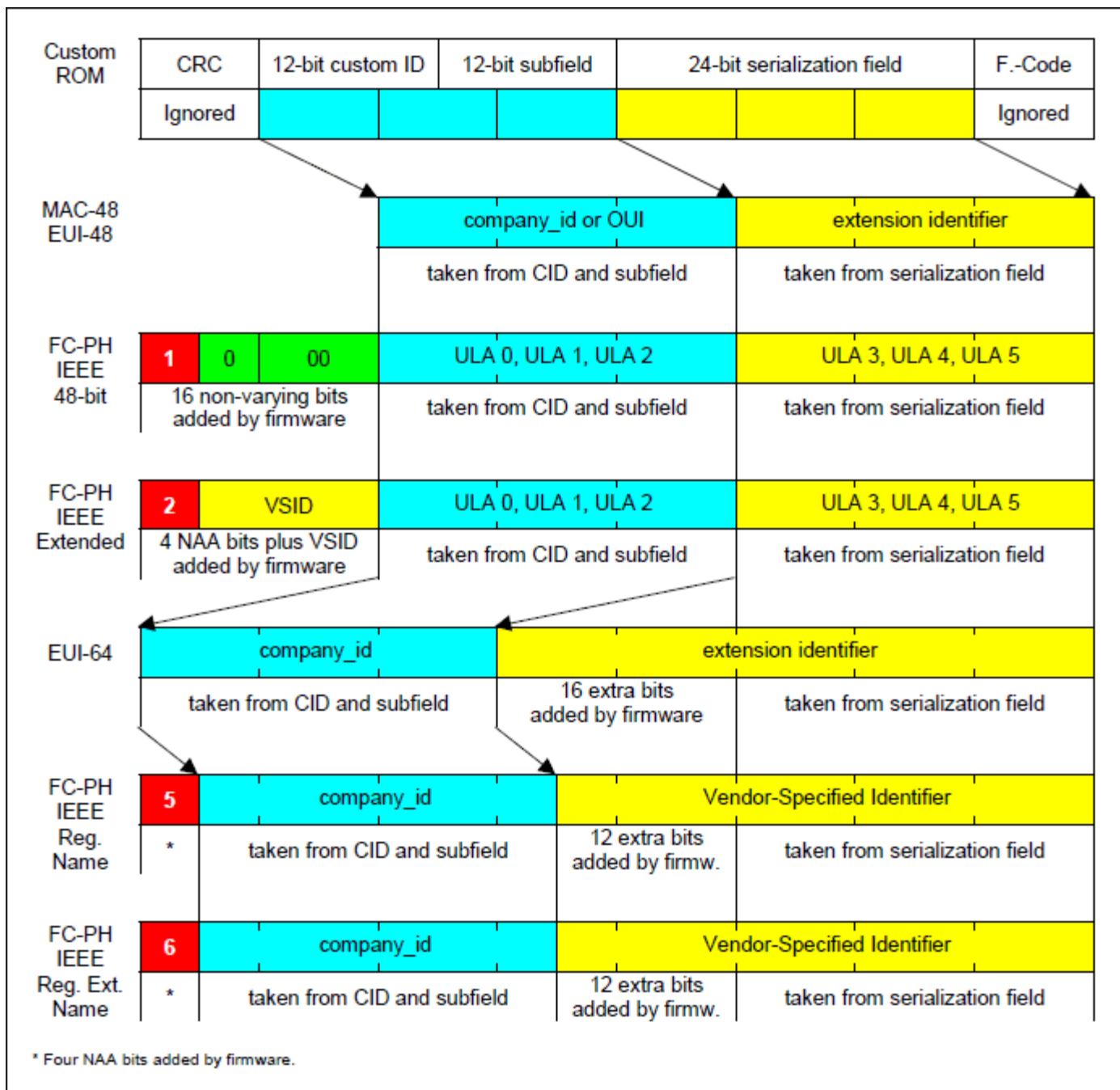
Figure 9. Creating identifiers from custom ROM parts.
