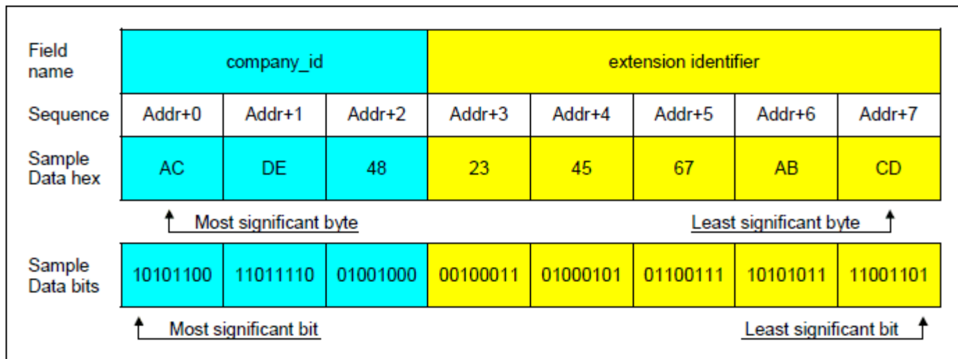
Figure 2. EUI-64 global identifier format.
