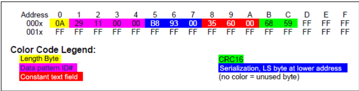
Figure 11. DS2502-E48 ethernet address.
