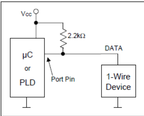
Figure 11. Minimal 1-Wire interface.
