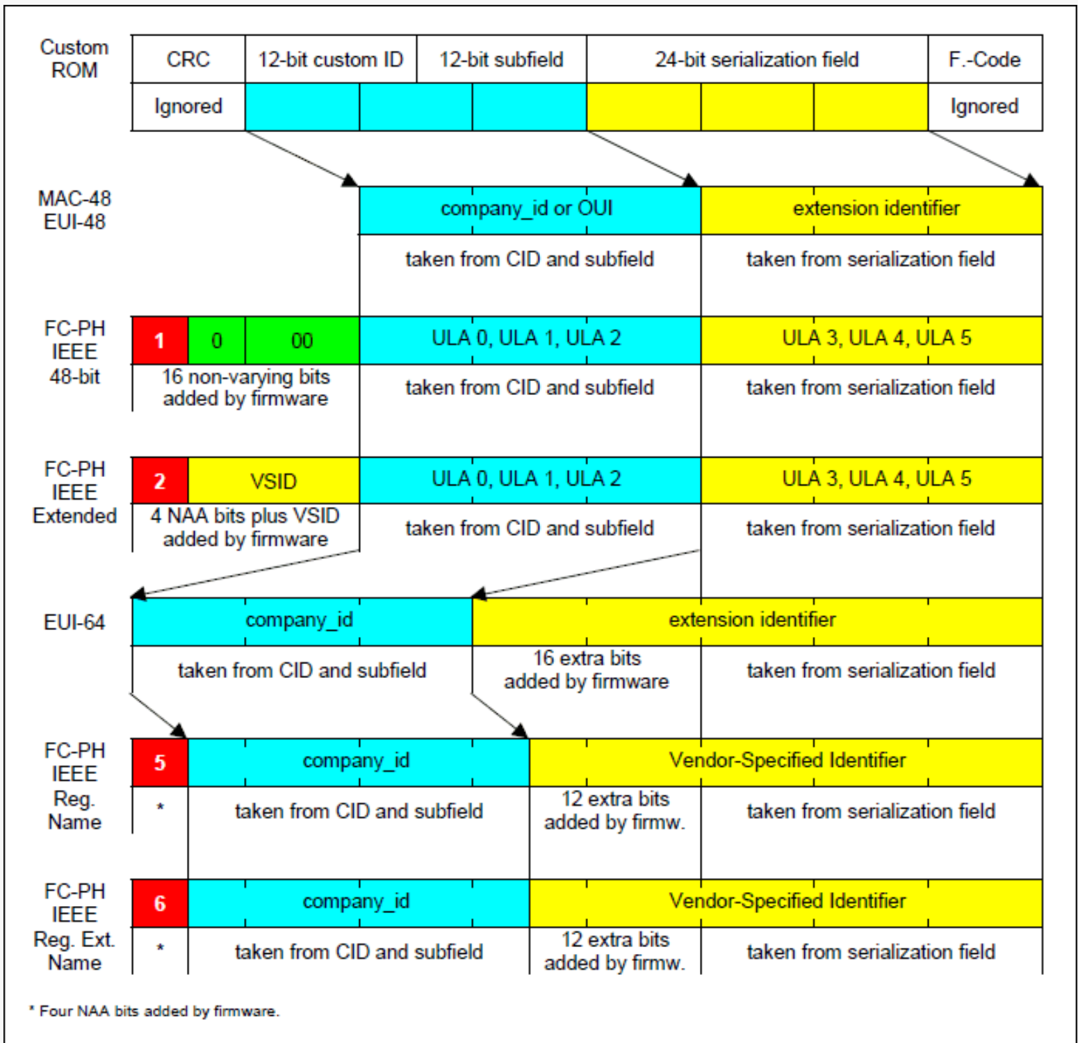
Figure 9. Creating identifiers from custom ROM parts.
