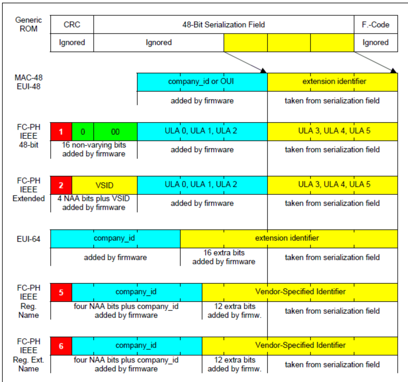
Figure 7. Creating identifiers from generic parts.
