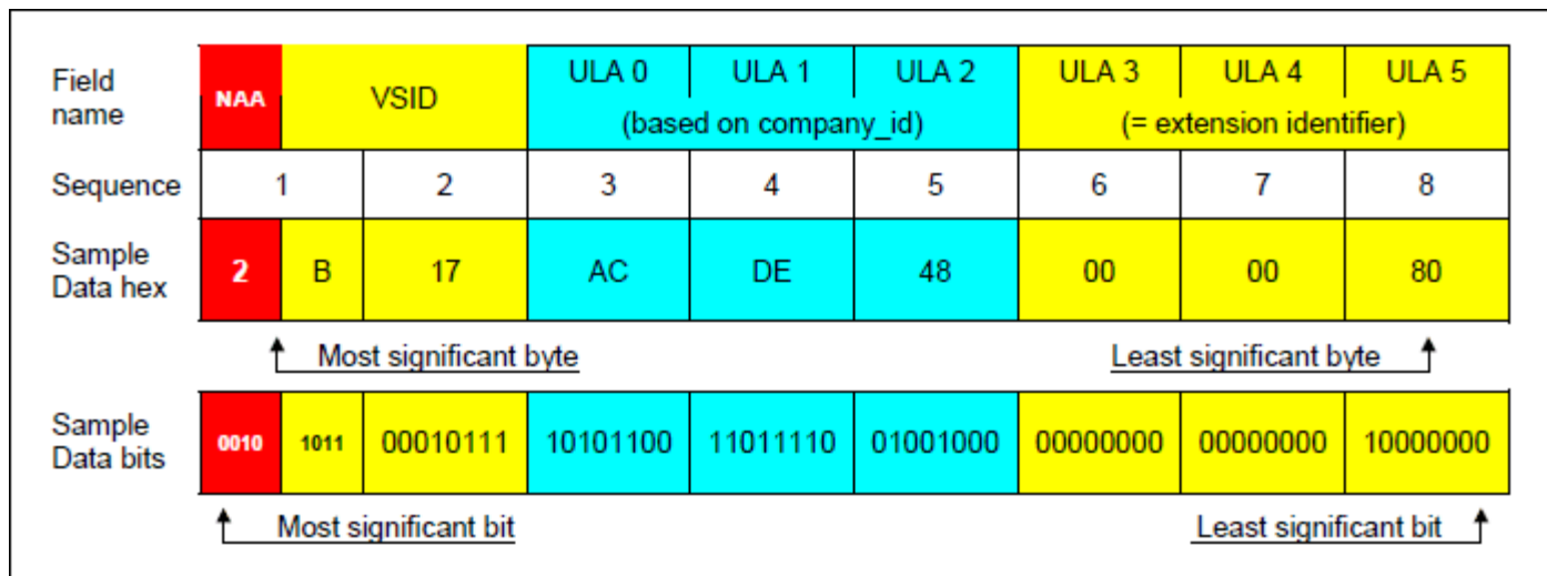
Figure 4. FC-PH IEEE extended identifier format.
