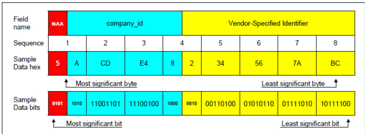
Figure 5. FC-PH IEEE registered name format.
