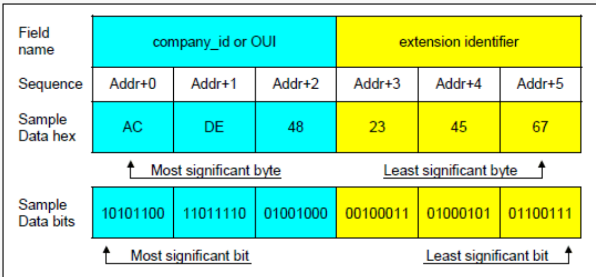
Figure 1. MAC-48 identifier/EUI-48 global identifier format.
