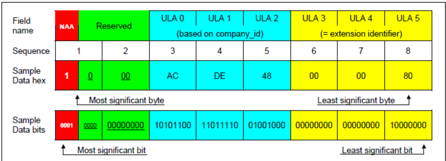
Figure 3. FC-PH IEEE 48-bit identifier format.
