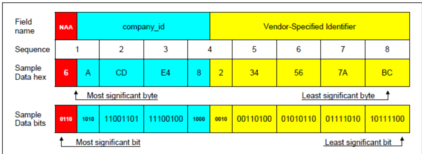
Figure 6. FC-PH IEEE registered extended name format (first block).
