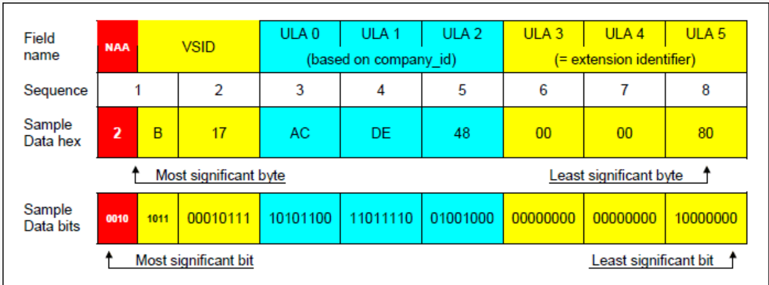
Figure 4. FC-PH IEEE extended identifier format.
