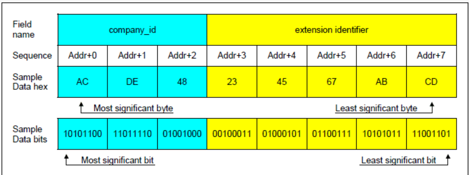
Figure 2. EUI-64 global identifier format.
