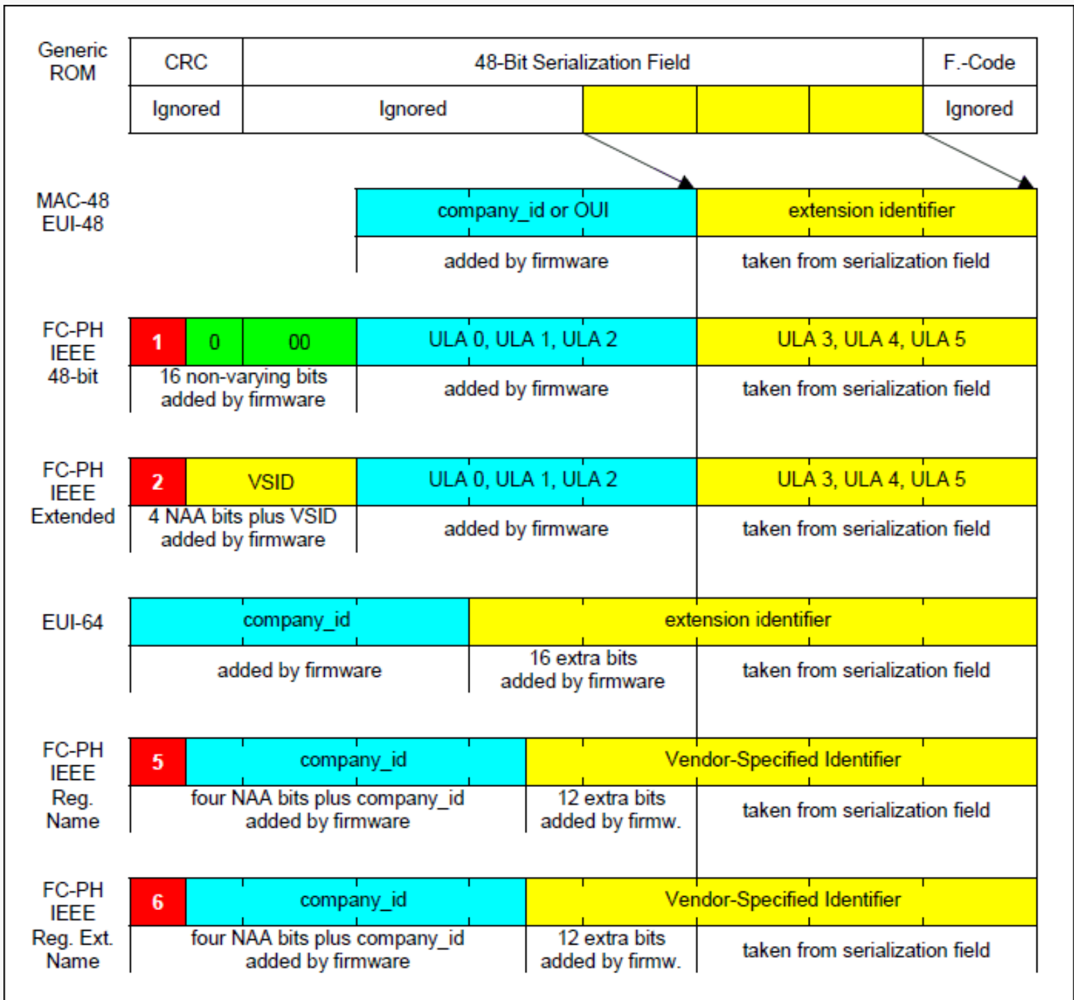
Figure 7. Creating identifiers from generic parts.
