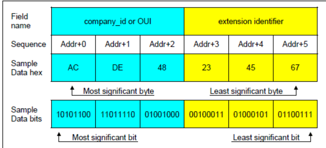
Figure 1. MAC-48 identifier/EUI-48 global identifier format.
