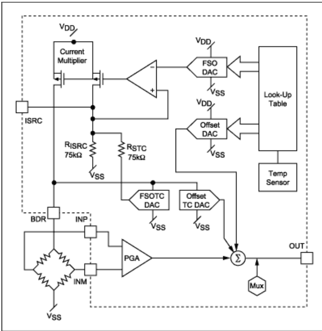
Figure 8. MAX1452 sensor conditioner I.C.
