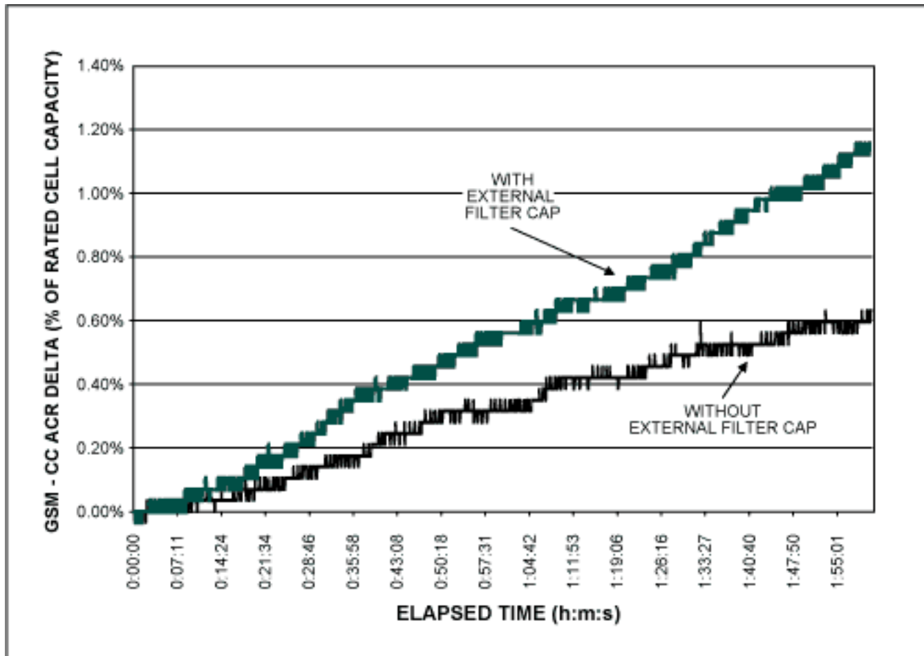
Figure 4. The difference in measured ACR between one GSM and one constant current discharge illustrates the deviation at the endpoints.
