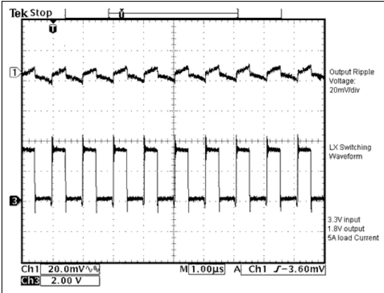
Figure 2. Output ripple voltage and LX switching waveforms.
