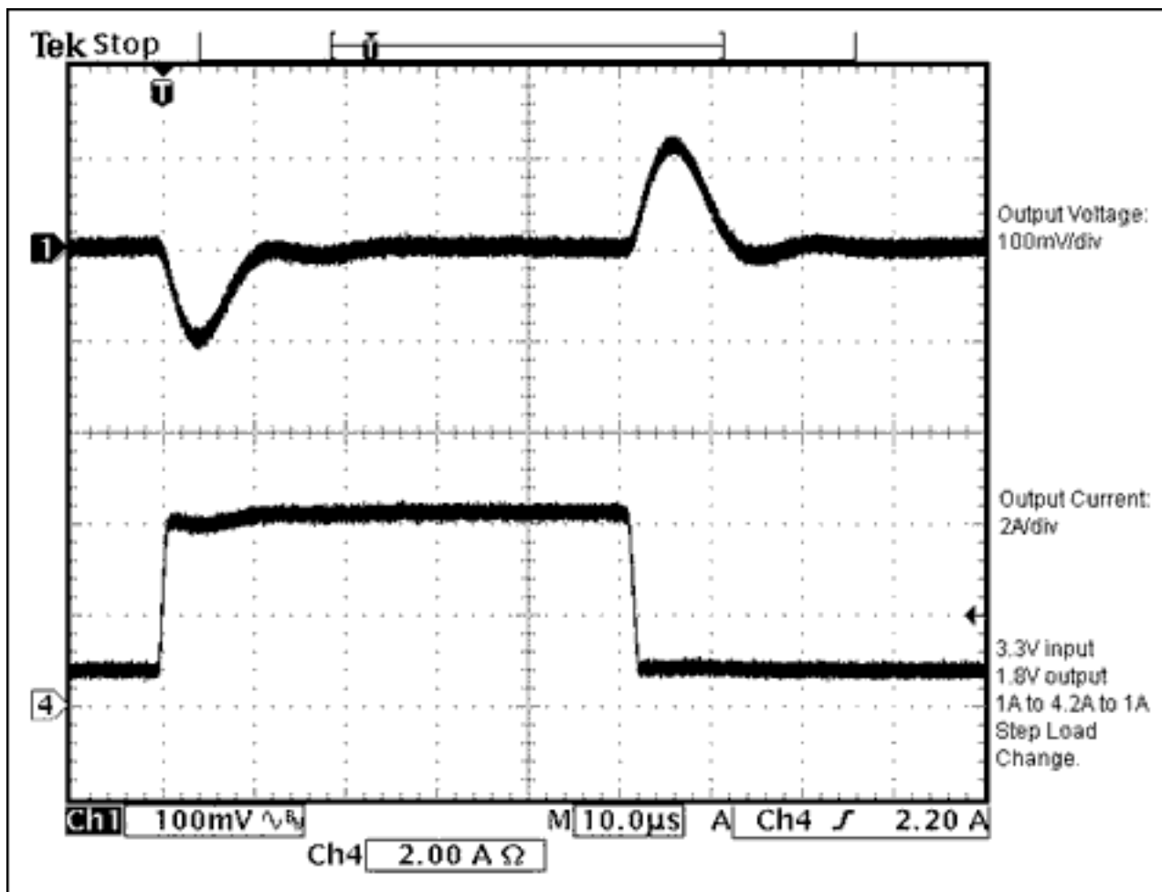
Figure 3. Step load transient response: output current from 1A to 4.2A back to 1A. The output voltage back to regulation within 10µs for 50% step load change.
