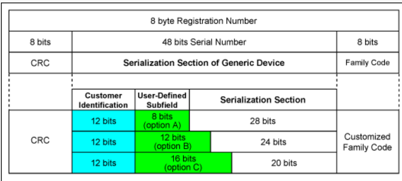
Figure 1. Generic and Customized ROM Registration Number
