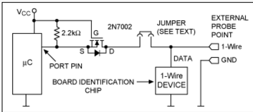
Figure 2. Dual-Read Mode Interface
