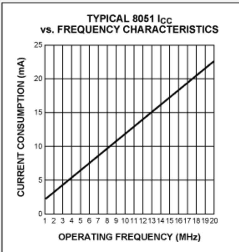
Figure 1. Typical power curve for generic 8051 microcontroller.
