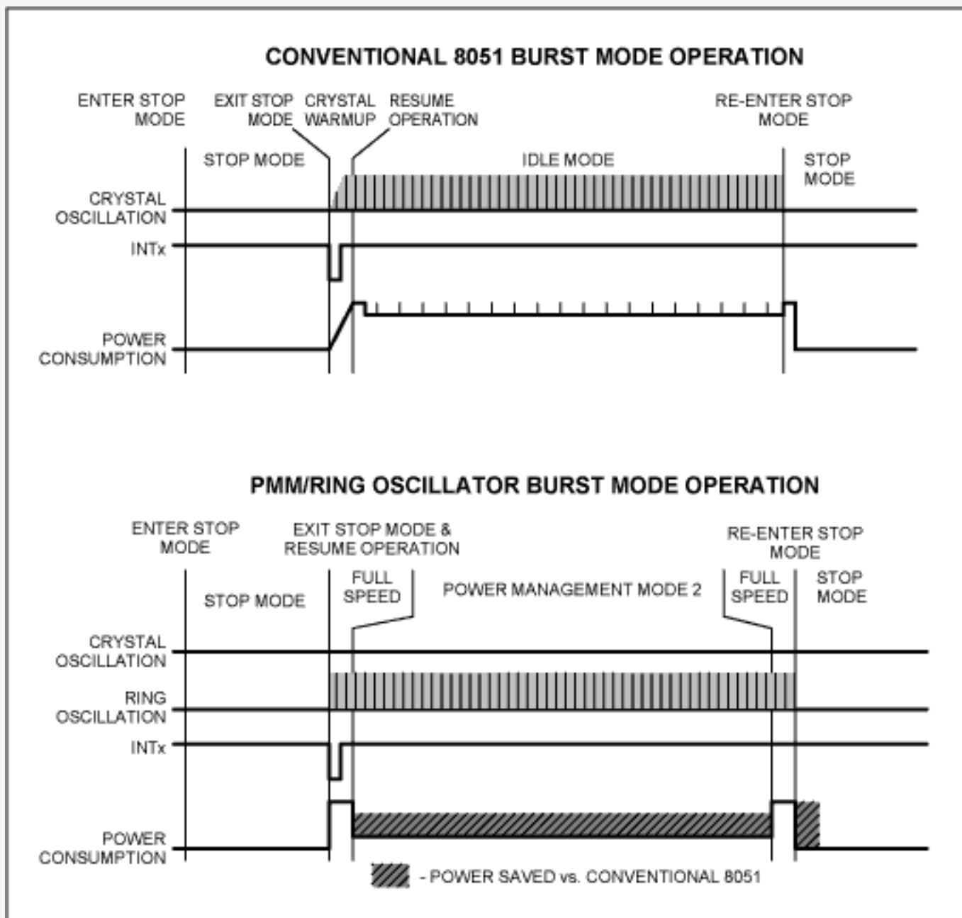
Figure 8. Implementing an 8051 "Hurry Up and Wait" scheme.
