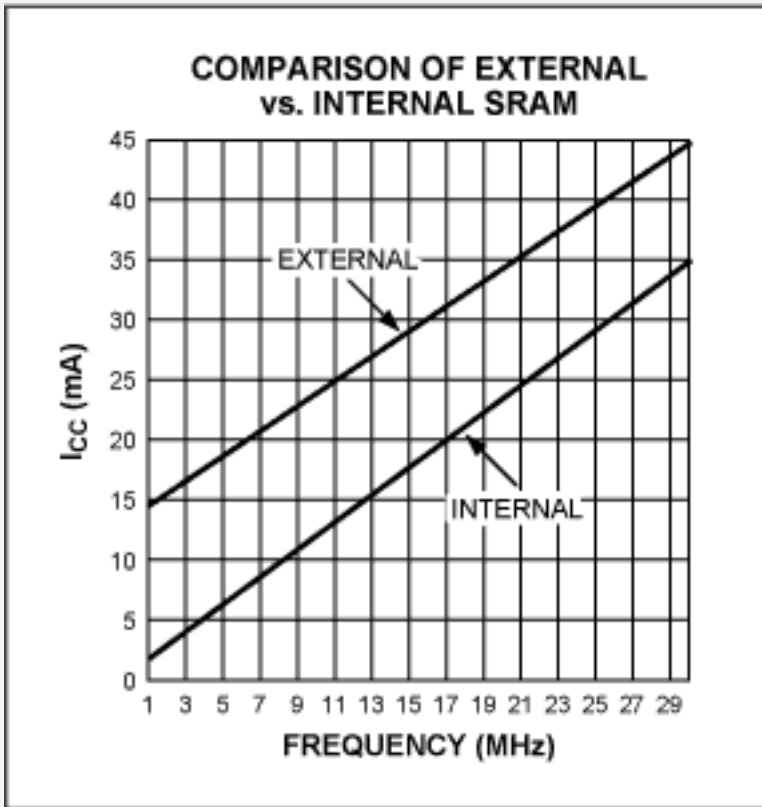
Figure 4. Eliminating external SRAM and latch saves power.
