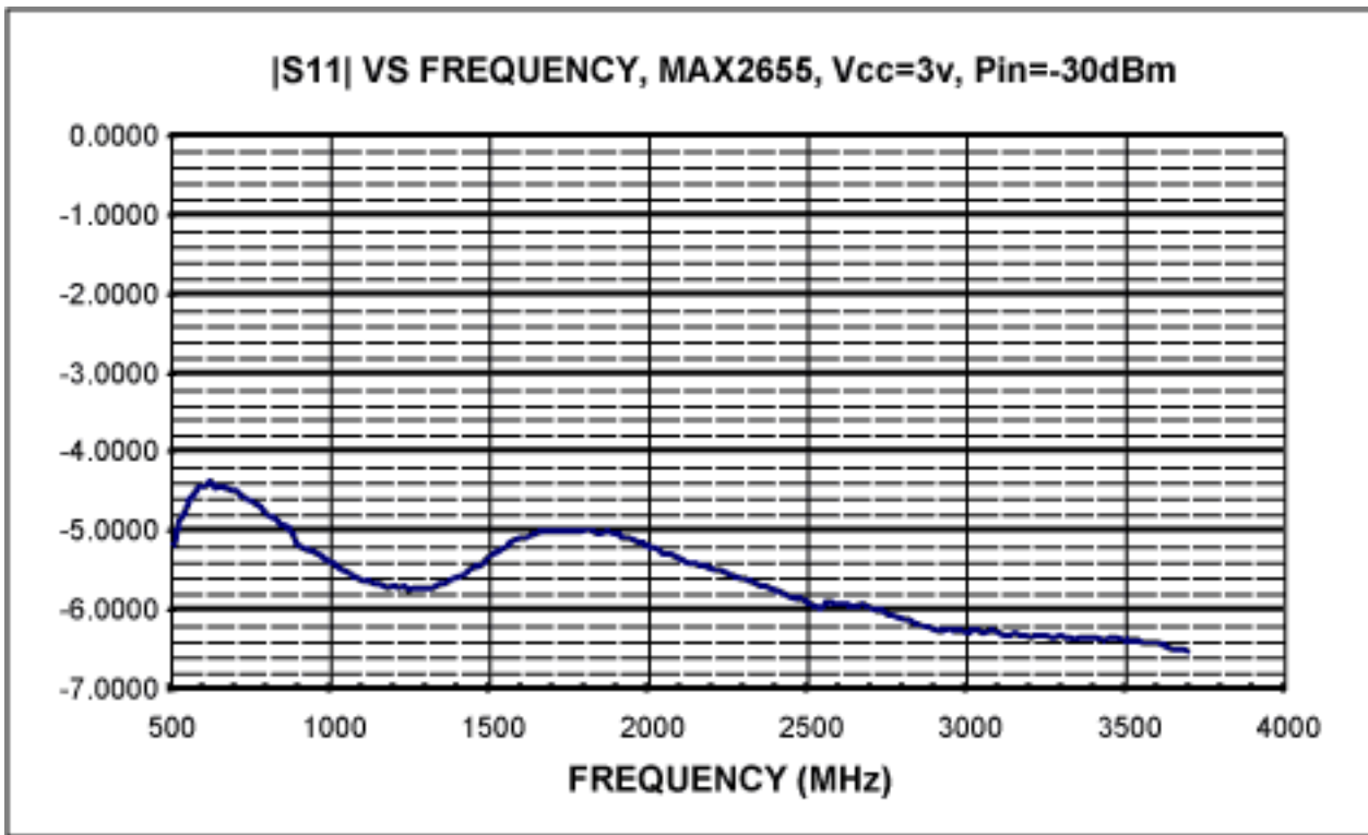
Figure 7. Input return loss vs. frequency.
