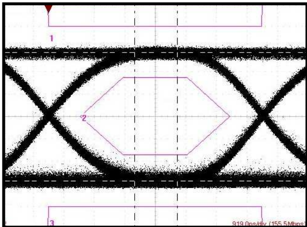
Figure 5. Optical eye – OC3, 2^{23}-1 PRBS, C_{APC} = 0.01\mu F
