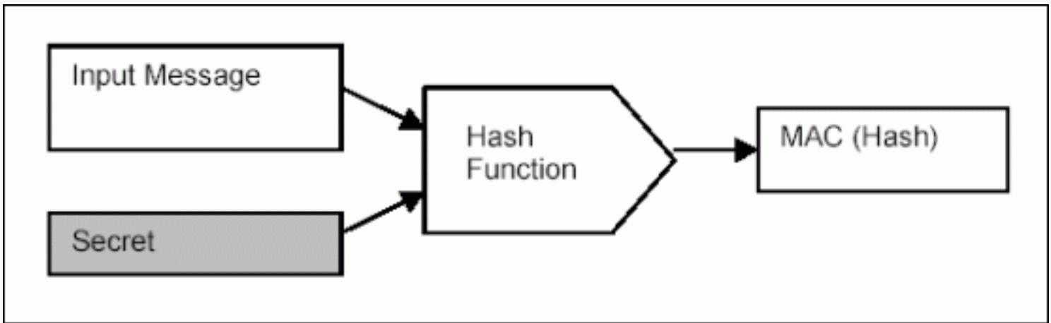
Figure 1. MAC generation.
