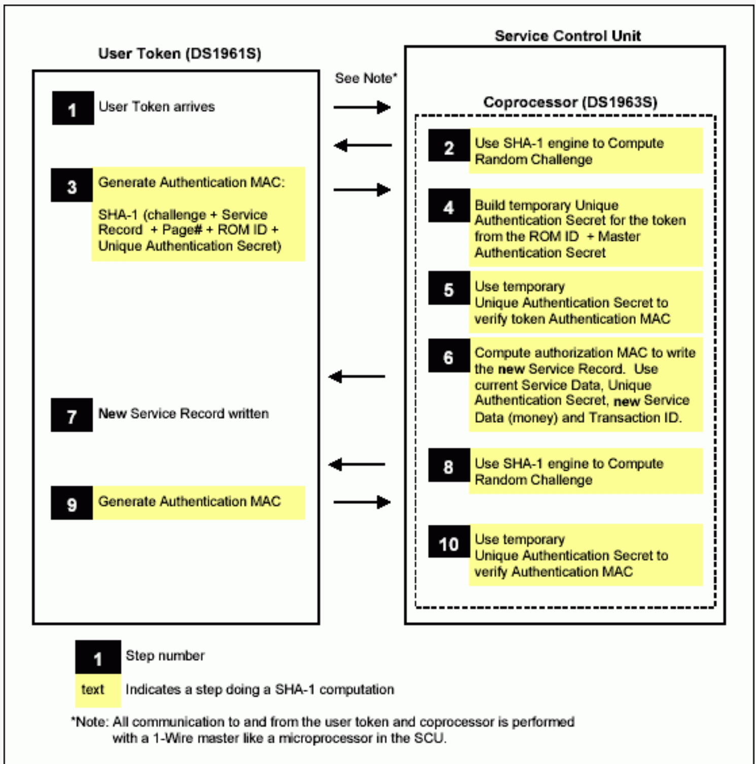
Figure 7. DS1961S typical transaction flow.
