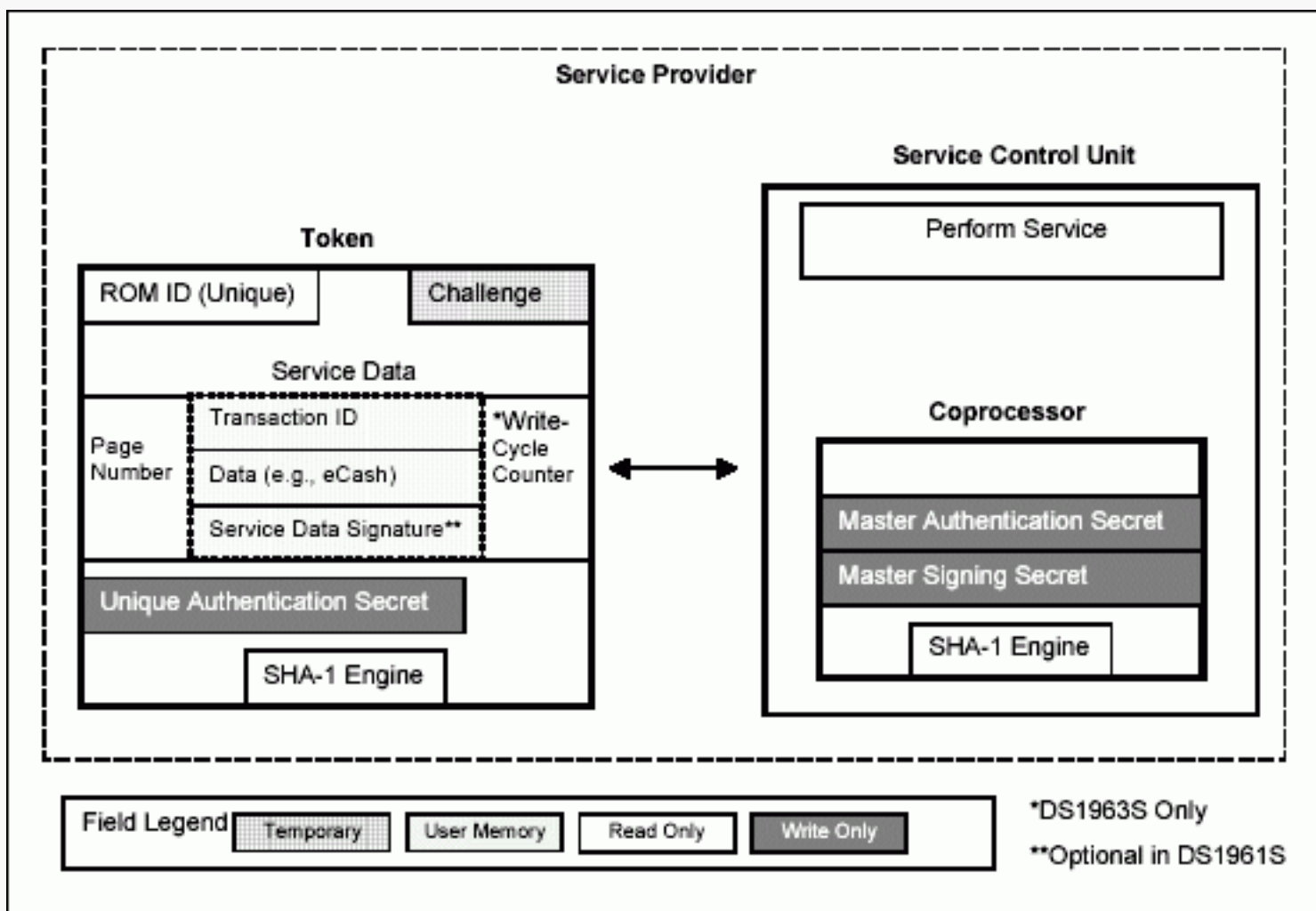
Figure 3. Service.
