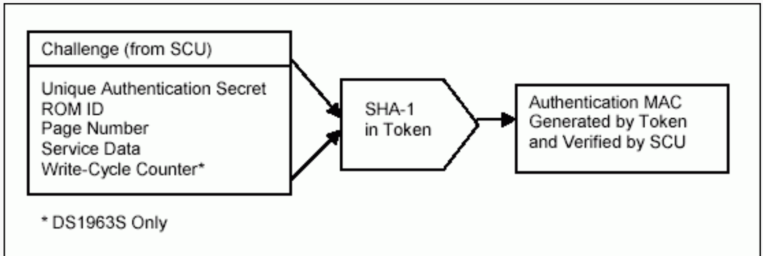
Figure 4. Token authentication.
