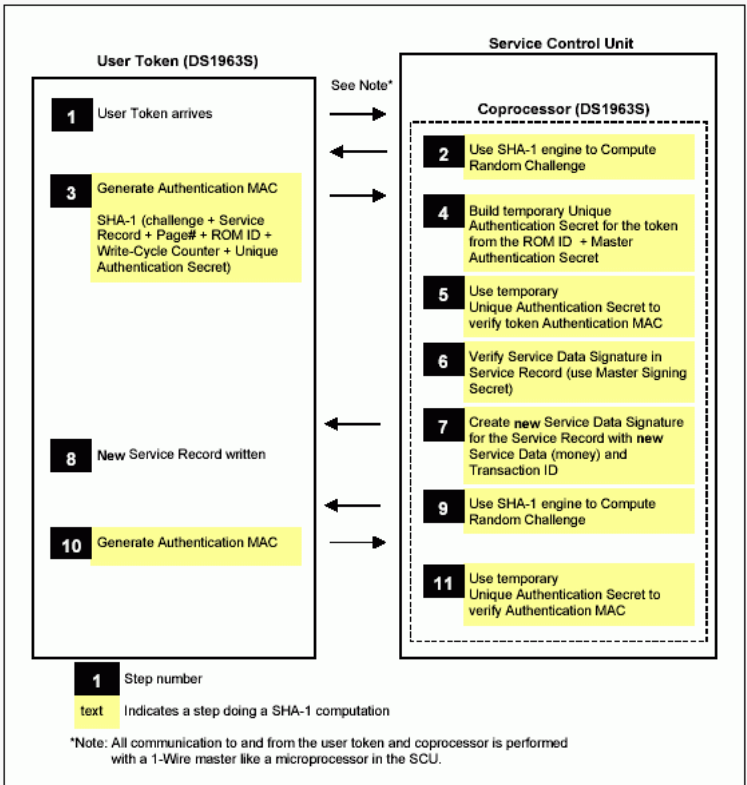
Figure 6. DS1963S typical transaction flow.
