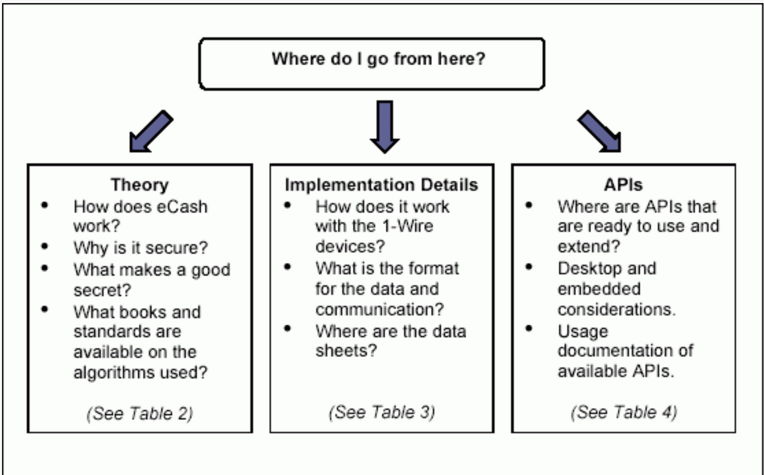
Figure 8. Resource overview.
