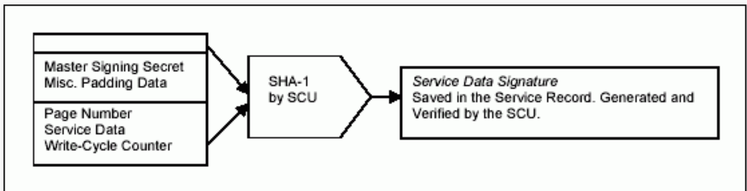
Figure 5. DS1963S service data validation.
