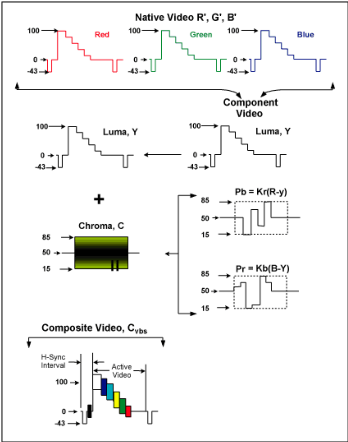
Figure 2. Analog encoding from R'G'B' to C_{vbs} .
