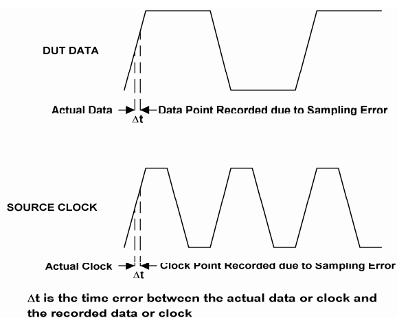
Figure 2. Error Caused by Non-Ideal Sampling
