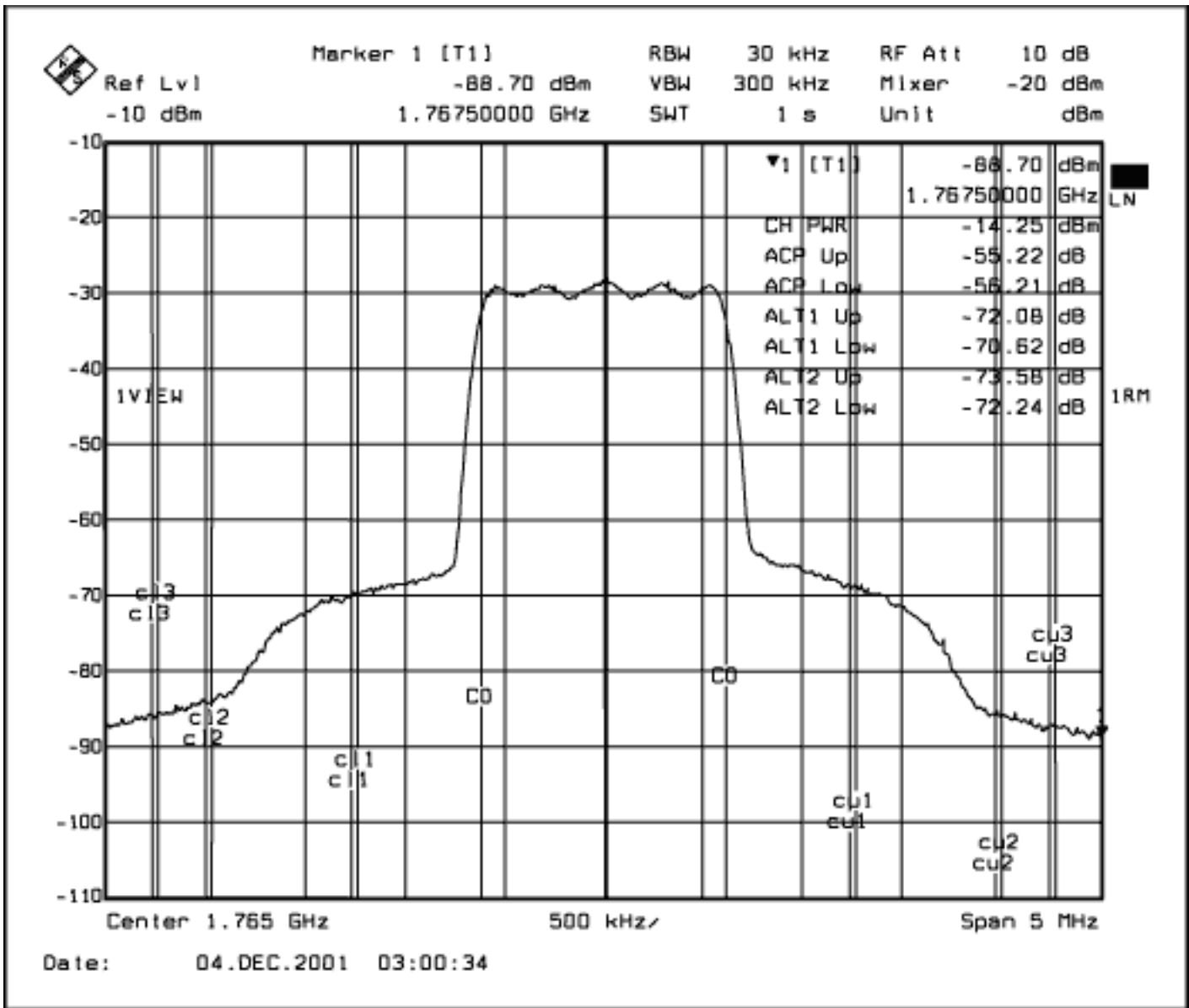
Figure 5. The MAX2361 driver output at +10dBm (measured at RFHO).
