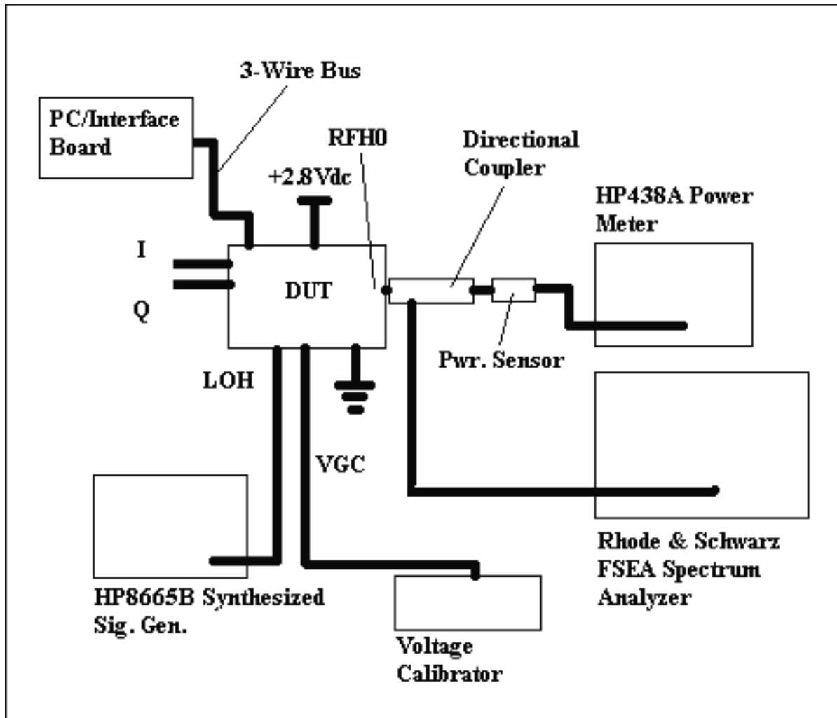
Figure 1. Test setup diagram.
