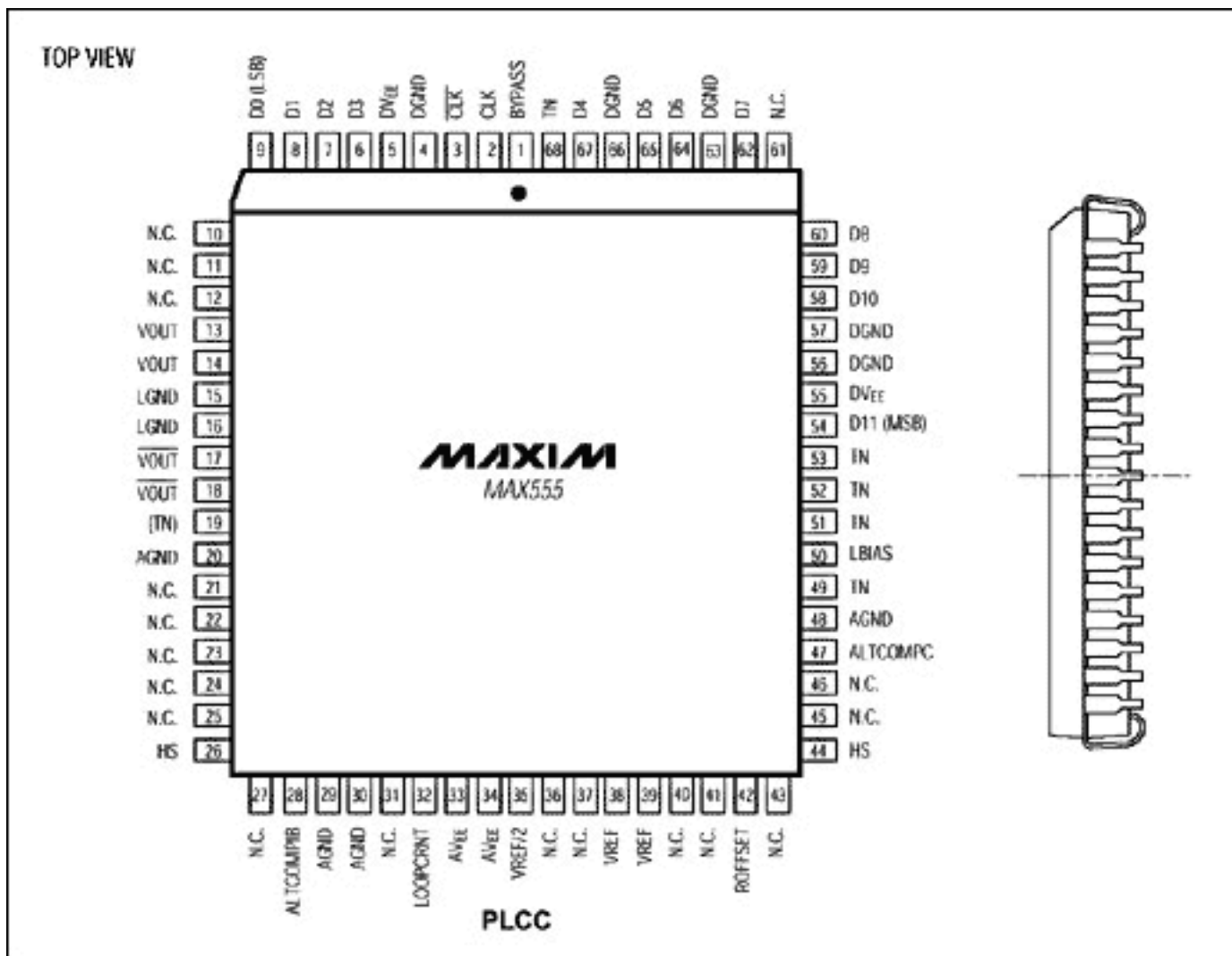
Figure 1a. Old 68-pin PLCC pinout.
