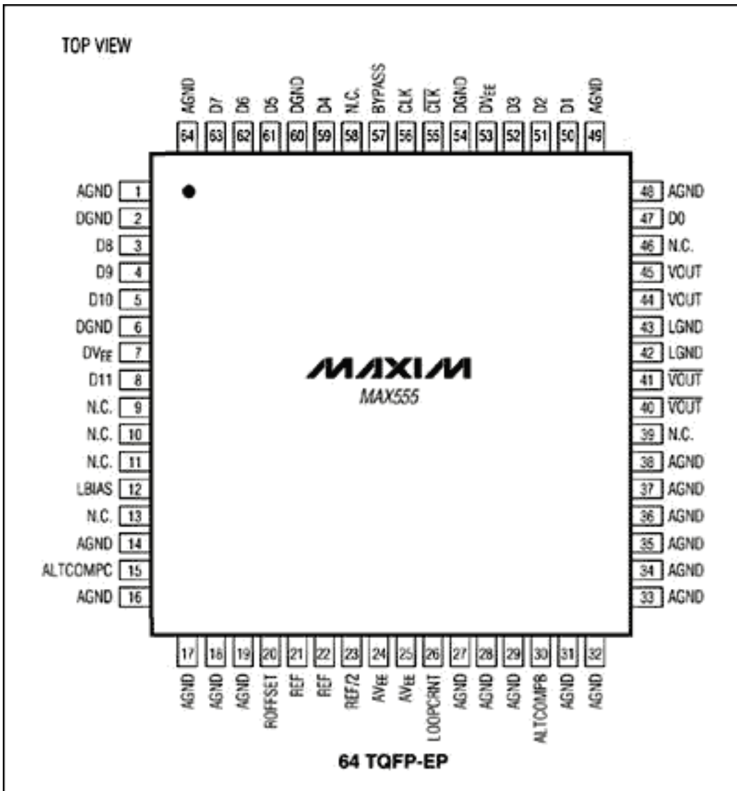
Figure 1b. New 64-pin TQFP pinout.
