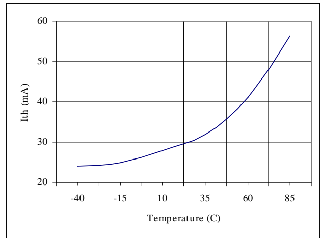
Figure 2. Laser threshold change over temperature
