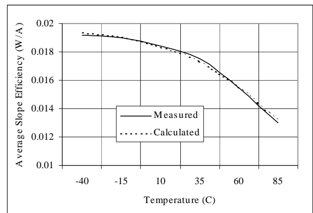
Figure 3. Laser average slope efficiency change over temperature ( P_{AVG} = -4dBm ): from measurement and from calculation
