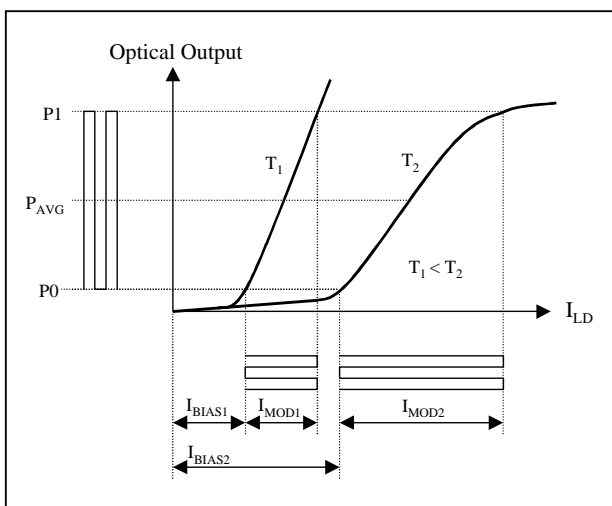
Figure 1. Laser behavior changes over temperature
