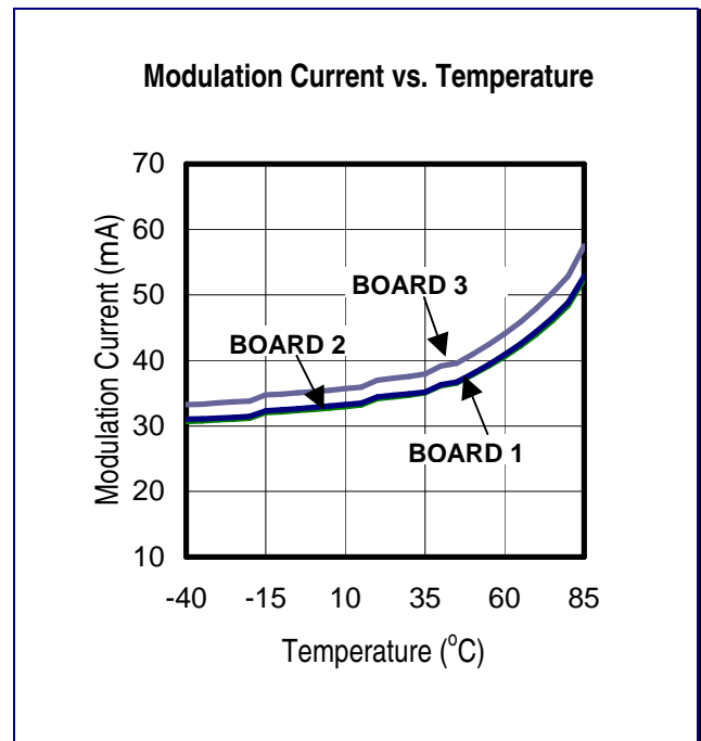
Figure 10: Modulation Current vs. Temperature
