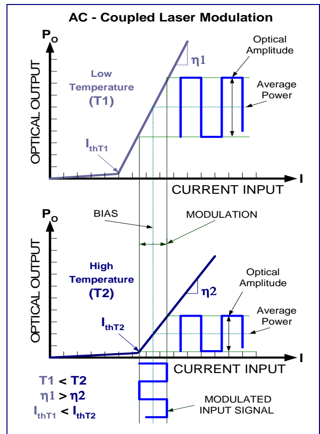
Figure 1. Optical Output vs. Laser Current
