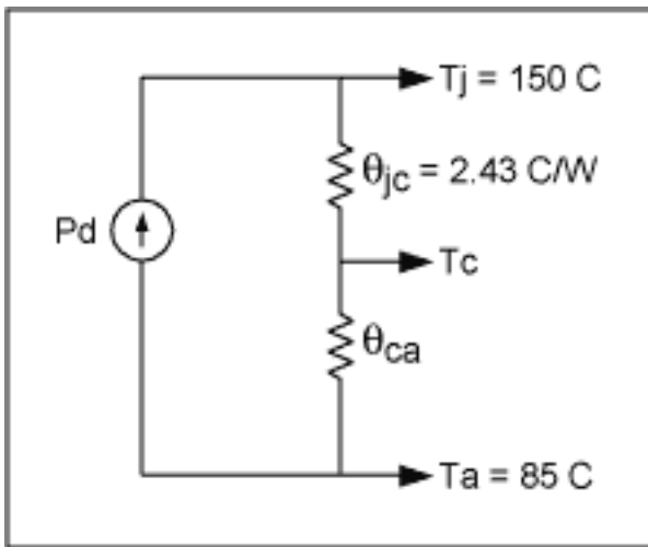
Figure 2. Power dissipation.
