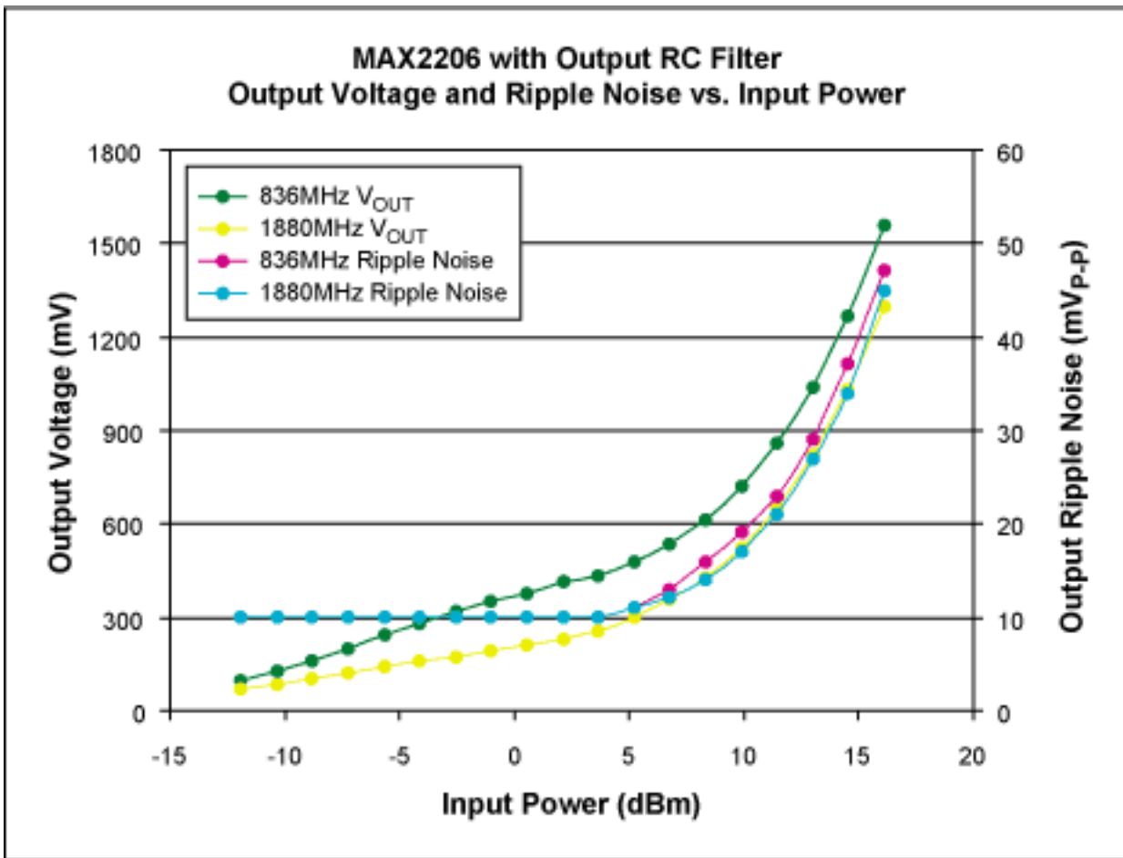
Figure 2. The MAX2206 performance data.
