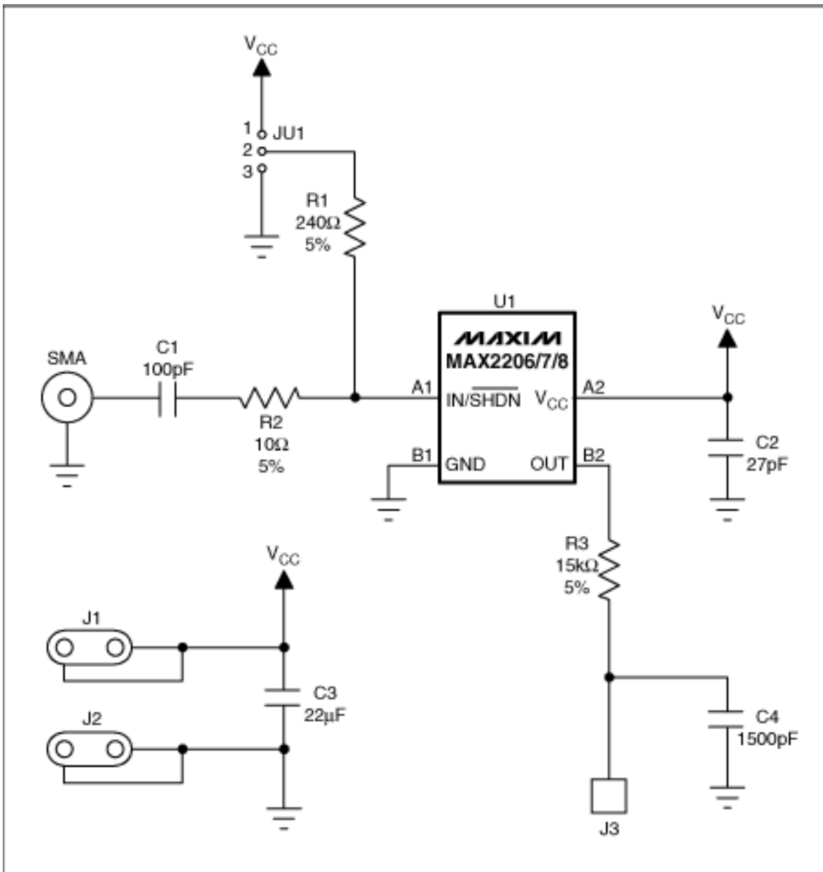
Figure 4. The MAX2206 evaluation kit schematic.
