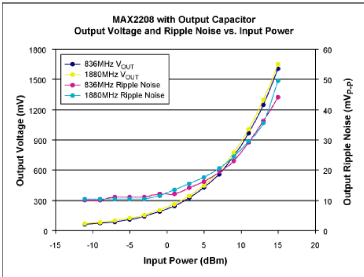
Figure 1. The MAX2208 performance data.
