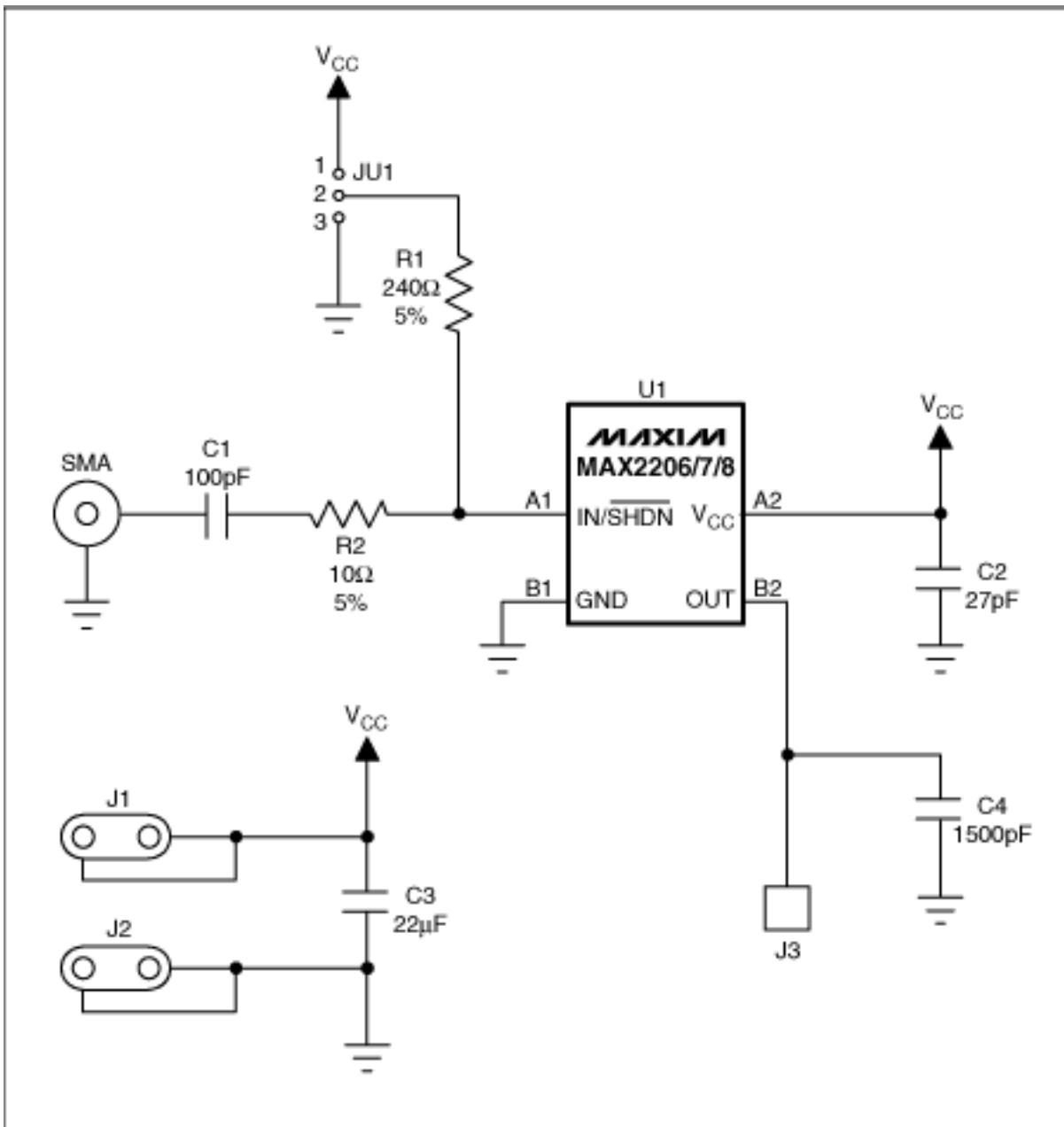
Figure 3. The MAX2208 evaluation kit schematic.
