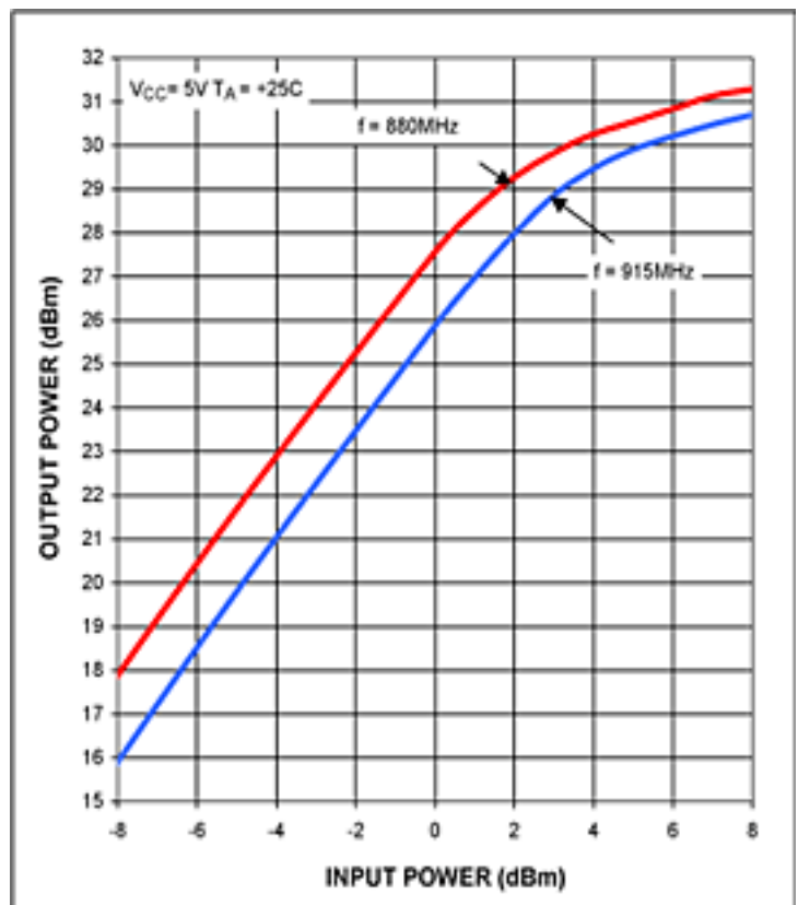
Figure 2. The MAX2235 output power vs input power.
