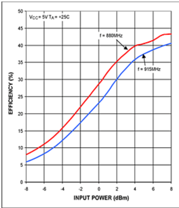
Figure 3. The MAX2235 efficiency vs input power.
