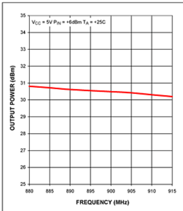
Figure 1. The MAX2235 output power vs frequency.
