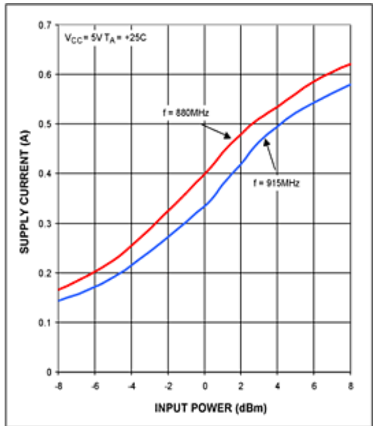
Figure 4. The MAX2235 supply current vs input power.
