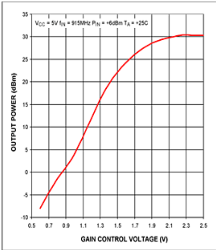
Figure 5. The MAX2235 output power vs GC voltage.
