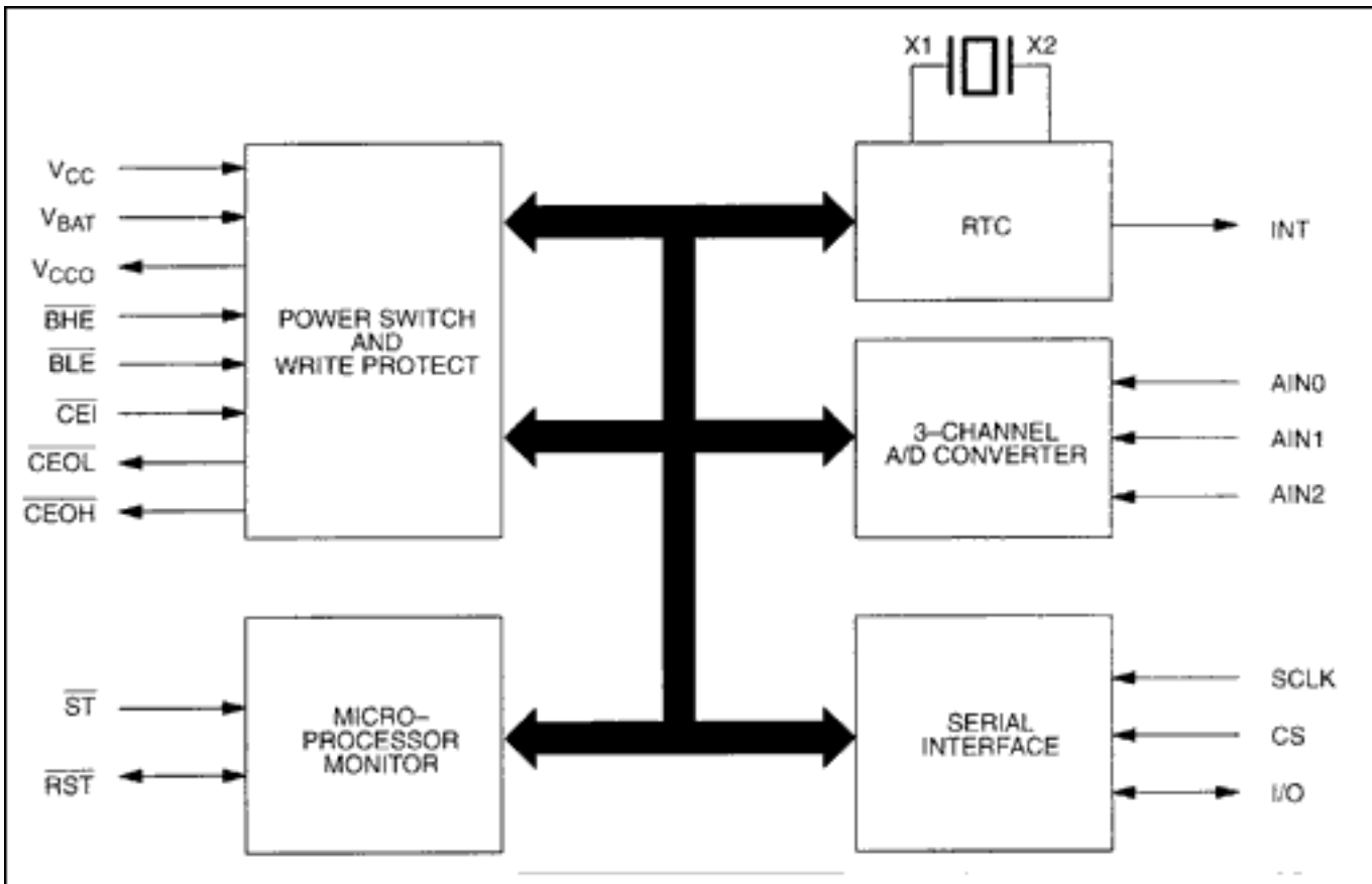
Figure 1. DS1670 block diagram.
