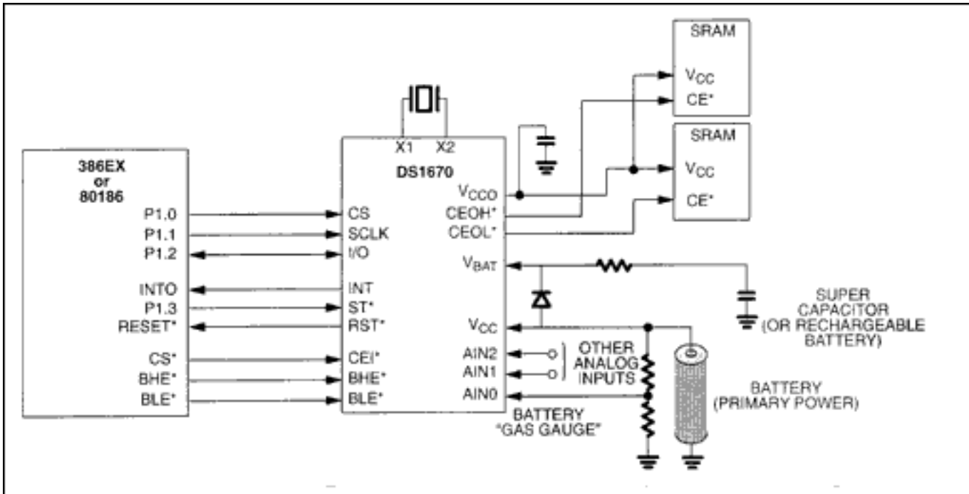
Figure 2. Typical application.
