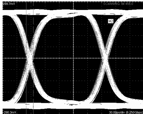
6.25Gbps MAX3785 Equalizer Output
