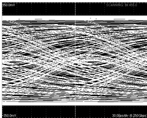
6.25Gbps Unequalized Signal after 30in FR4
